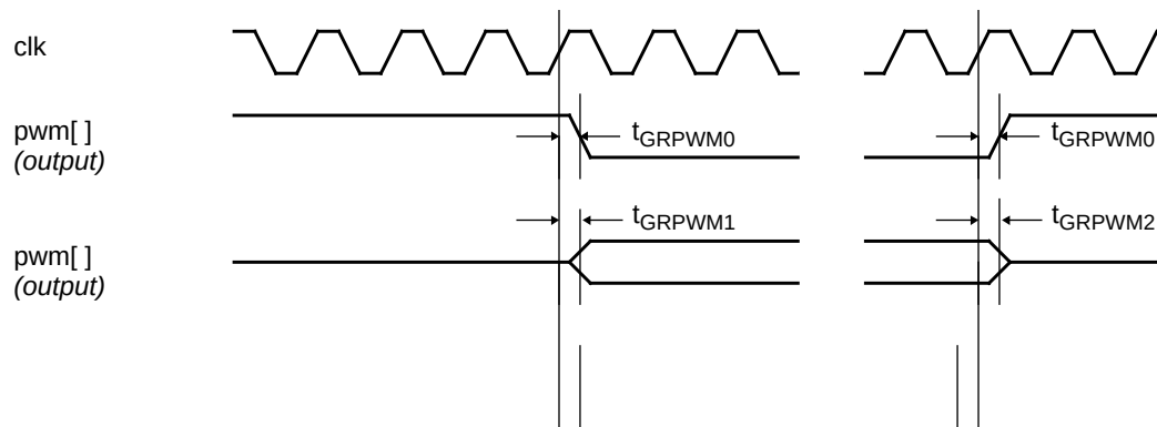
Figure 158. Timing waveforms
