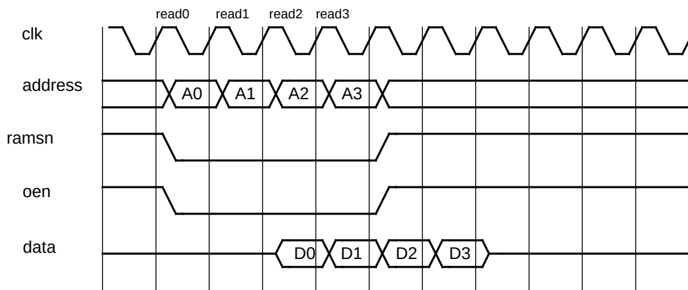
Figure 278. 32-bit SSRAM read cycle
