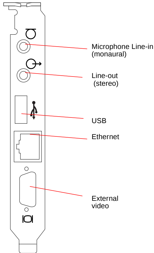
FIGURE 10-1 SunPCi II Card Backplate Connectors
