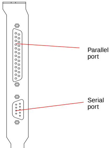
FIGURE 10-2 SunPCi II Card Add-On Backplate Connectors
