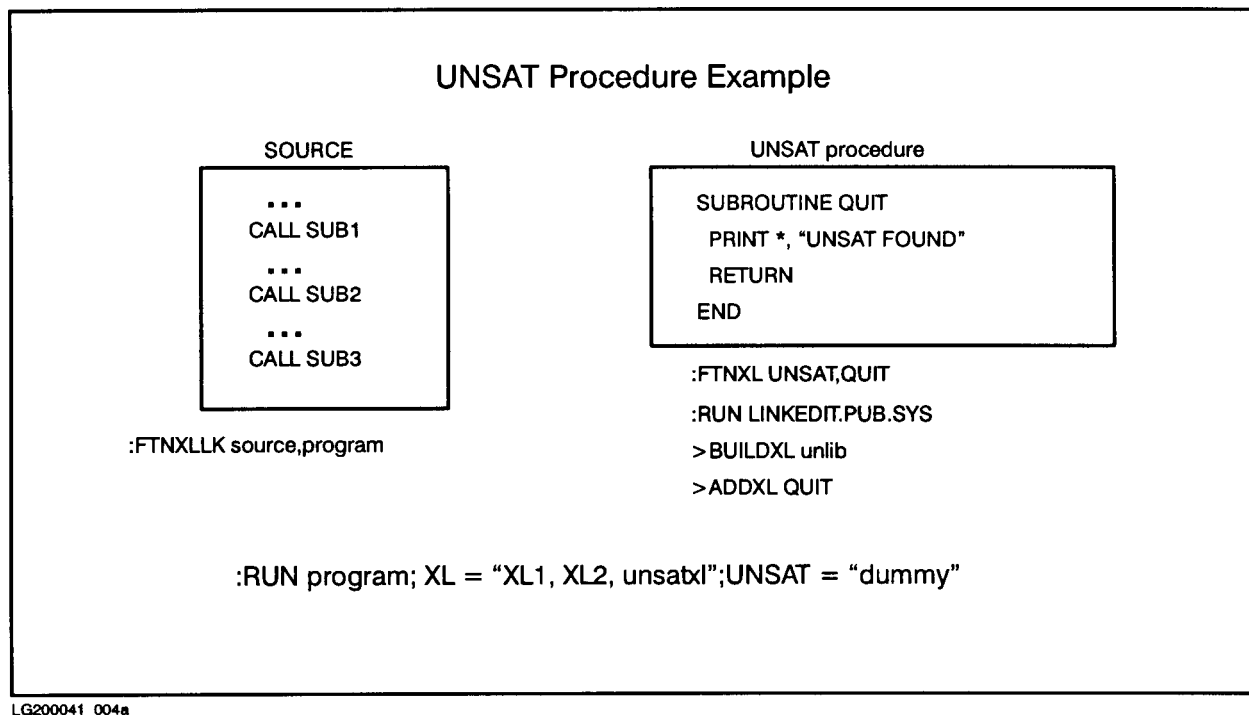
Figure 3-4. UNSAT Procedure Example
