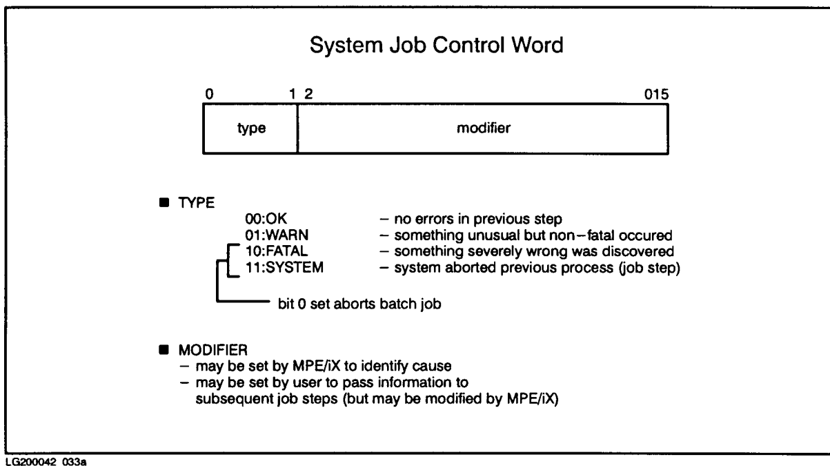
Figure 3-5. Job Control Word (JCW) Structure
