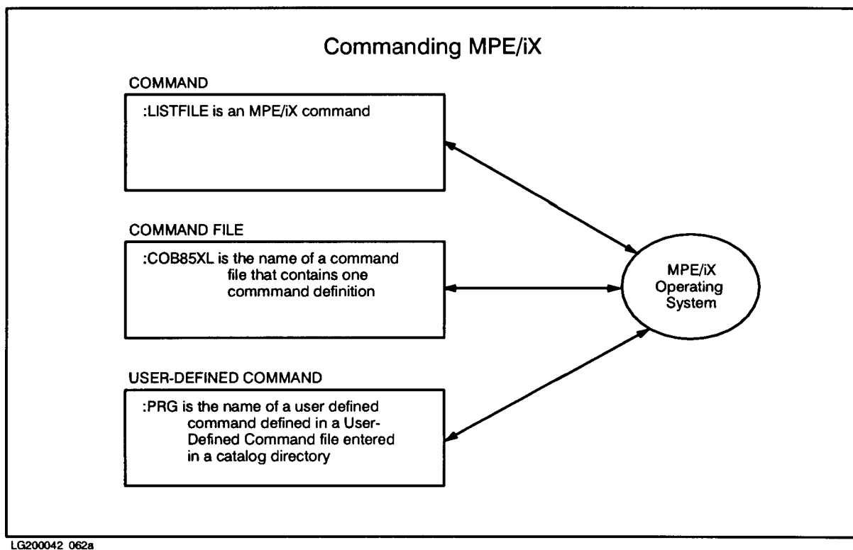
Figure 1-4. Commanding MPE/iX
