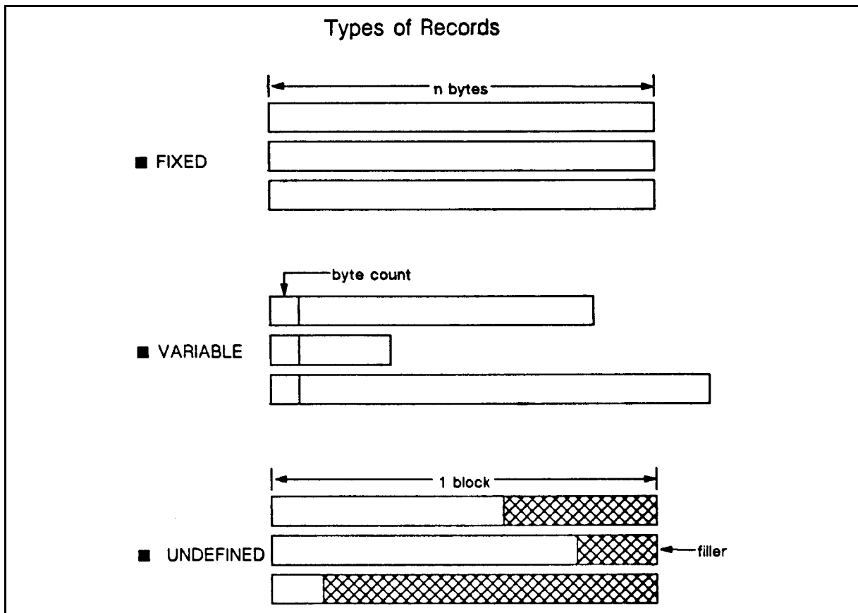
Figure 6-12. Record Types
