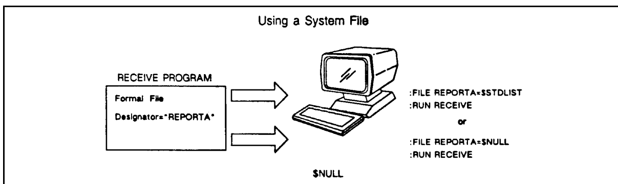
Figure 6-7. Using a System File
