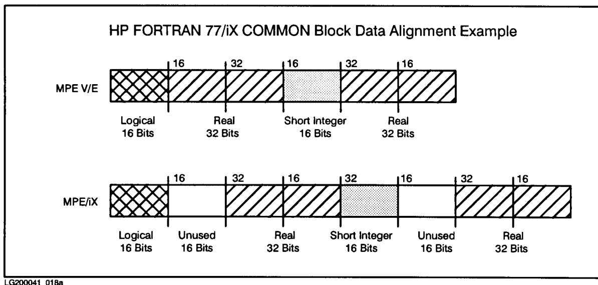
Figure 1-11. HP FORTRAN 77/iX COMMON Block Data Alignment Example
