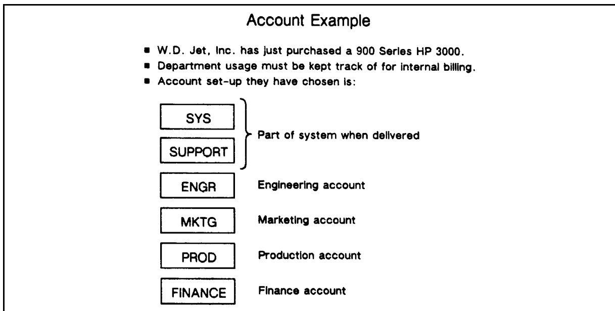
Figure 1-6. Accounts Example
