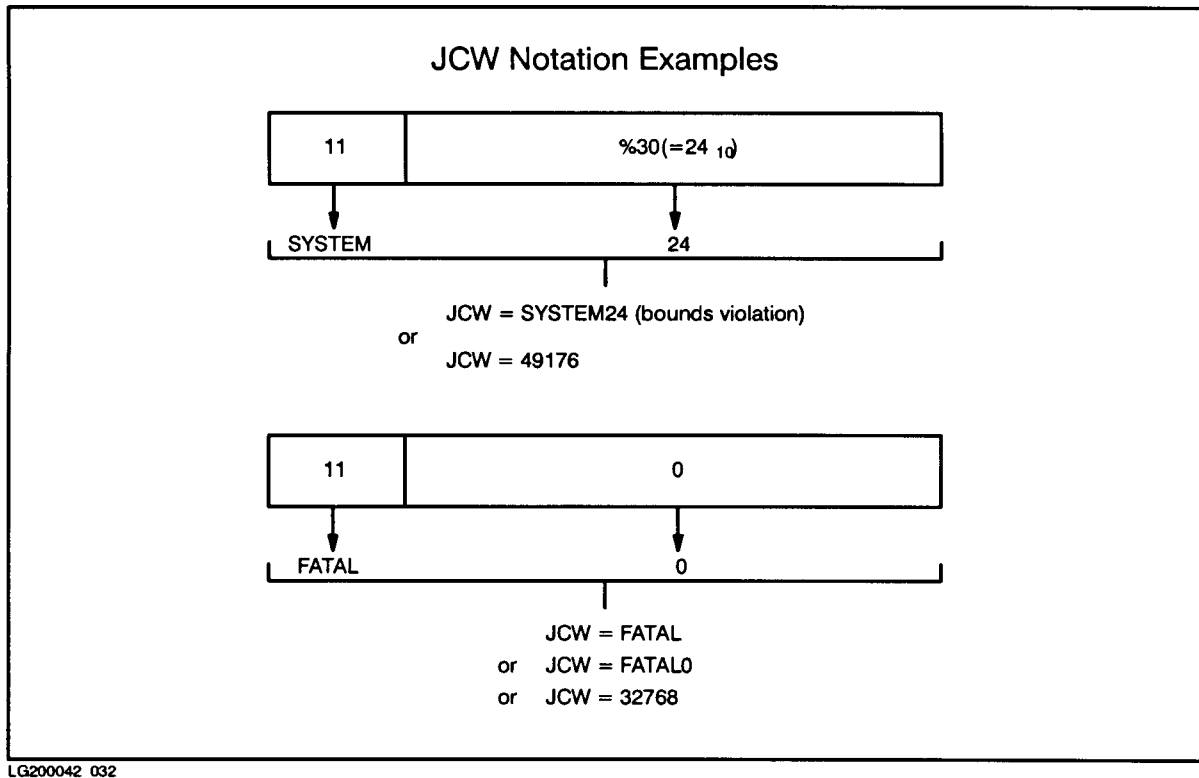
Figure 3-6. JCW Notation Examples
