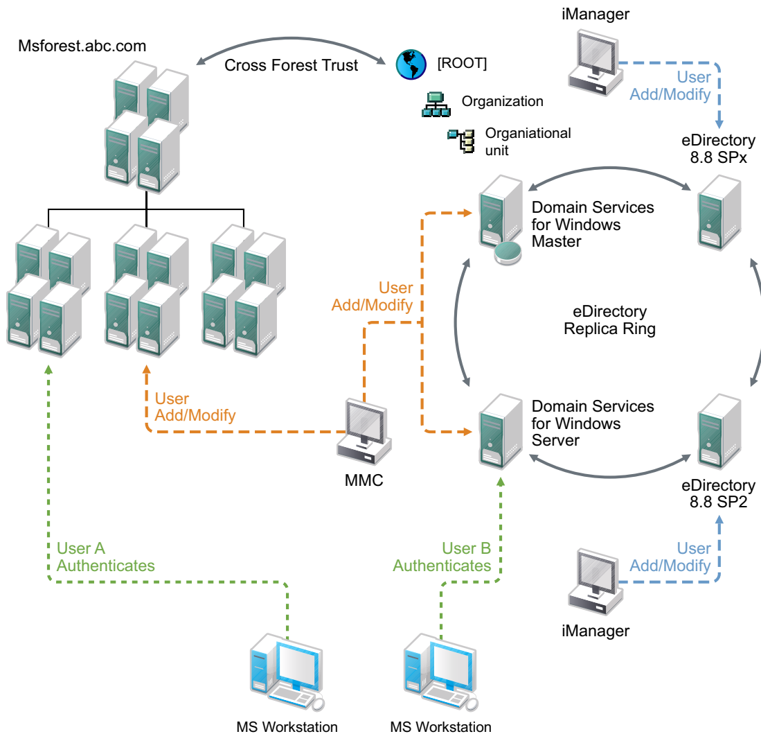
Figure 3-4 Cross-Forest Trust between Active Directory and DSfW
