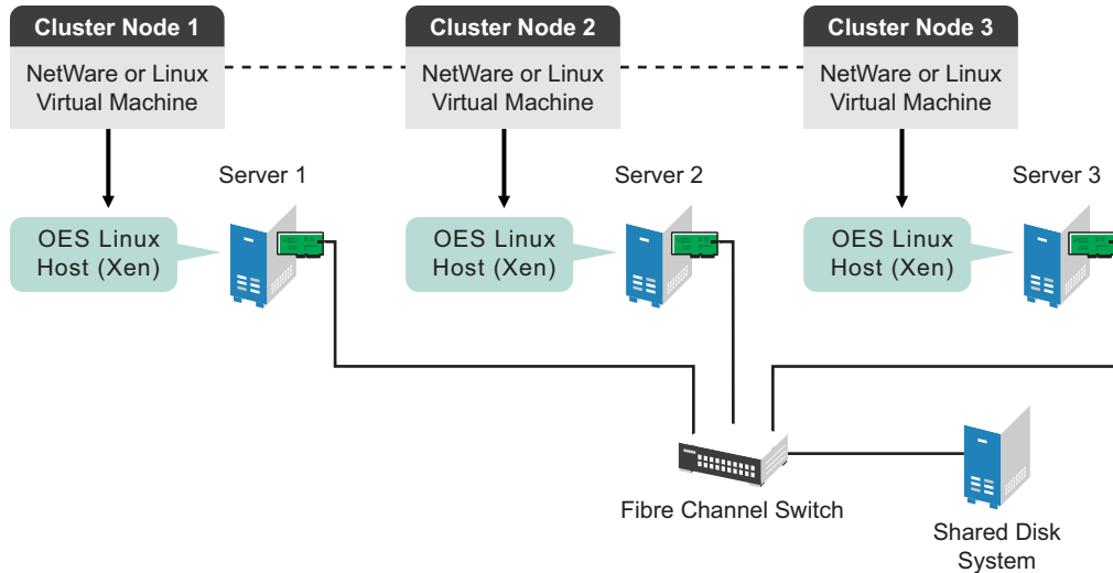
Figure 12-2 Virtual Machines as Cluster Nodes
