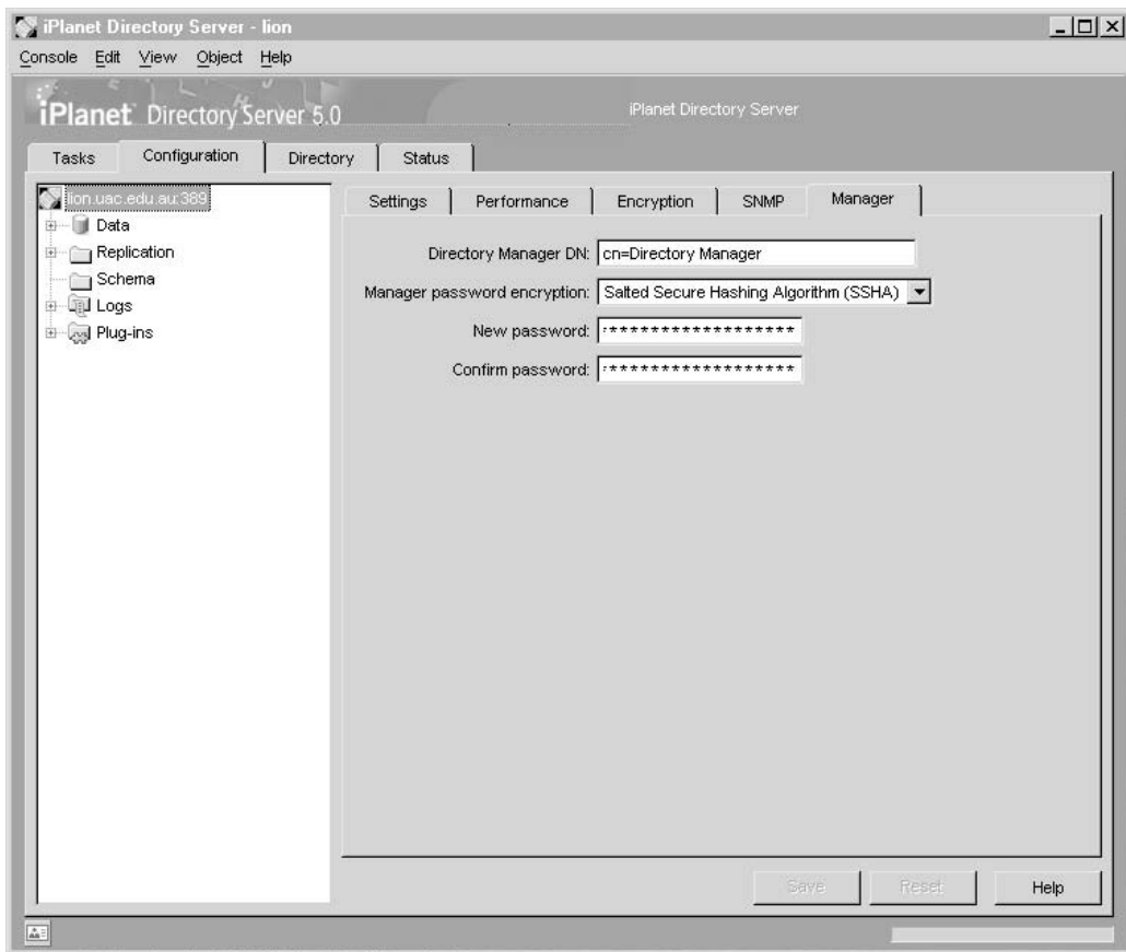
FIGURE 30-9 Manager configuration window
