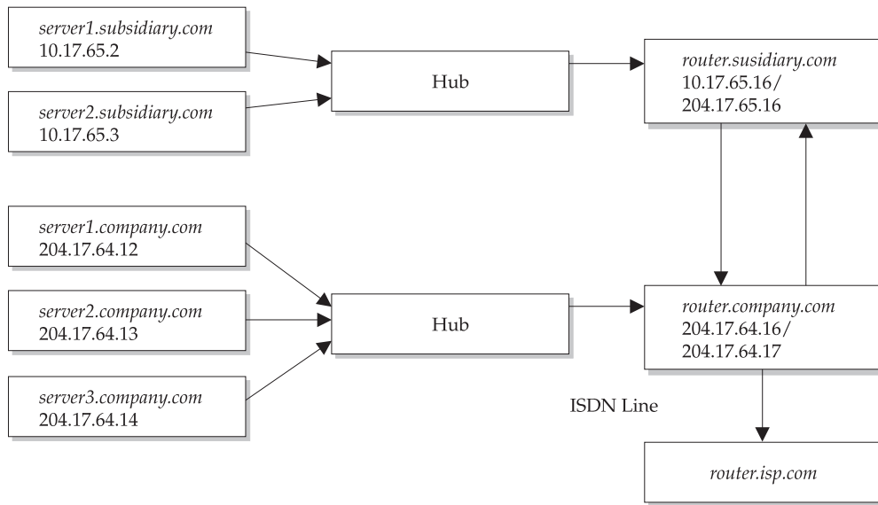
FIGURE 23-2 Connecting two class C networks (204.17.64.0 and 204.17.65.0)
