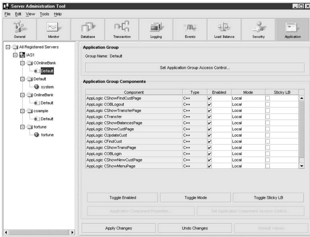
FIGURE 33-29 Application group configuration
