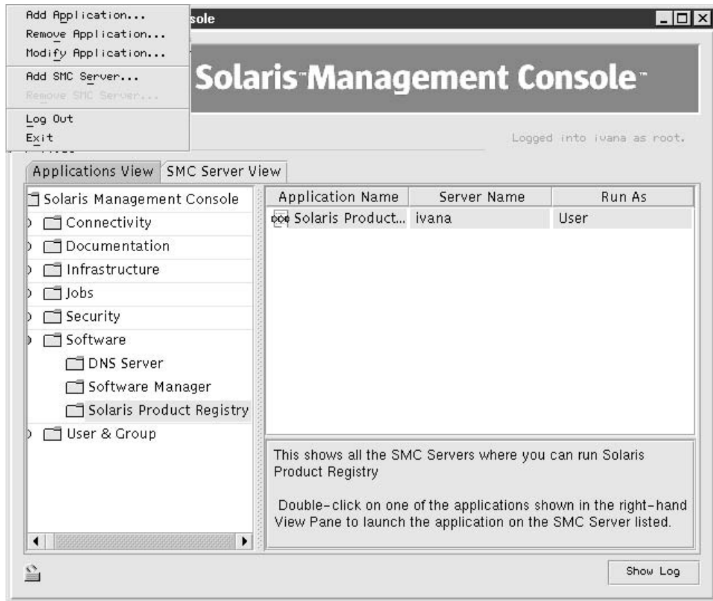
FIGURE 12-11 SMC Console menu
