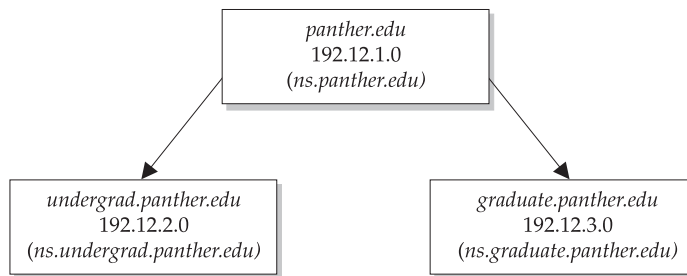
FIGURE 29-1 DNS configuration for a fictional college with two divisions—graduate and undergraduate—both of which have their own name server
