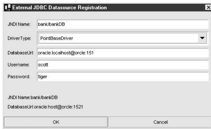
FIGURE 33-14 Data source configuration
