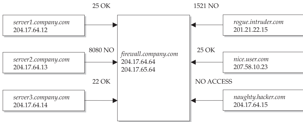
FIGURE 23-4 Basic firewall configuration blocking incoming and outgoing ports
