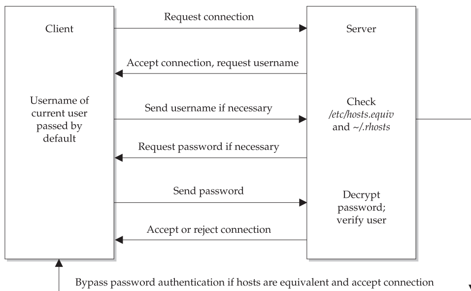
FIGURE 9-3 Identification and authentication sequence for rlogin
