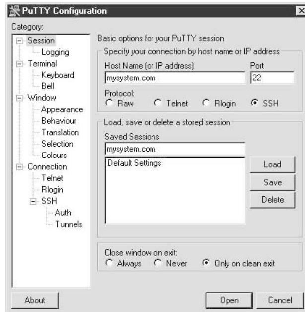
FIGURE 9-4 Typical SSH client session
