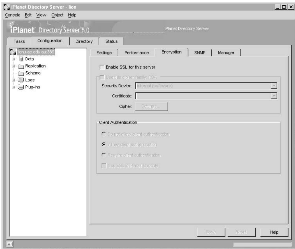
FIGURE 30-7 Encryption configuration window
