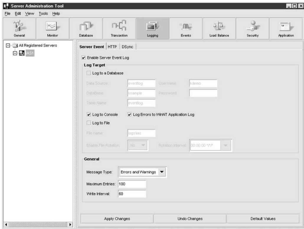
FIGURE 33-21 Server event configuration
