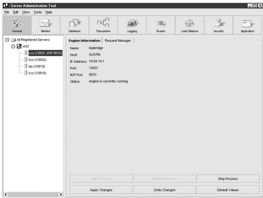
FIGURE 33-8 Application server engine configuration
