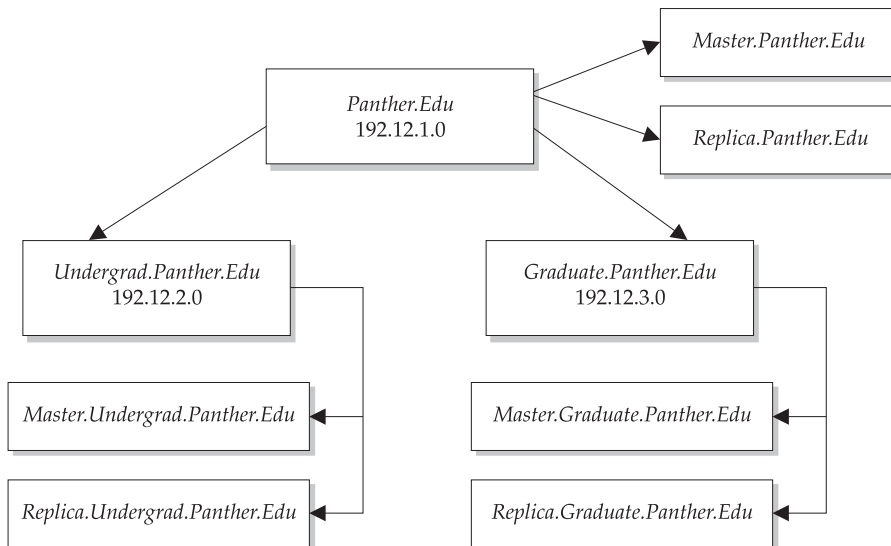
FIGURE 29-3 NIS+ domains with a master and a slave server each
