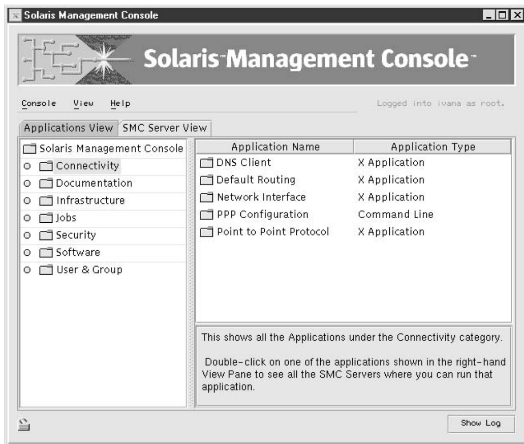
FIGURE 12-3 SMC Applications View
