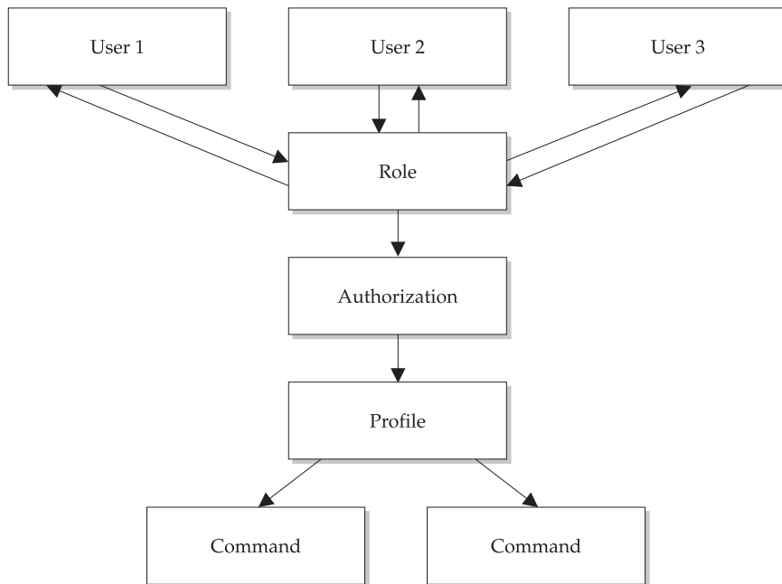
FIGURE 11-2 Profiles and authorizations are associated with roles that are granted to individual users.
