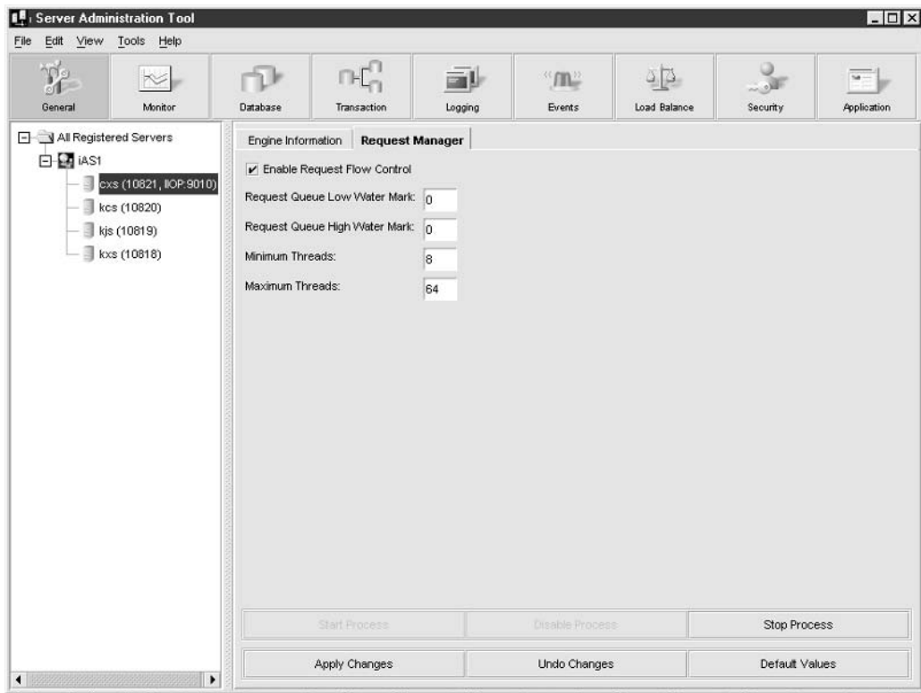
FIGURE 33-9 Request Manager configuration
