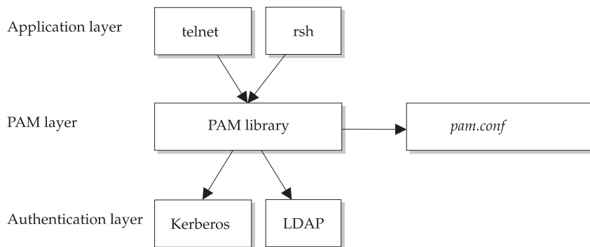
FIGURE 13-2 PAM stack structure for flexible authentication
