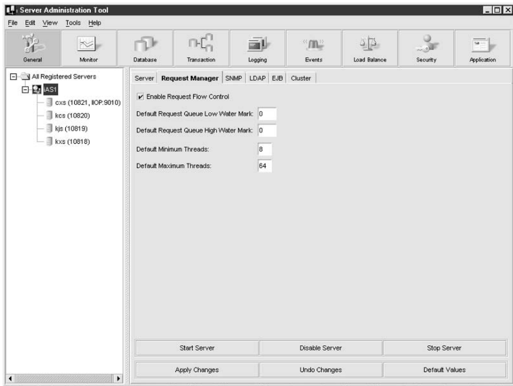
FIGURE 33-3 Request Manager tab
