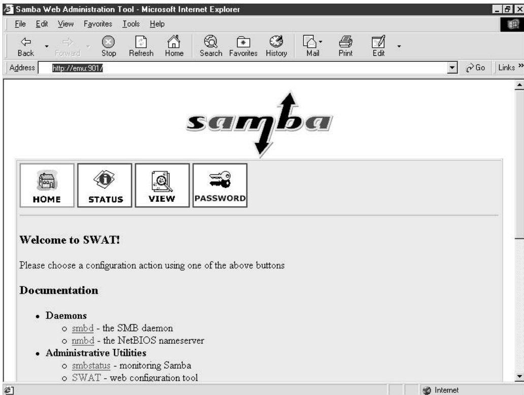
FIGURE 31-3 SWAT GUI for Samba
