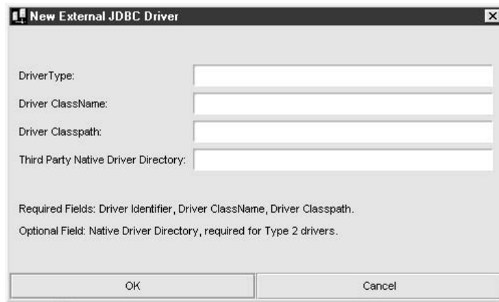
FIGURE 33-15 JDBC driver selection
