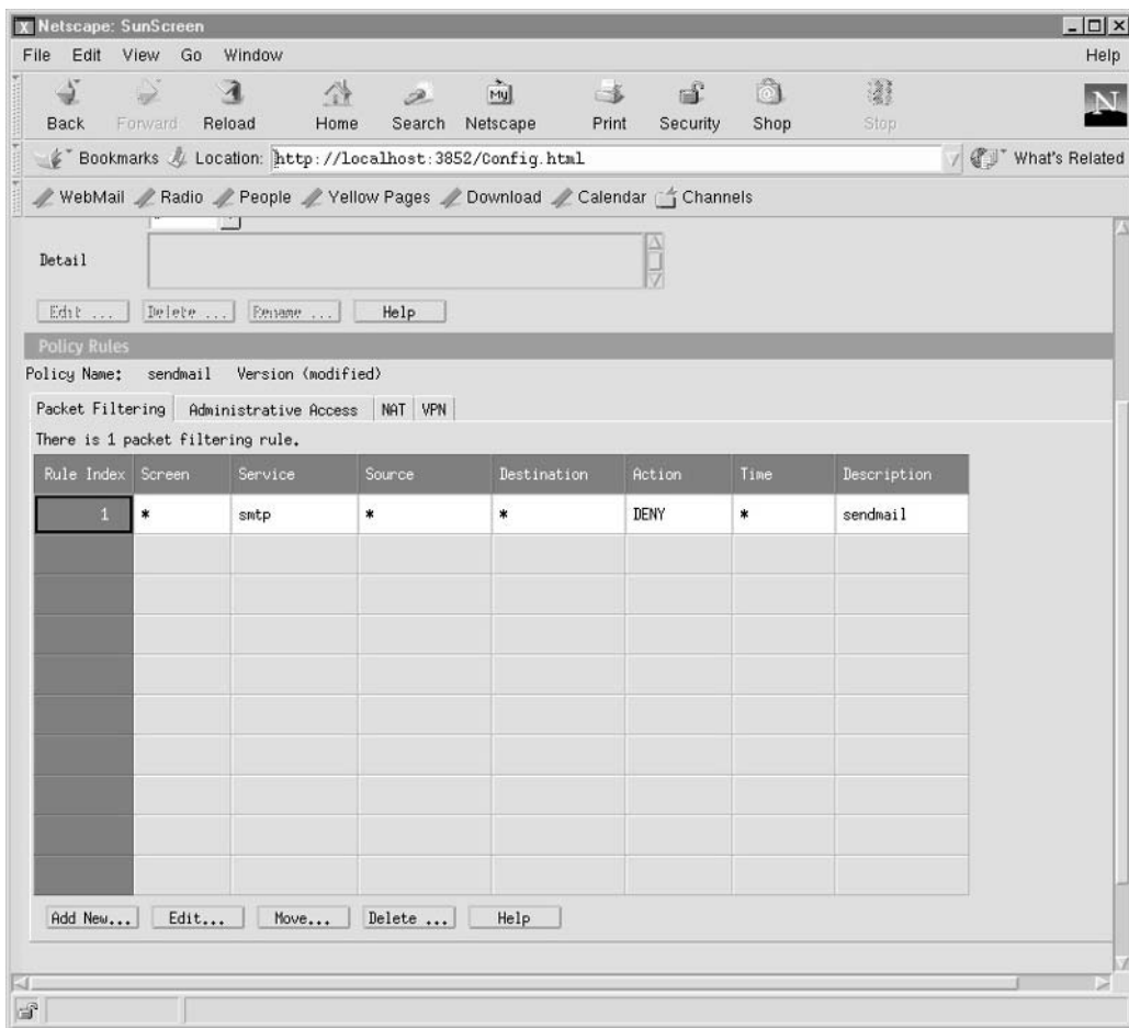
FIGURE 23-8 Policy Rules interface
