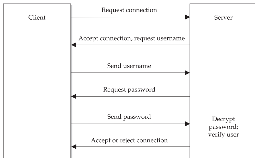
FIGURE 9-2 Identification and authentication of a Telnet session
