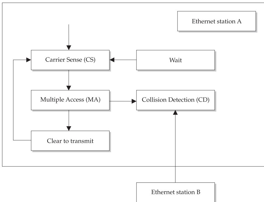
FIGURE 21-6 Process flow for CSMA/CD
