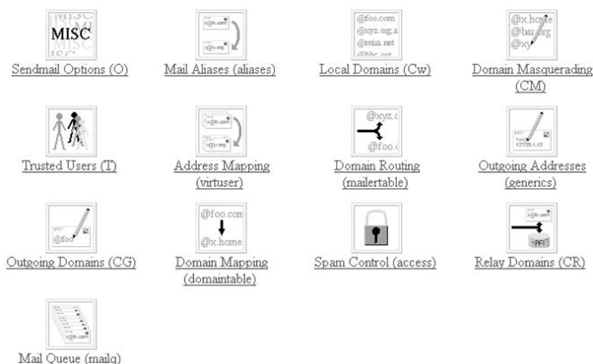
FIGURE 27-3 webmin GUI for configuring sendmail
