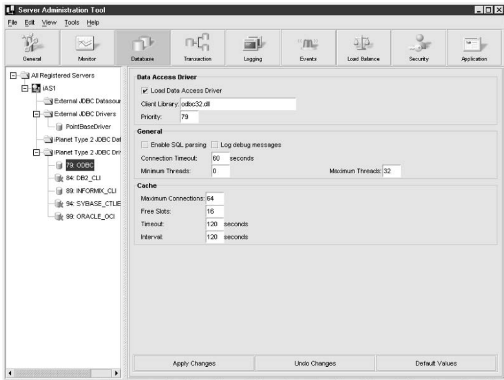
FIGURE 33-16 Selecting an existing JDBC configuration
