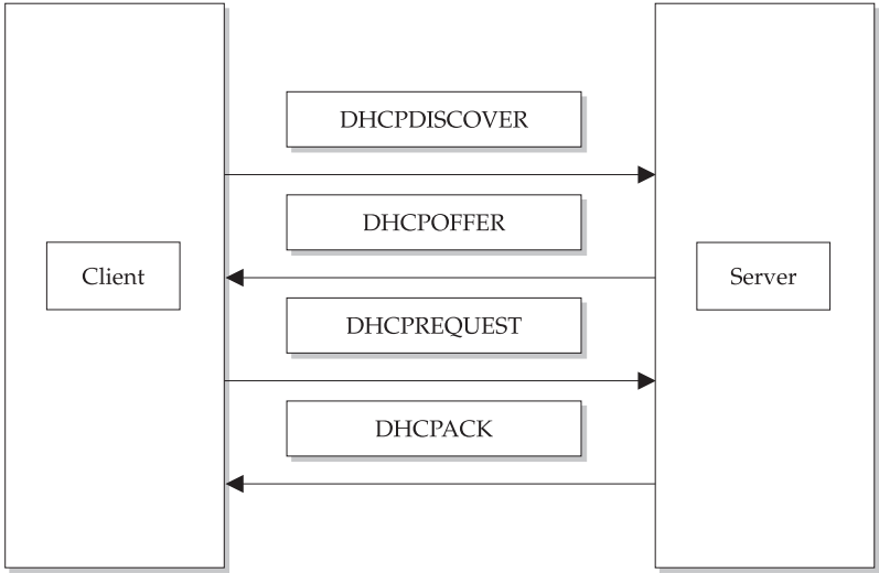
FIGURE 22-3 How DHCP leases IP addresses
