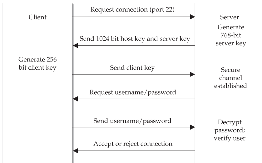
FIGURE 9-5 Authenticating an SSH connection
