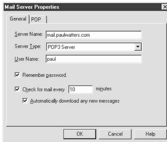
FIGURE 27-6 Configuring POP settings in the Netscape mail client
