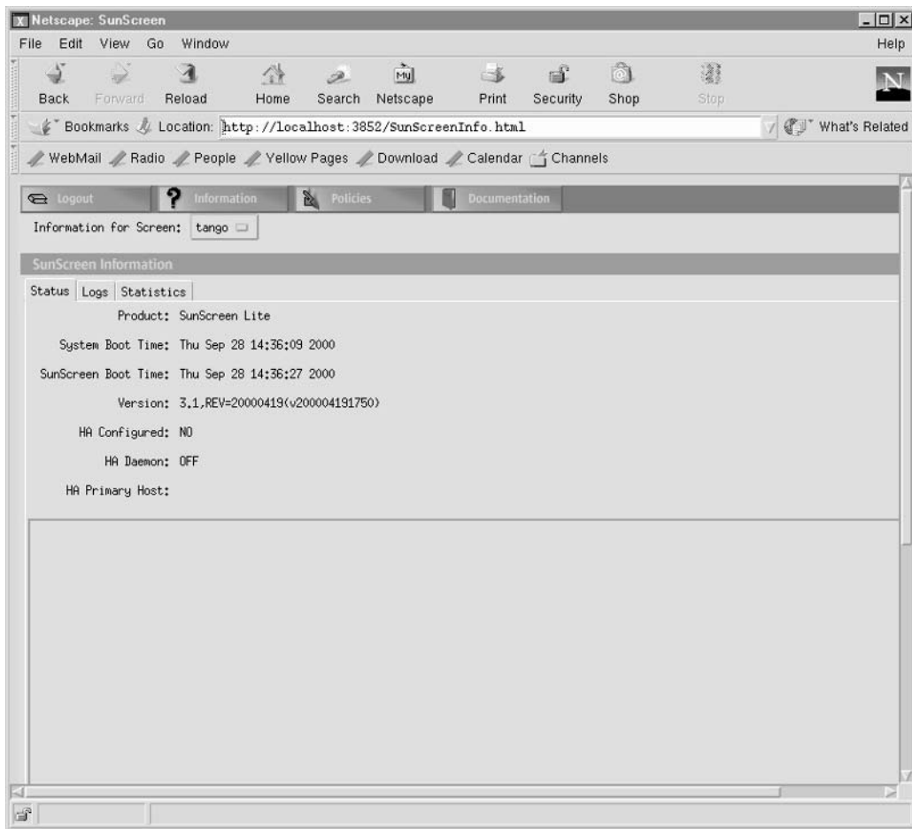
FIGURE 23-6 SunScreen Information interface
