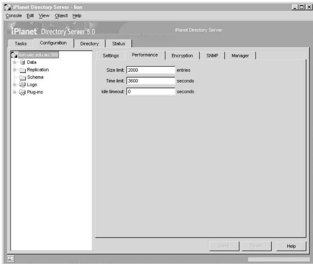
FIGURE 30-6 Performance configuration window
