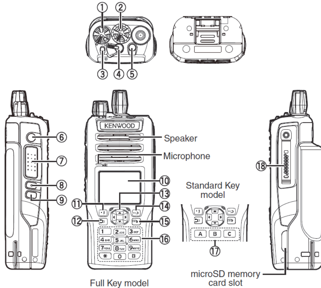
Figure 3.10 Locations of VP5000 Controls and Indicators
