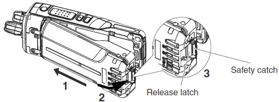
Figure 3.2 Removing VP5000 Battery Pack
