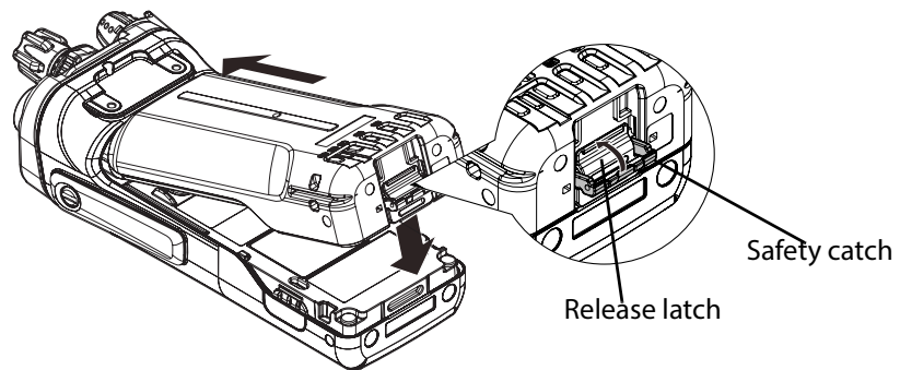
Figure 3.3 Removing VP6000 Battery Pack
