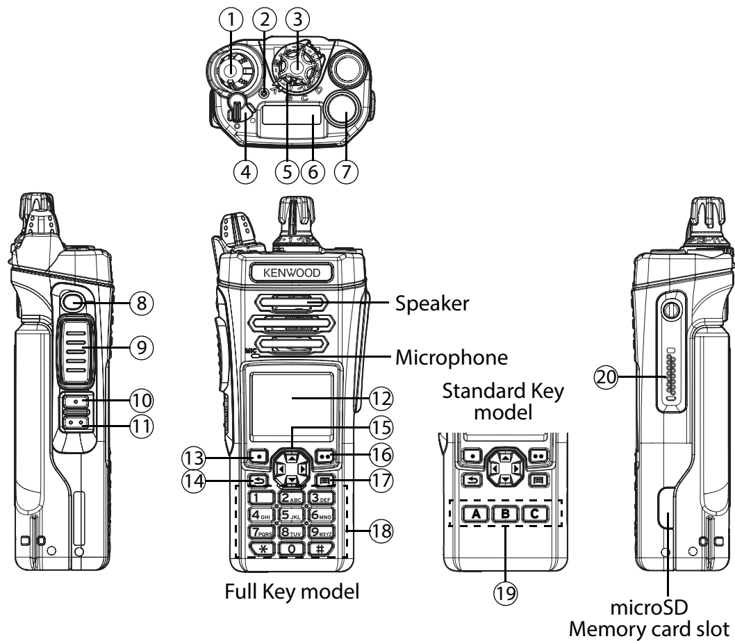
Figure 3.11 Locations of VP6000 Controls and Indicators
