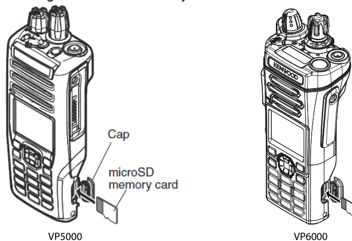
Figure 3.9 Installing the microSD Memory Card
