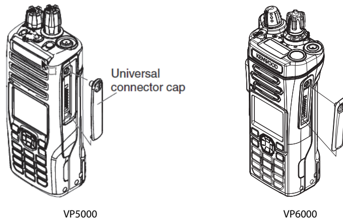
Figure 3.6 Installing Cap over Universal Connector
