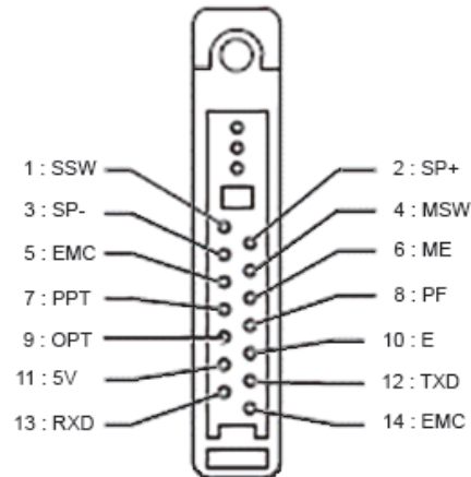
Figure 3.12 Universal Connector Terminal Pin Numbers
