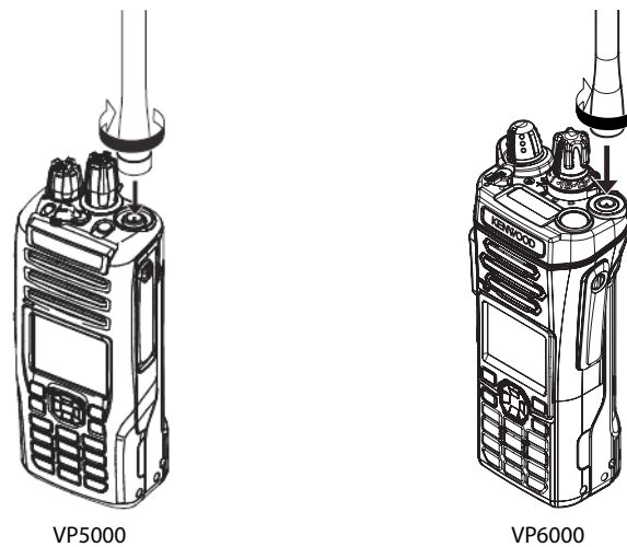
Figure 3.4 Installing the Antenna
