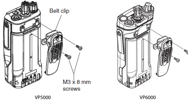
Figure 3.5 Installing Belt Clip
