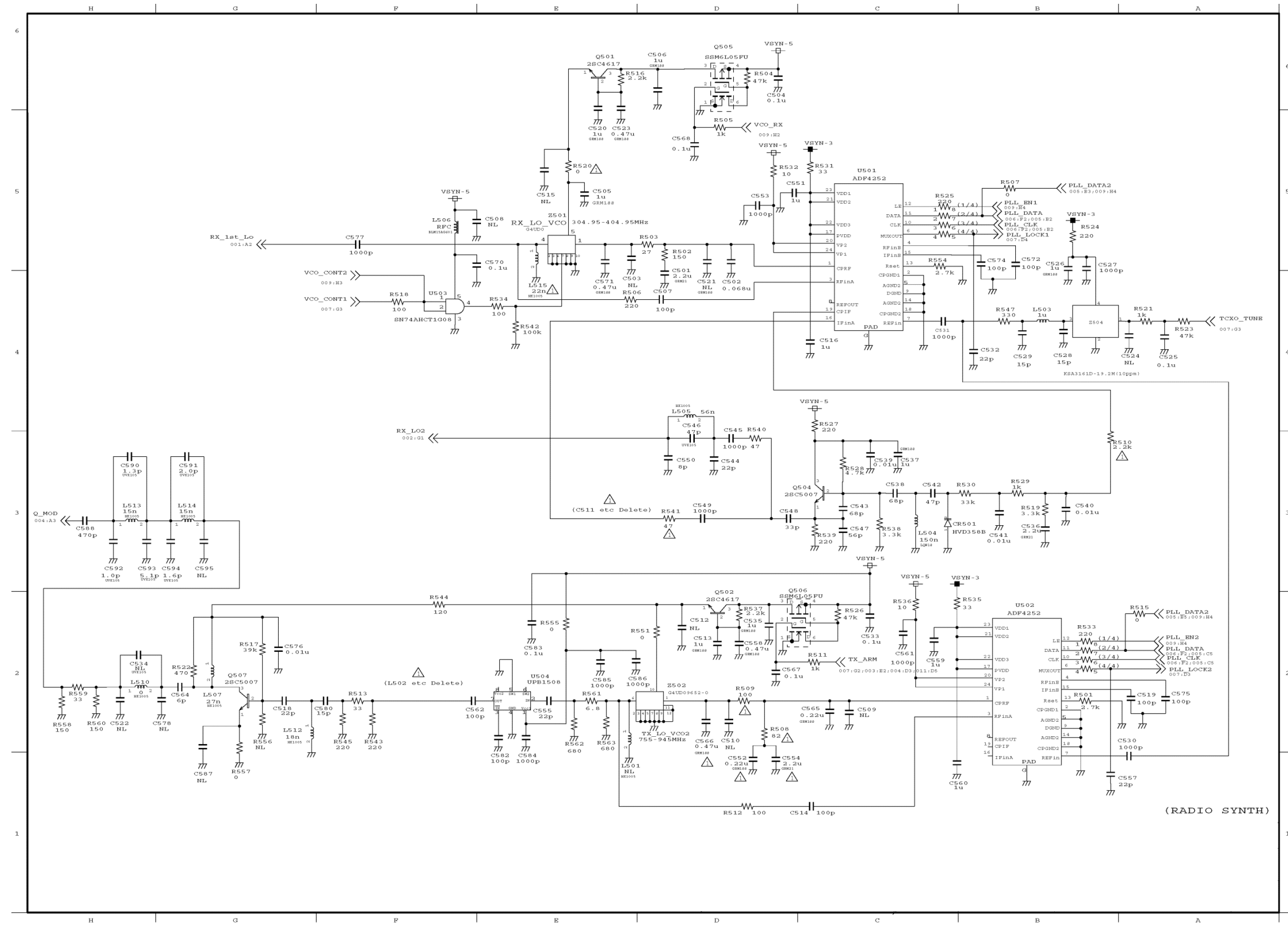
UHF-L (100 mW) MAIN SCHEMATIC DIAGRAM G3UD09920, Rev. 4, Page 5 of 12
