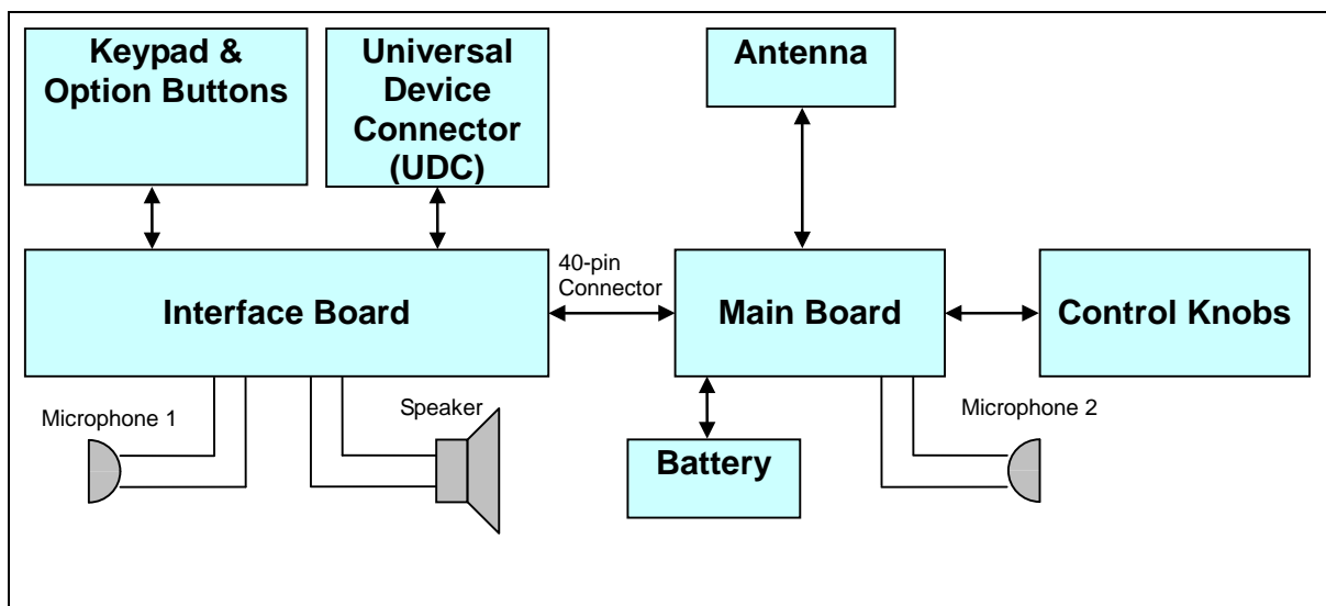
Figure 9-1: XG-75 Radio Block Diagram
