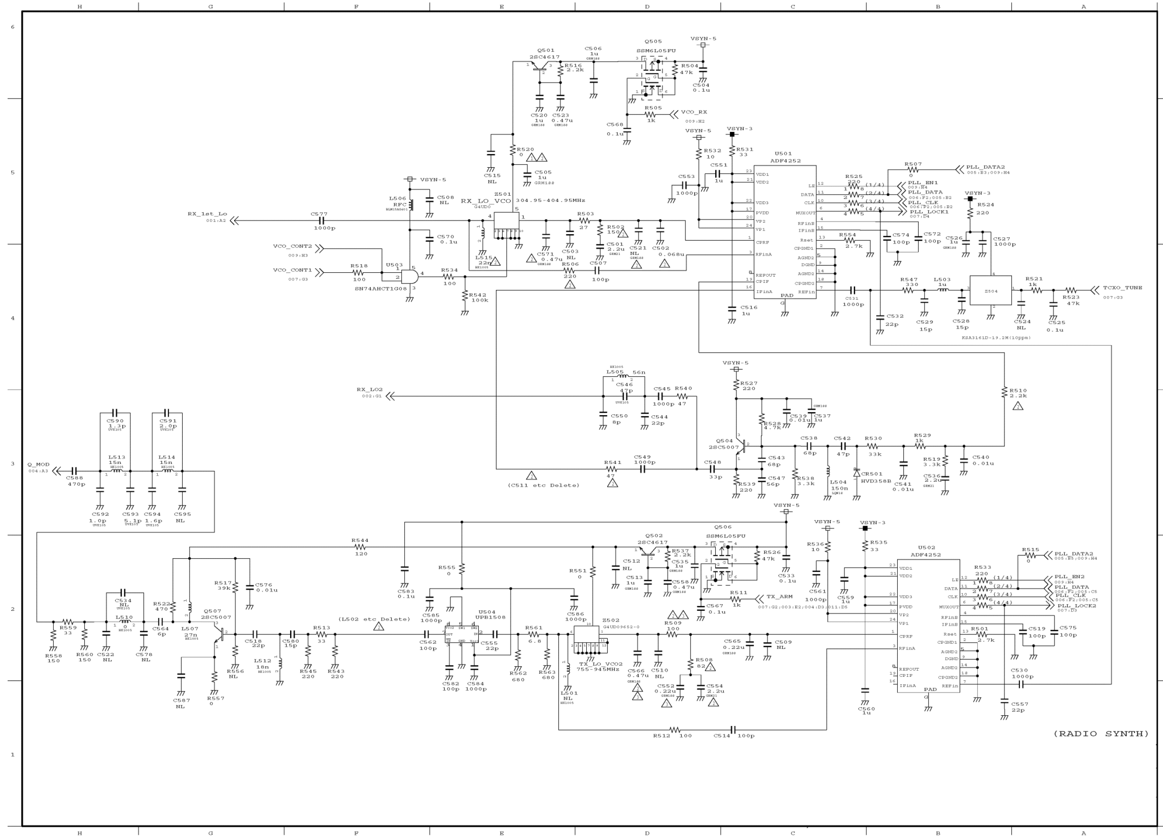
UHF-L (5 W) MAIN SCHEMATIC DIAGRAM G3UD09865, Rev. 6, Page 5 of 12
