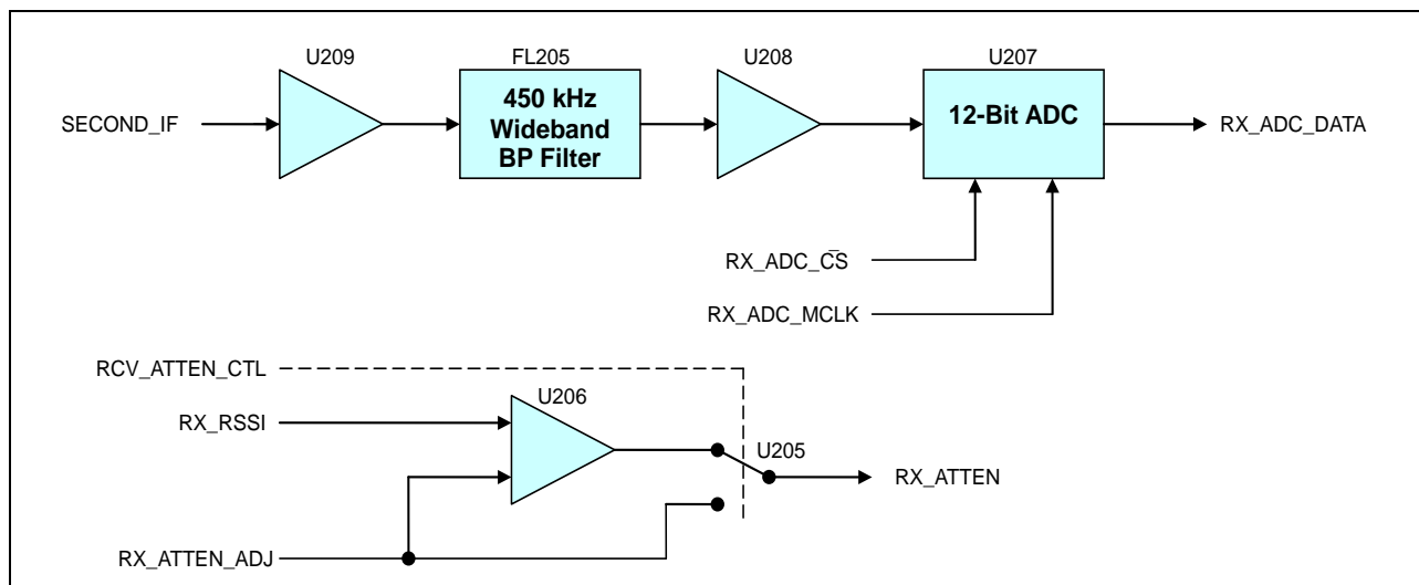
Figure 9-5: IF Amplifier Stage Block Diagram
