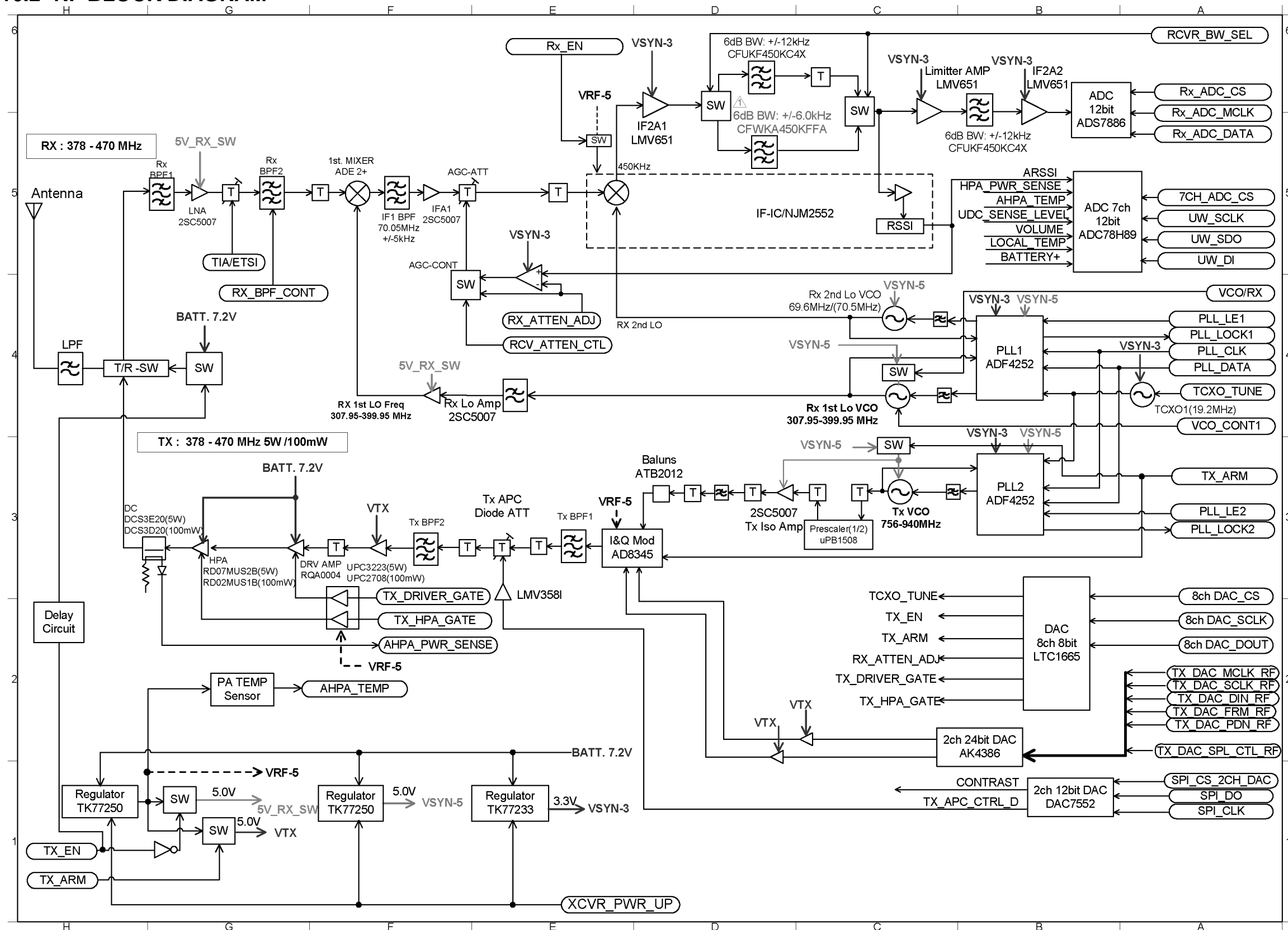
UHF-L RF BLOCK DIAGRAM G3UD10035, Rev. 1
