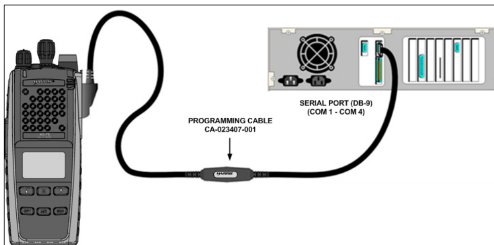
Figure 7-1: XG-75 Programming Setup
