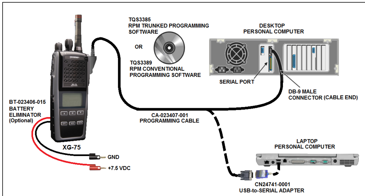
Figure 11-1: Programming Setup
