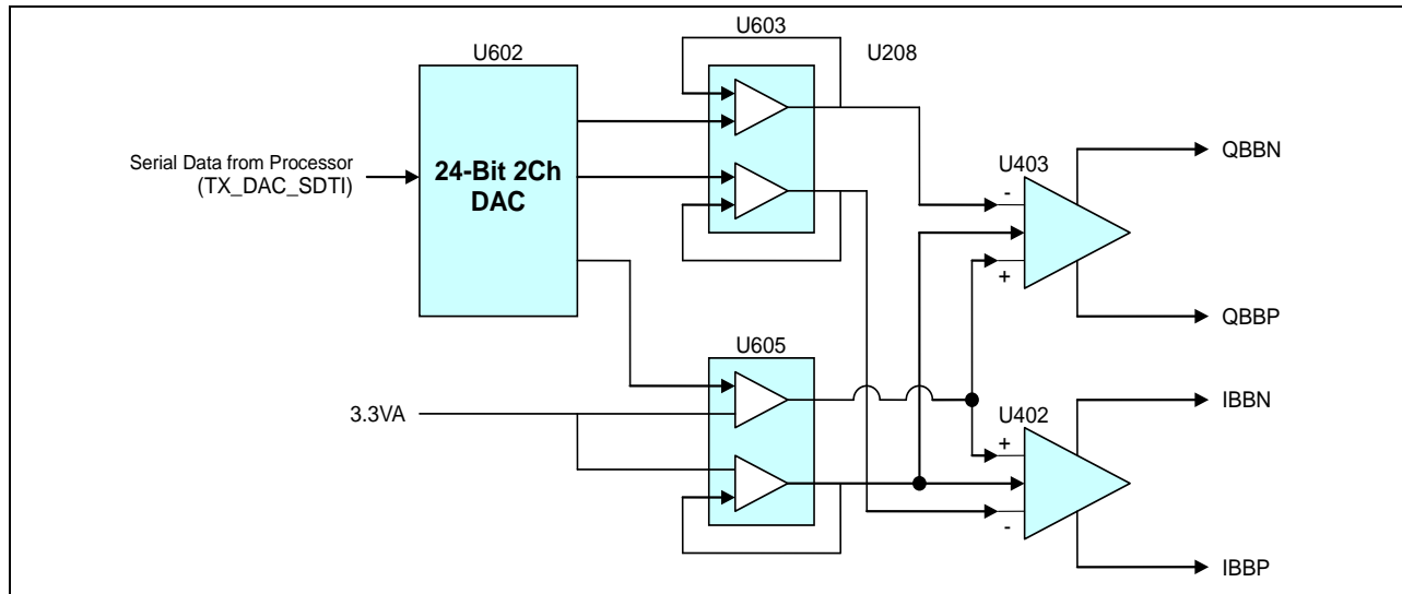
Figure 9-6: TX CODEC and Modulator Interface Block Diagram
