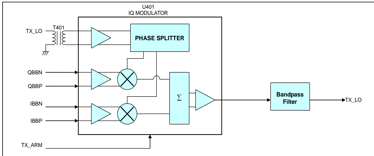
Figure 9-7: IQ Modulator Block Diagram
