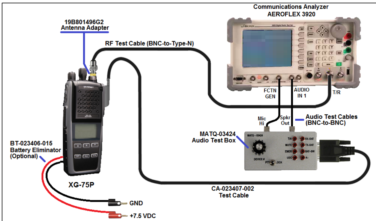
Figure 11-2: Test Equipment Connections for Radio Alignment
