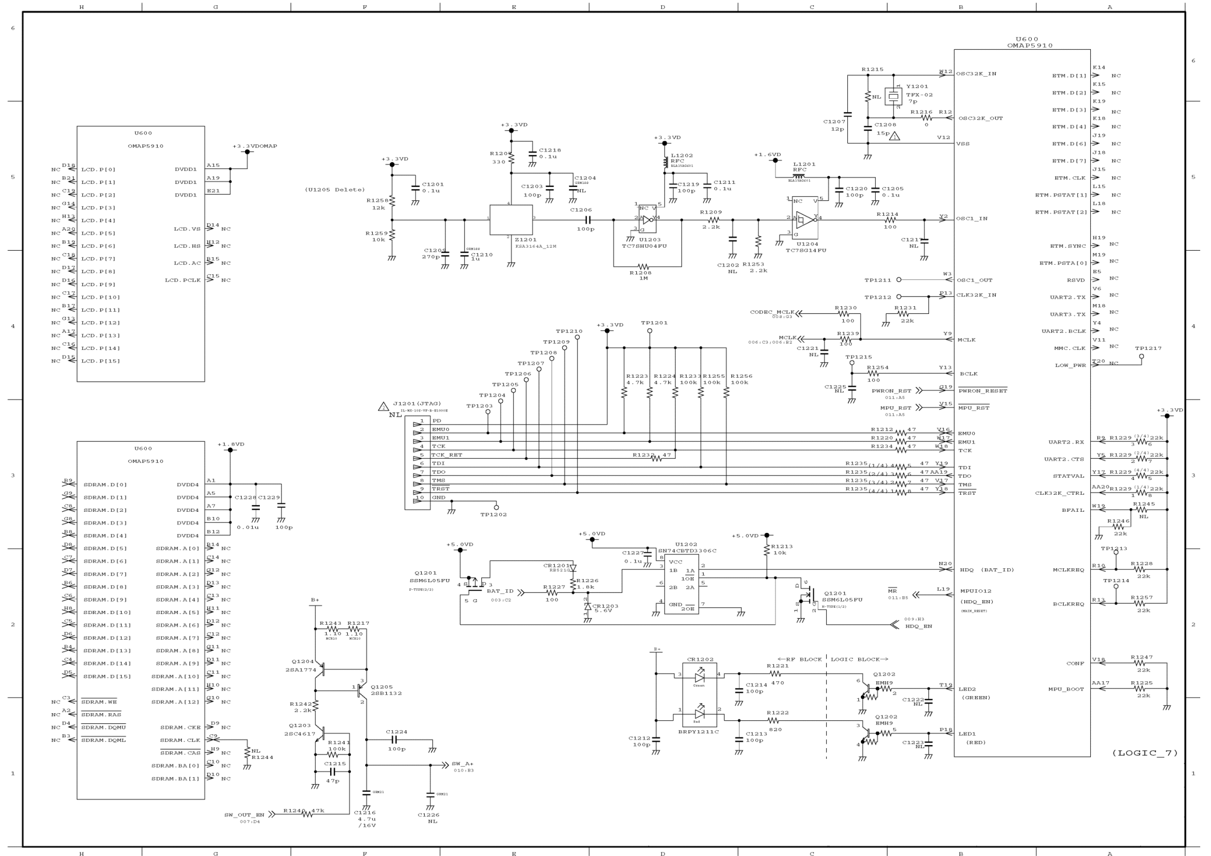
UHF-L (100 mW) MAIN SCHEMATIC DIAGRAM G3UD09920, Rev. 4, Page 12 of 12
