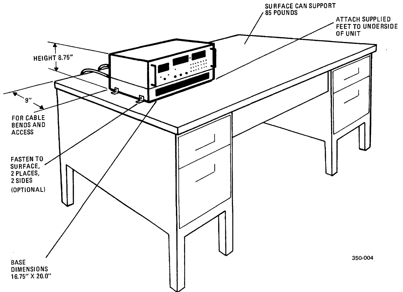
SURFACE MOUNT INSTALLATION DETAIL (DESK TOP SHOWN)
