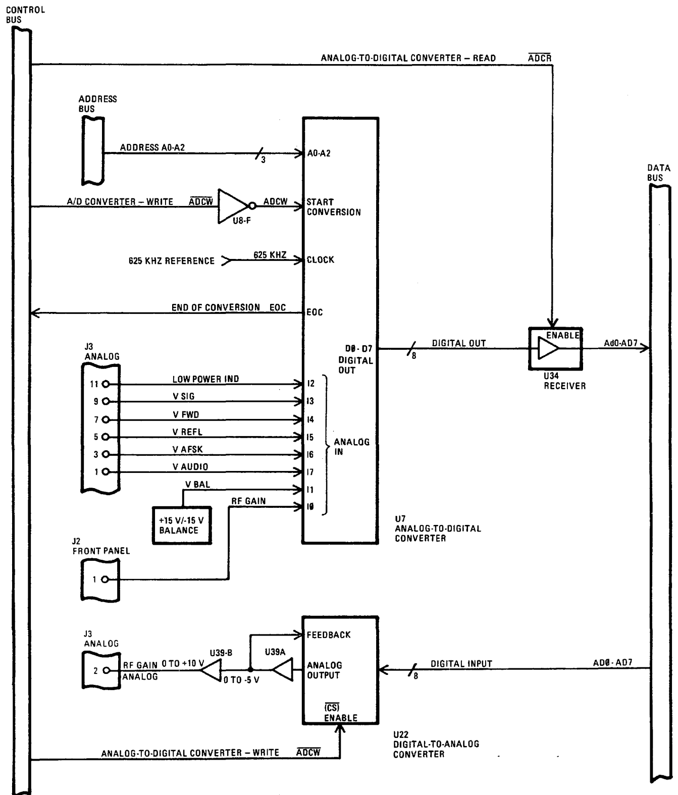
Figure 5-23. Simplified A/D - D/A Conversion Circuits
