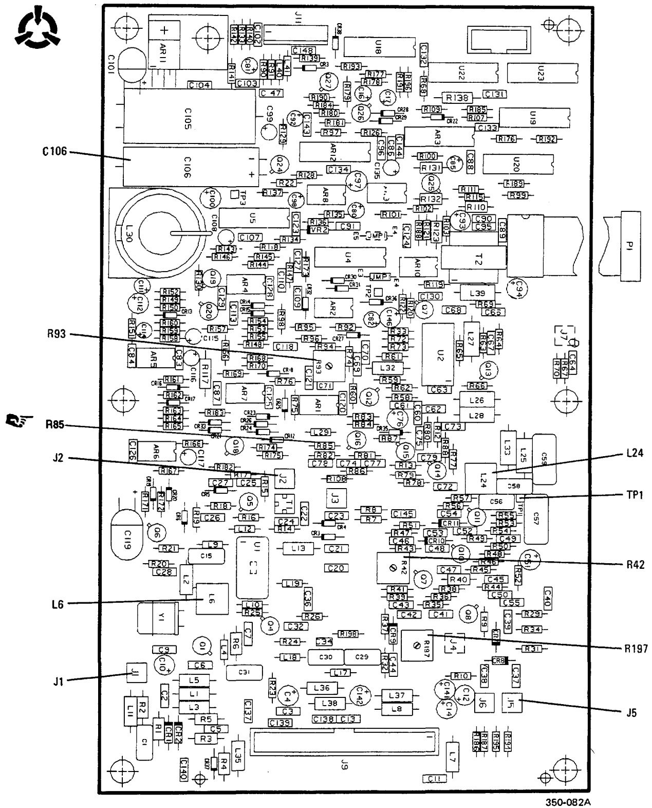
Figure 6-9. Receiver PWB Assy.
