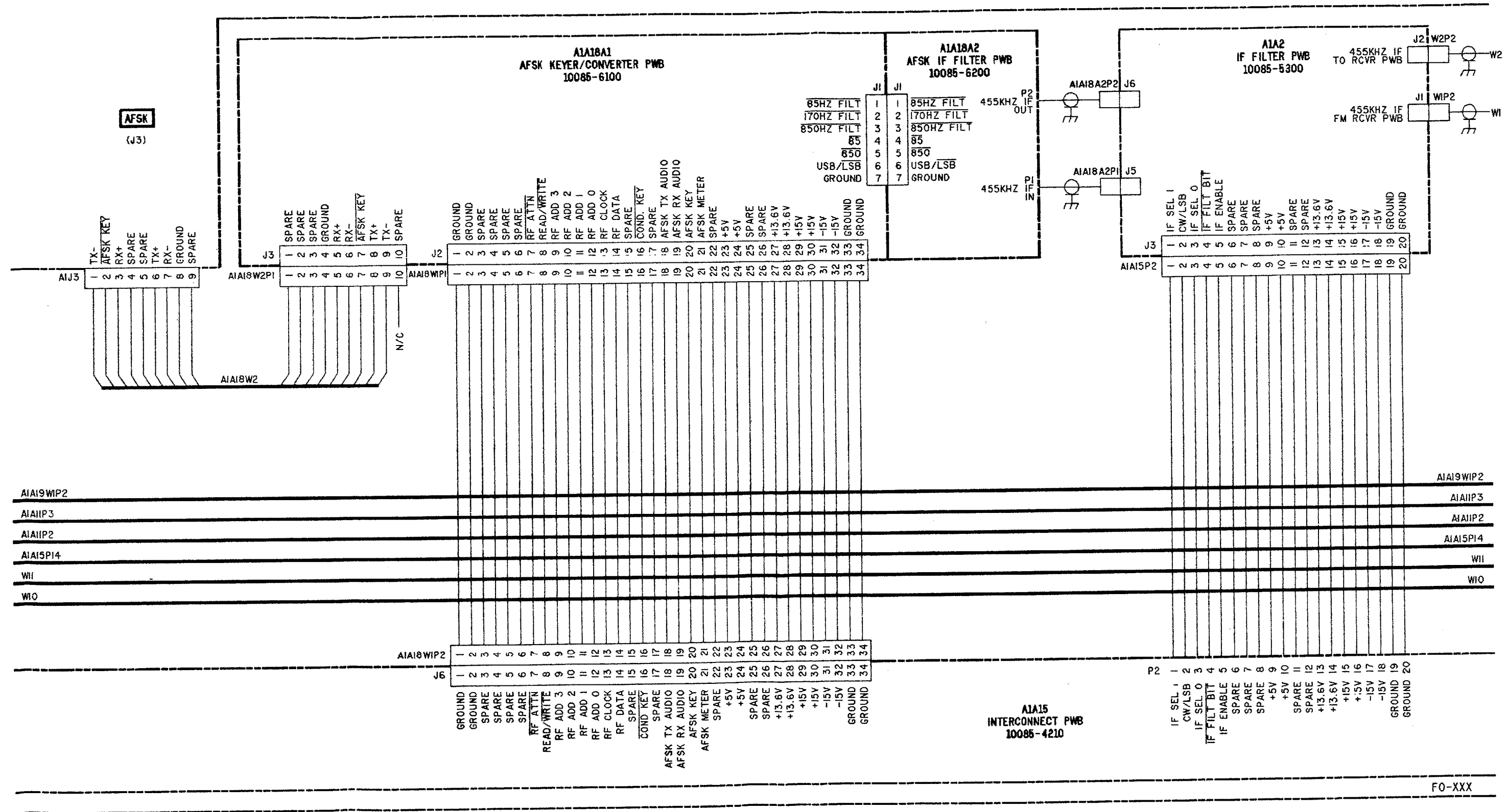
Figure FO-11. Interconnection Diagram (Sheet 4 of 13)
