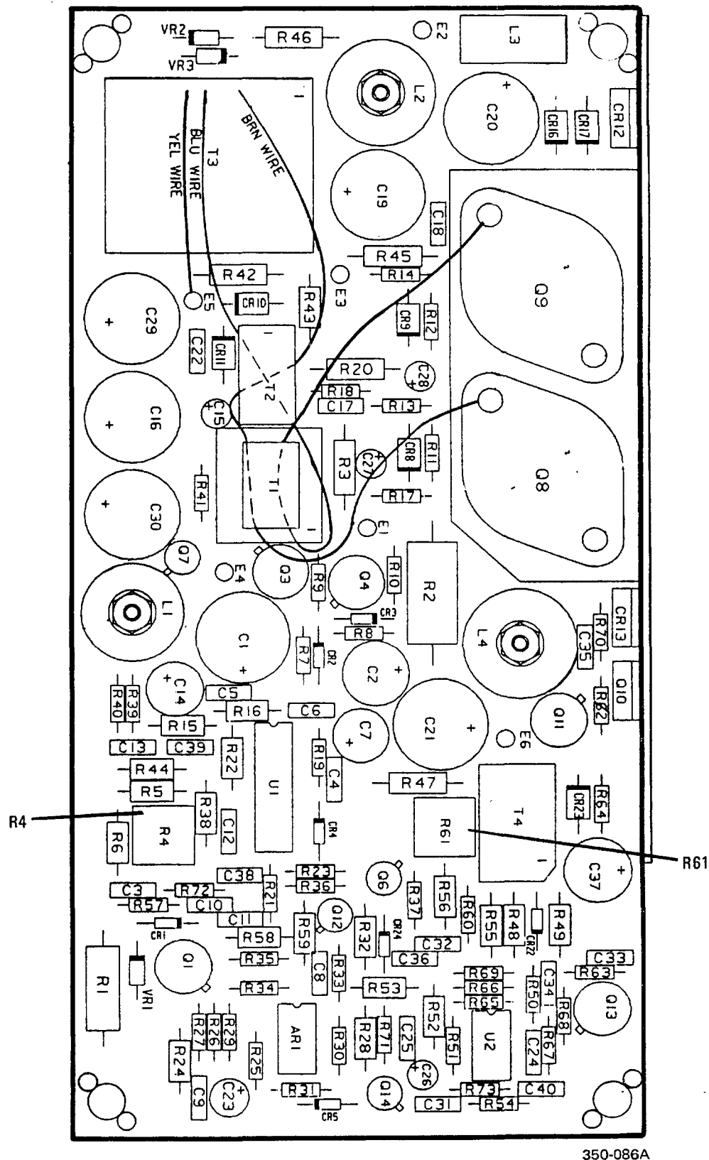
Figure 6-14. Multivoltage Supply PWB Assy.
