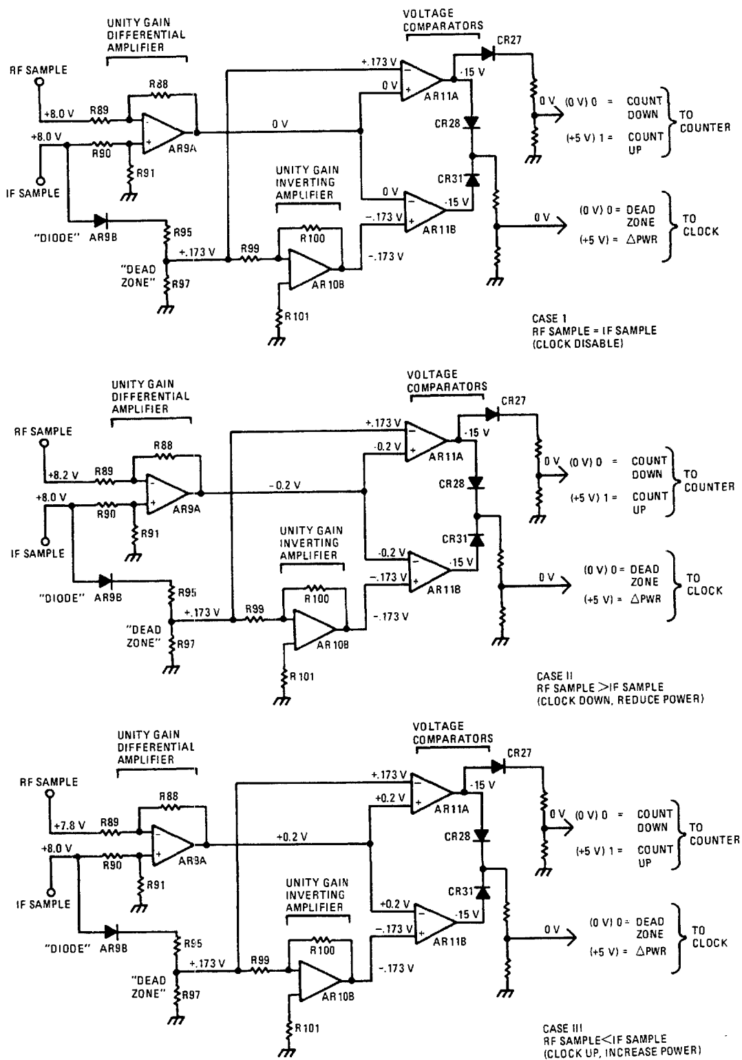
Figure 5-8. Simplified TGC Detector Operation
