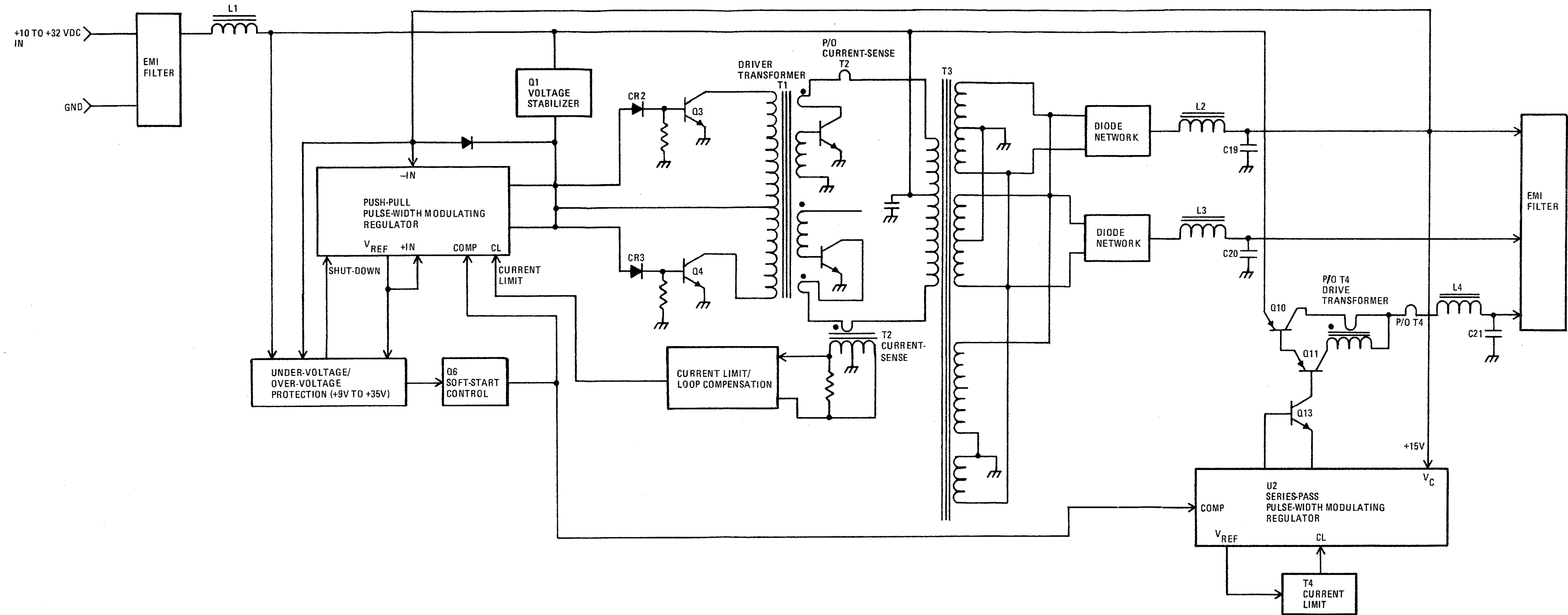
Figure FO-9. Multivoltage Power Supply Simplified Diagram.
