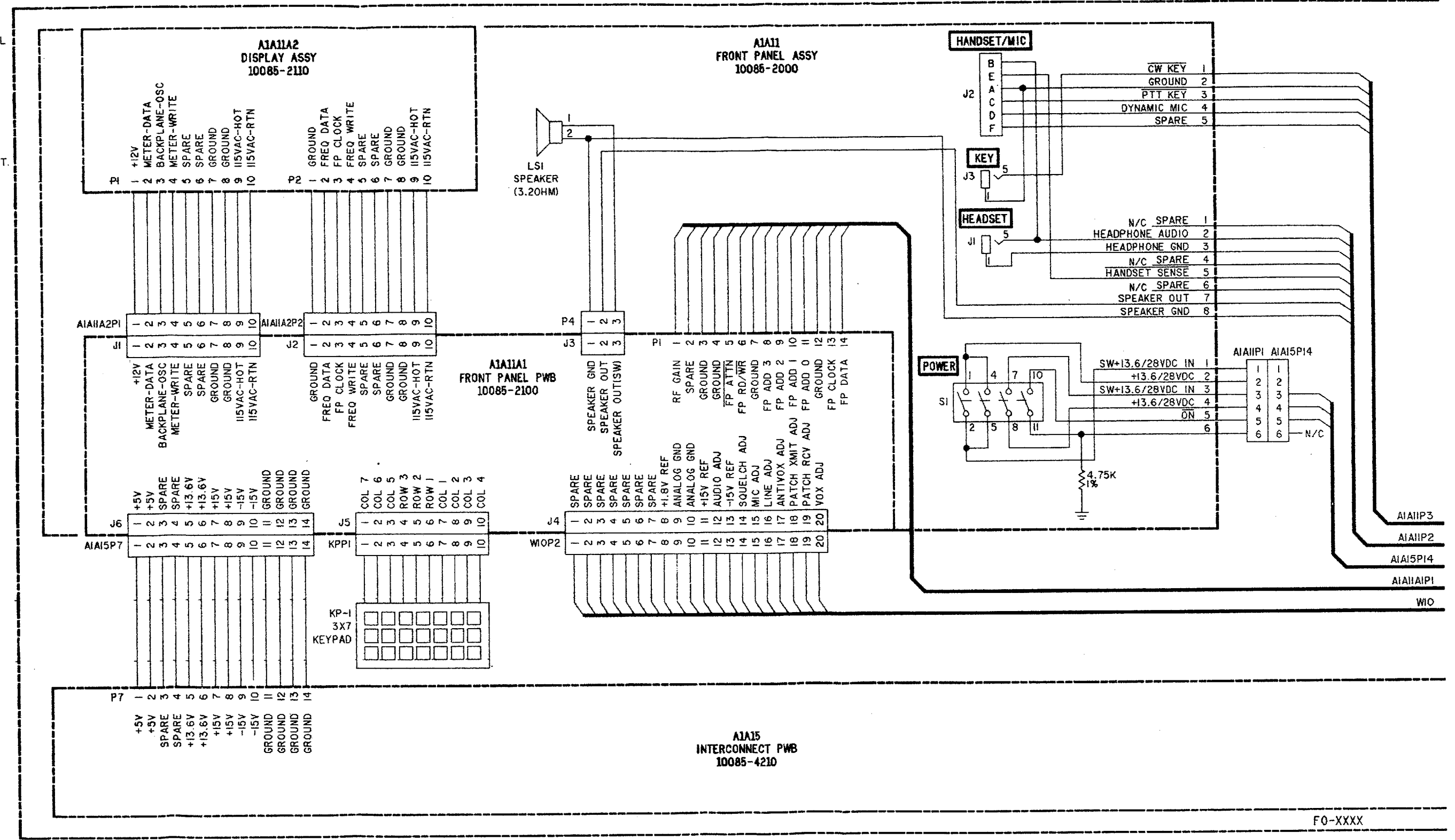
Figure FO-11. Interconnection Diagram. (Sheet 1 of 13)
