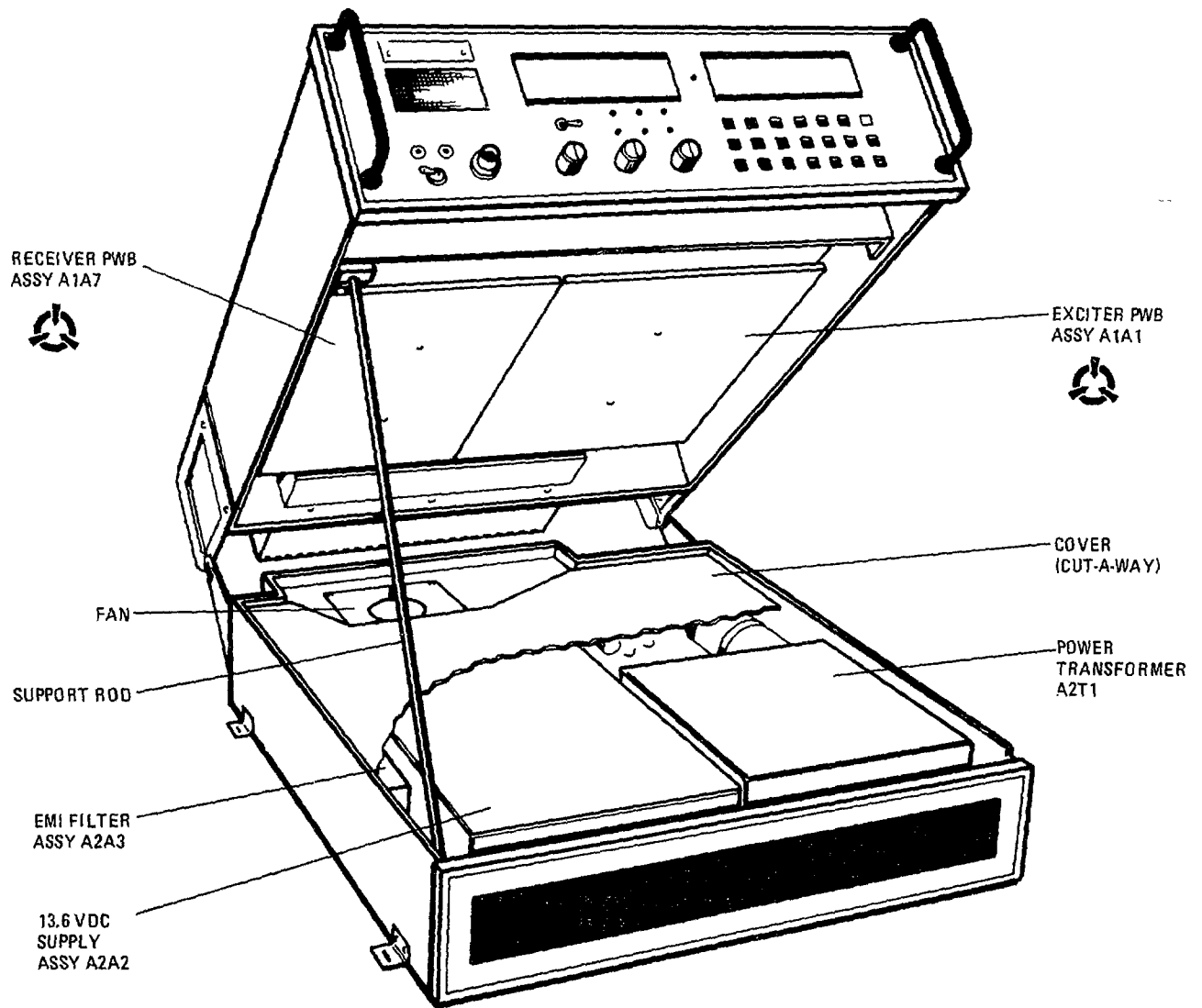
C. TRANSCEIVER ASSEMBLY UNLATCHED AND RAISED
