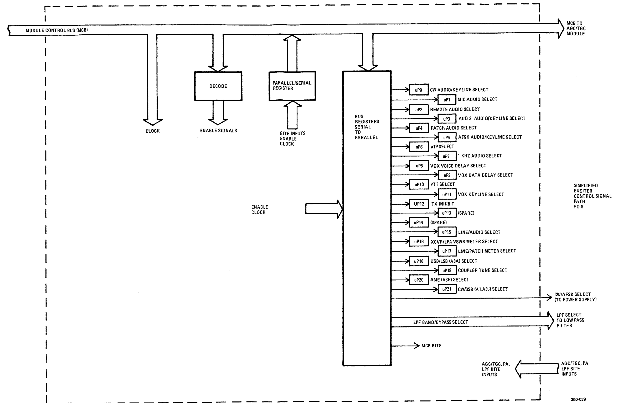
Figure FO-6. Simplified Exciter Control Signal Path.
