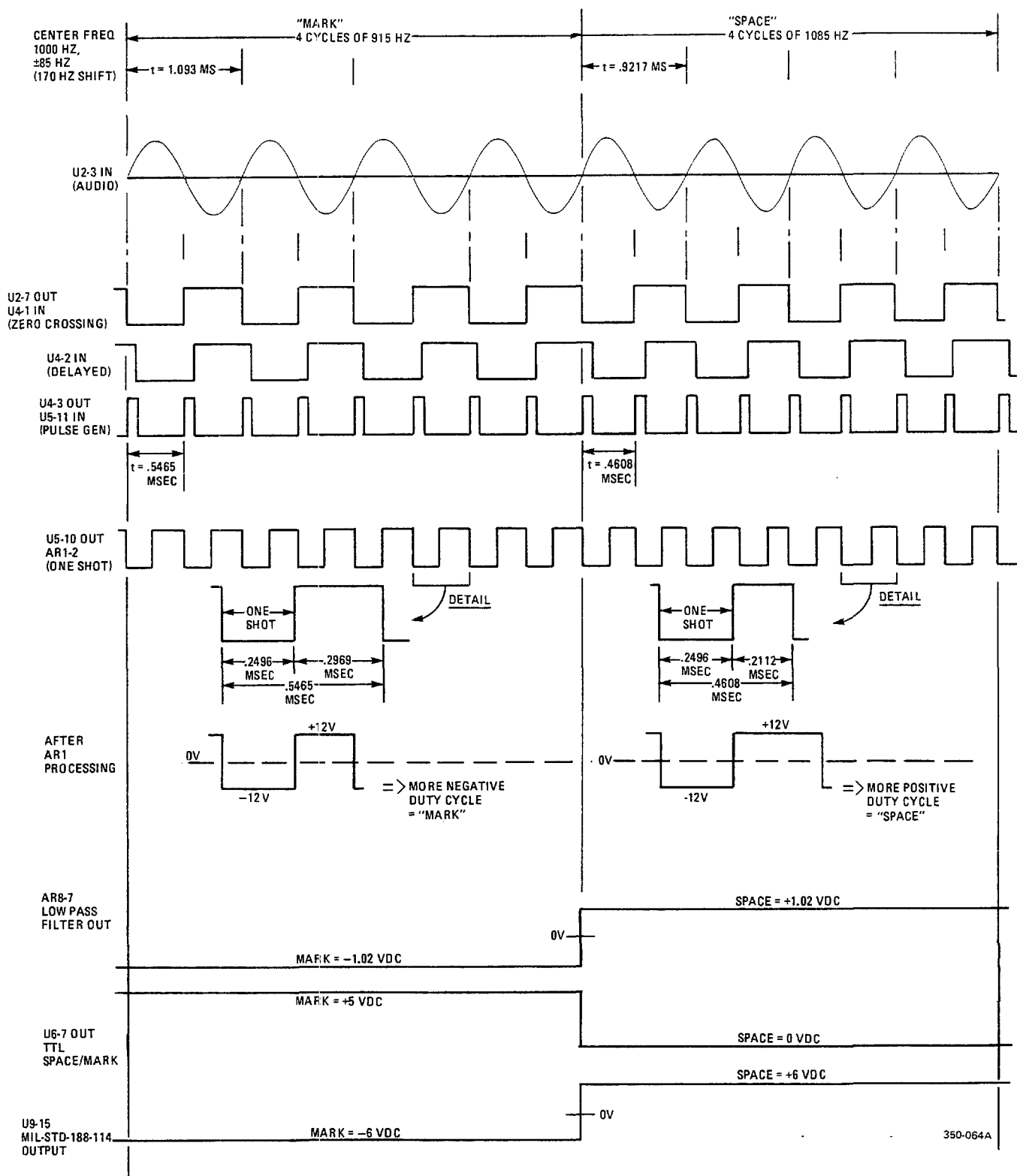
Figure 5-32. AFSK Converter Timing Diagram
