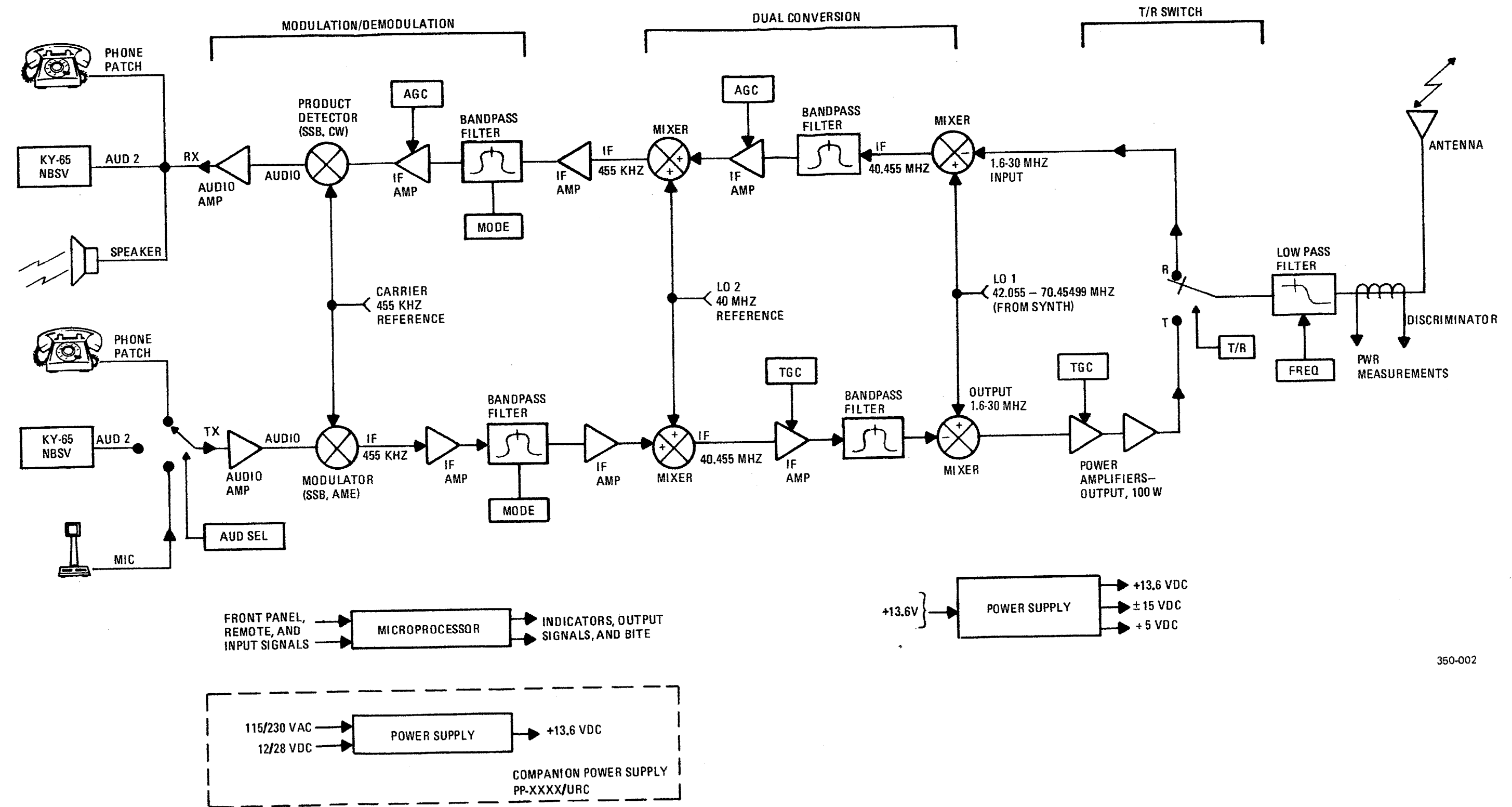
Figure FO-13. Simplified Functional Diagram, 100 Watt Transceiver
