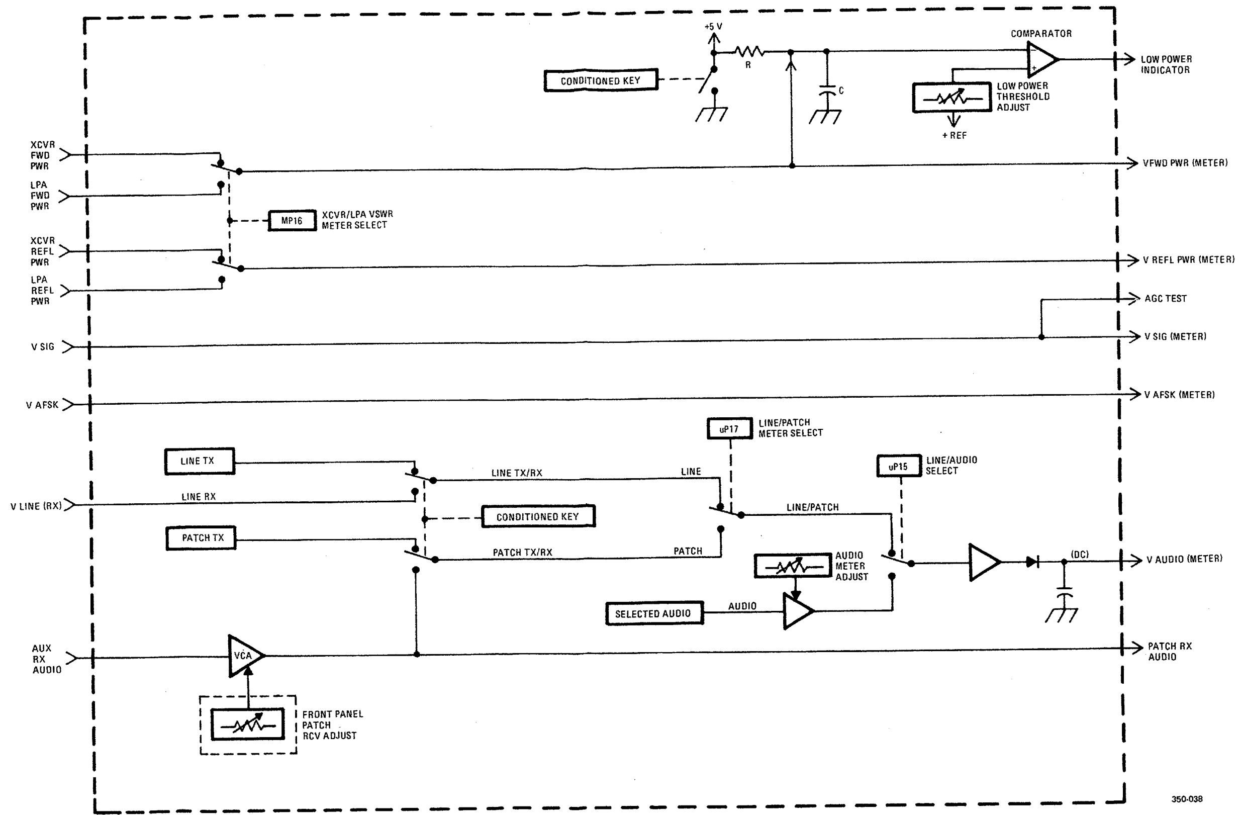
Figure FO-5. Simplified Exciter Meter Select Path.
