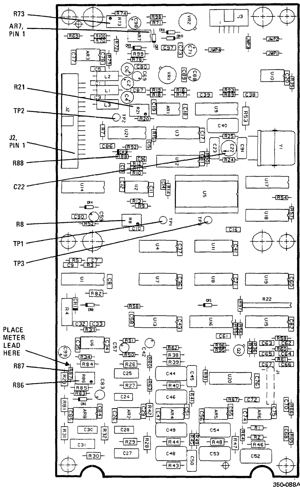
Figure 6-16. AFSK Keyer/Converter PWB Assy.
