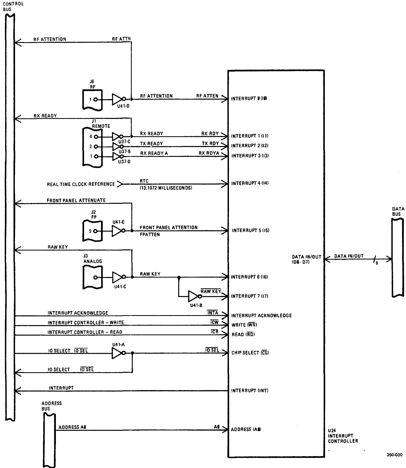
Figure 5-24. Simplified Interrupt Controller Circuits
