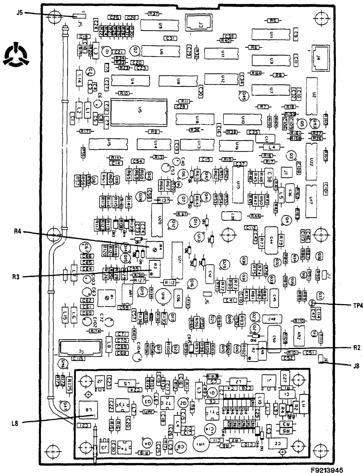
Figure 6-12. Synthesizer PWB Assy.
