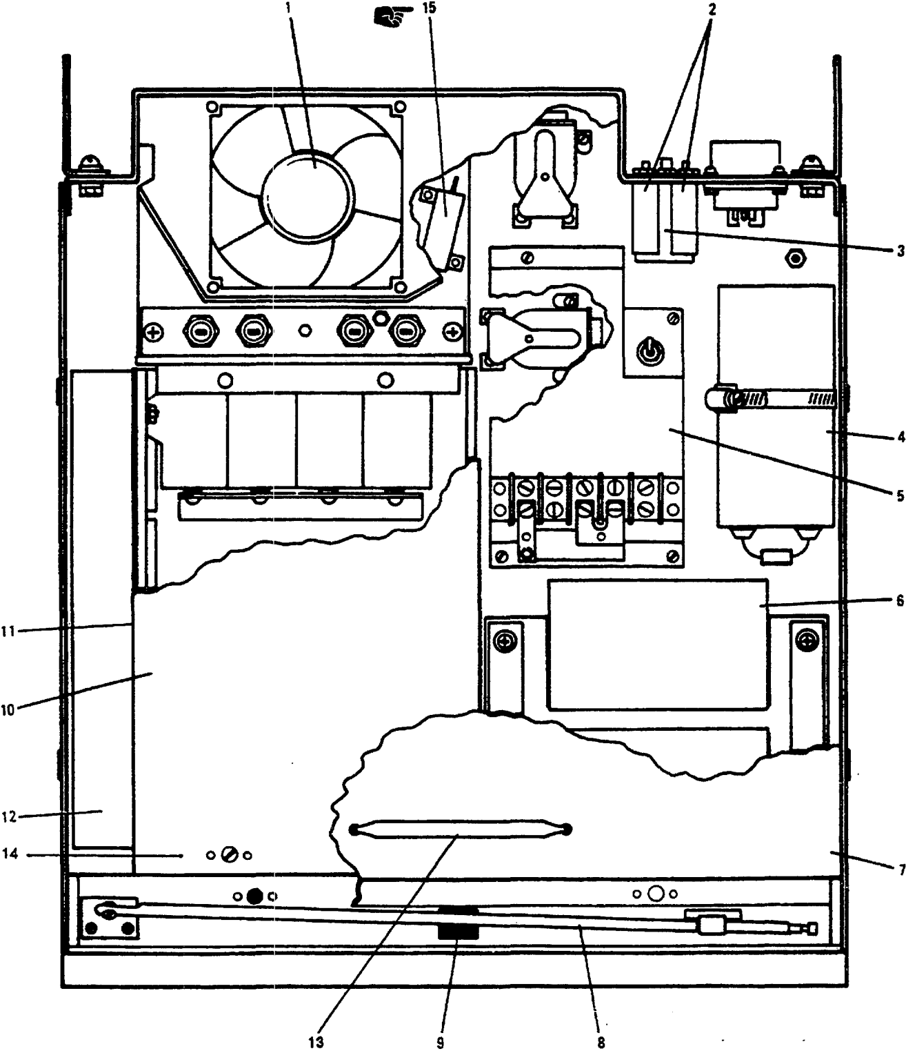
Figure 7-2. 100 Watt Transceiver, RT-1446/URC, Bottom Half
