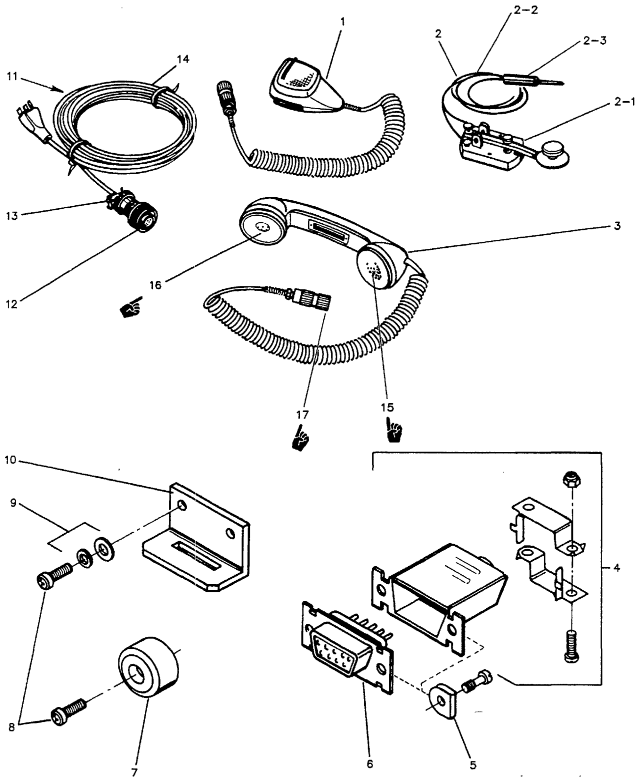
Figure 7-9. Installation Kit for the 100 Watt Transceiver
