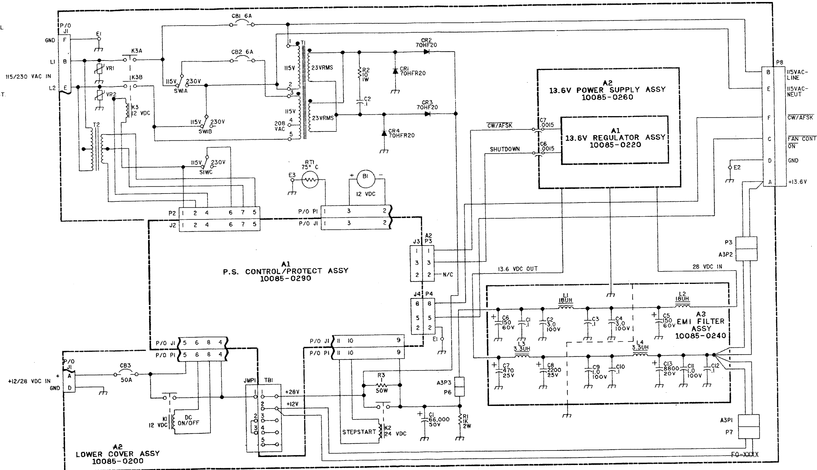
Figure FO-12. Interconnection Diagram, Power Supply Assembly
