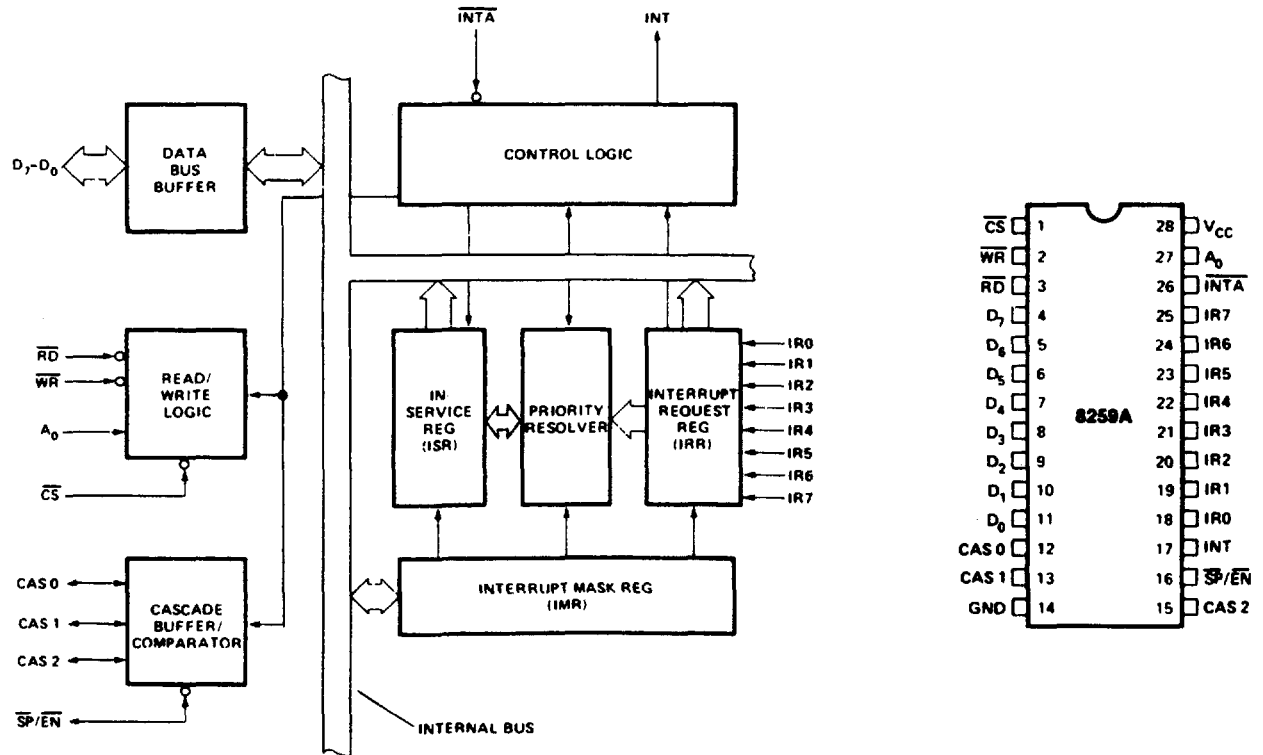
8259 BLOCK DIAGRAM
