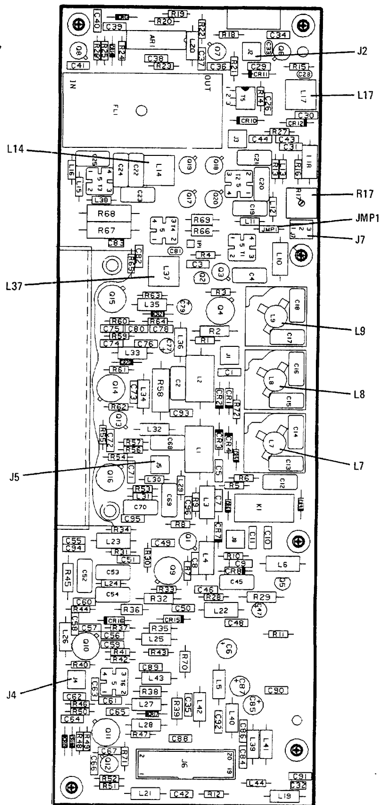
Figure 6-5. First Converter PWB Assy.
