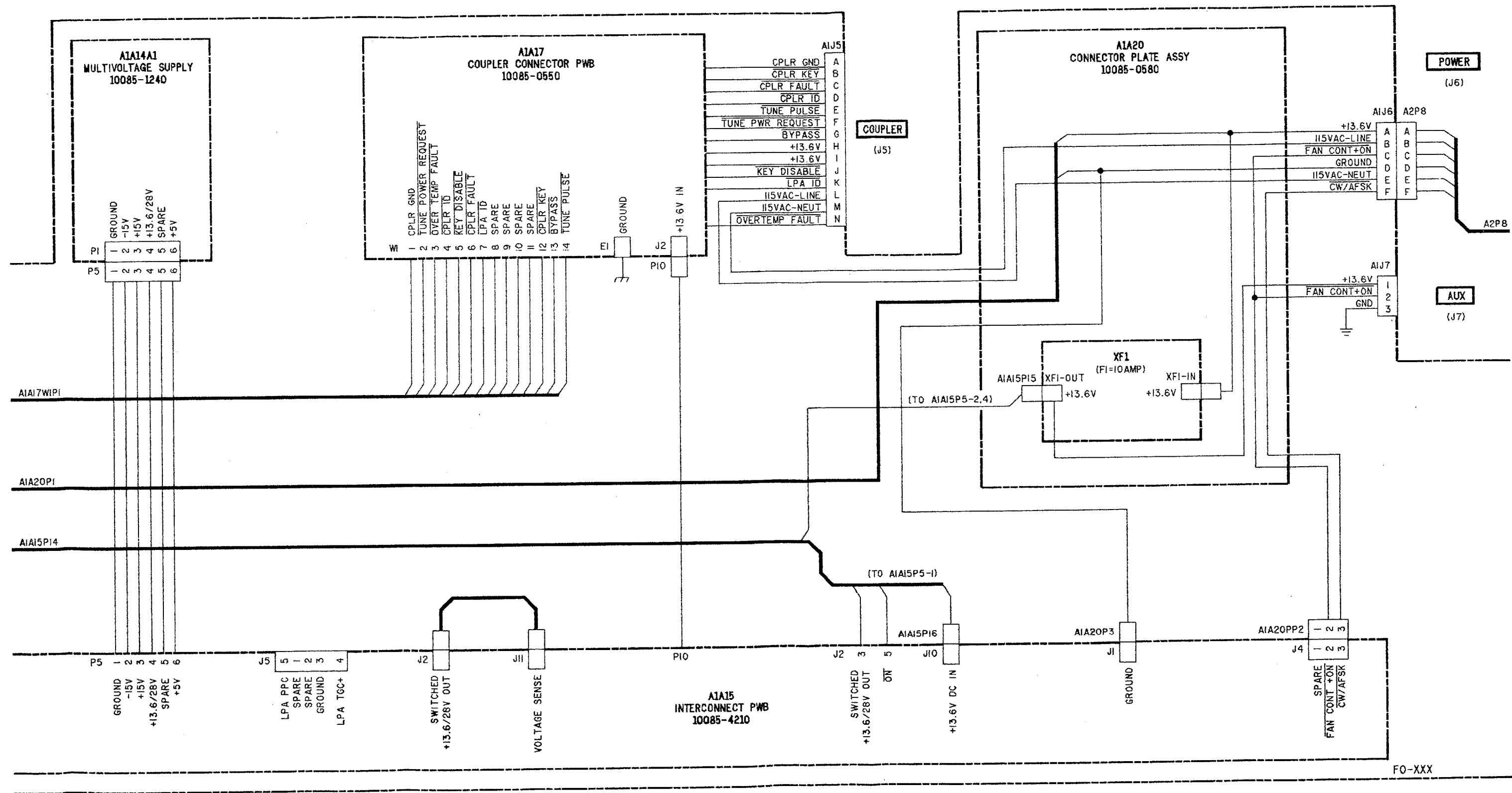
Figure FO-11. Interconnection Diagram. (Sheet 12 of 13)
