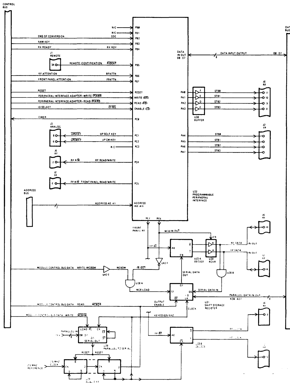
Figure 5-26. Simplified Programmable Peripheral Interface Circuits
