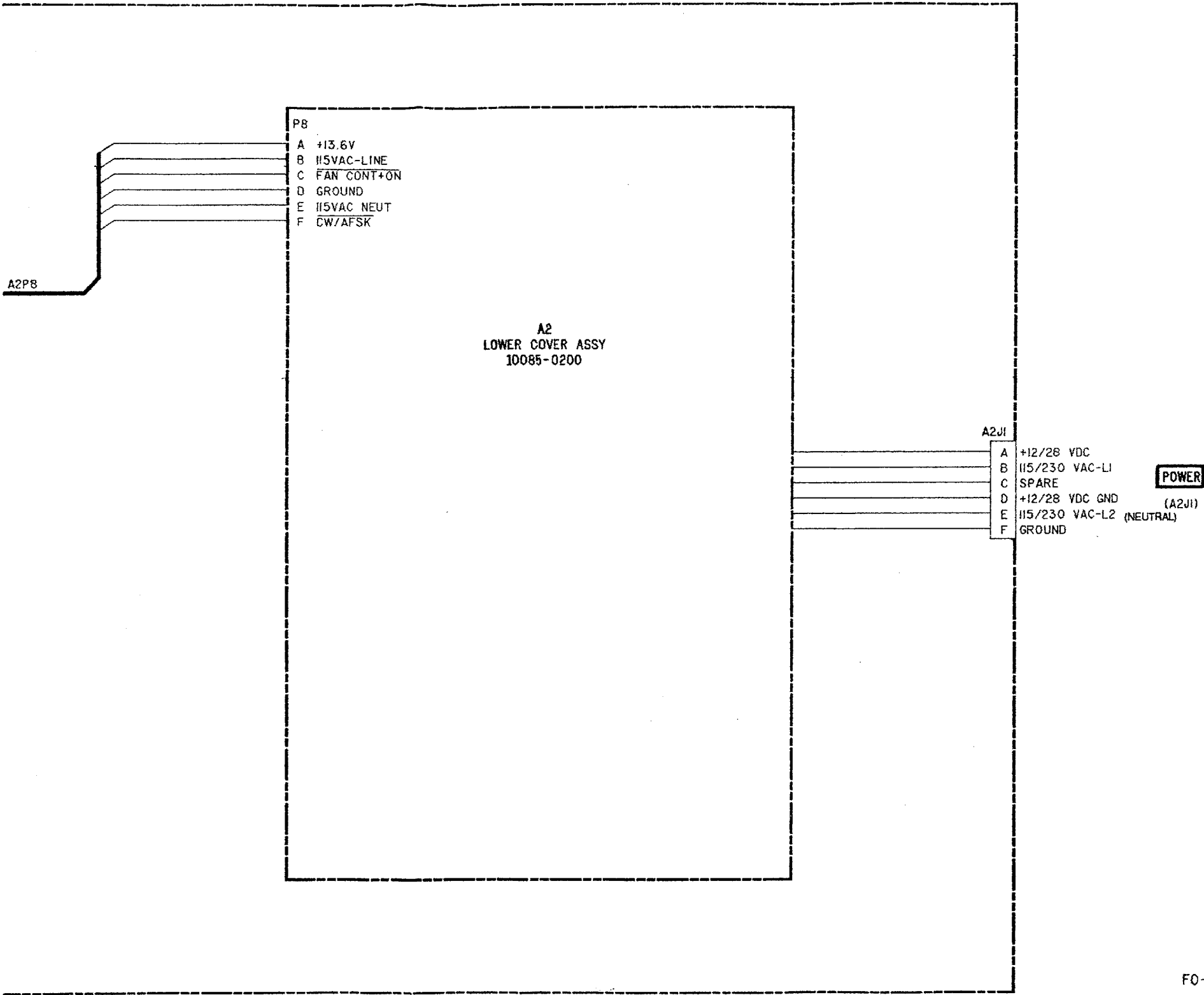
Figure FO-11. Interconnection Diagram. (Sheet 13 of 13)
