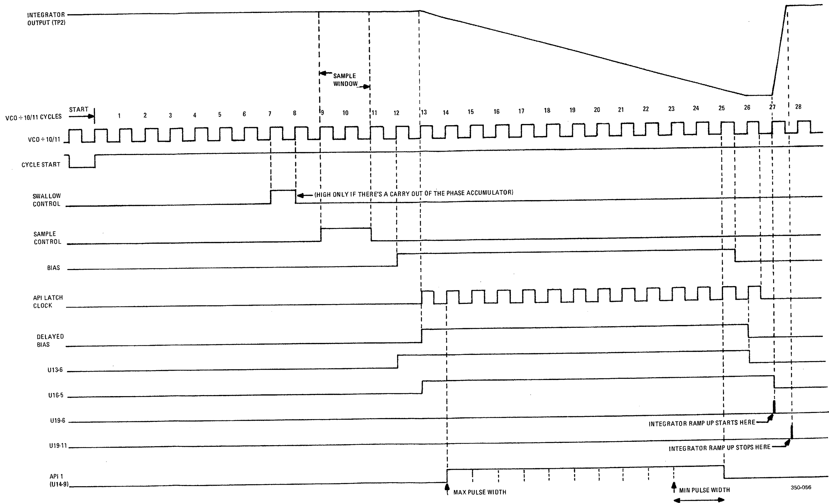
Figure FO-7. Synthesizer Integrator Timing Diagram.
