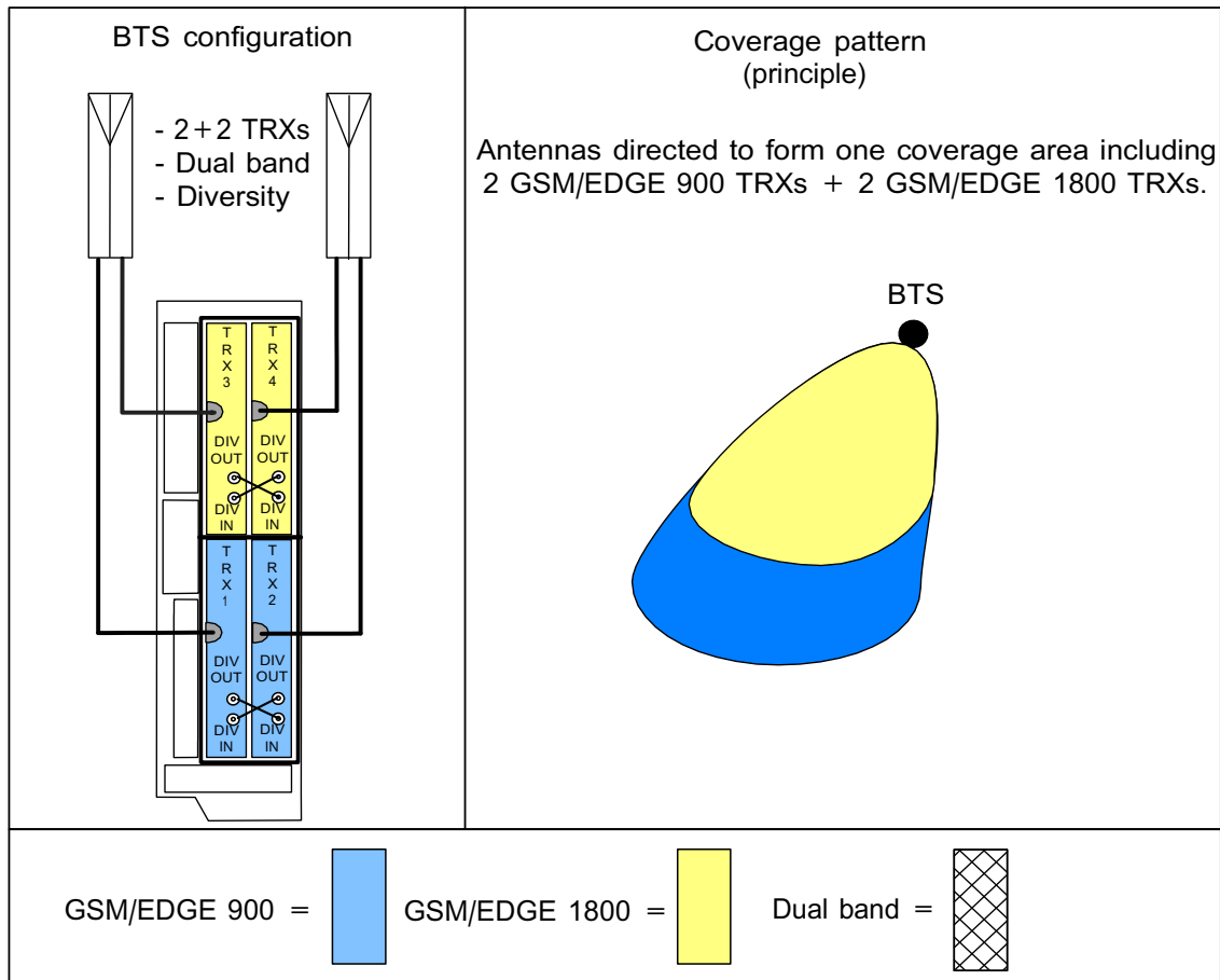
Figure 9. 2+2 dual band configuration
