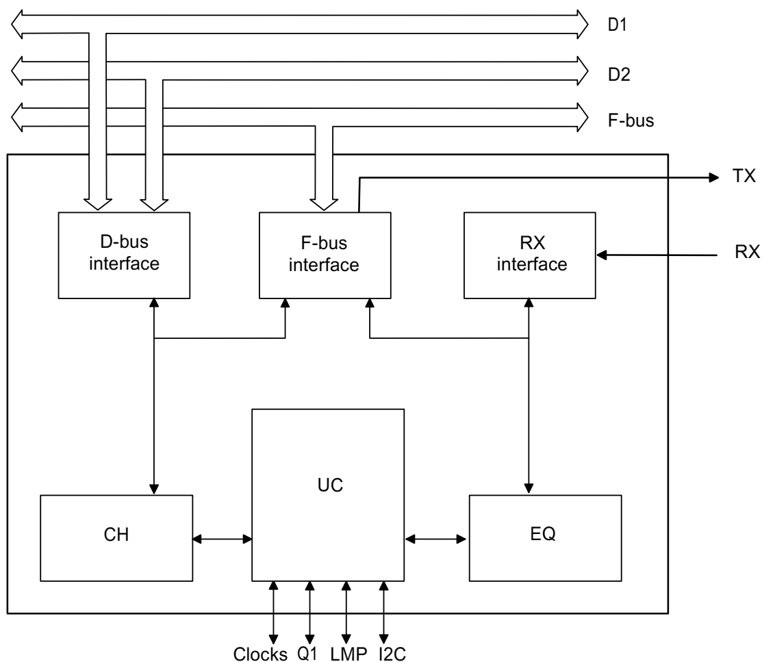
Figure 20. Block diagram of the baseband module
