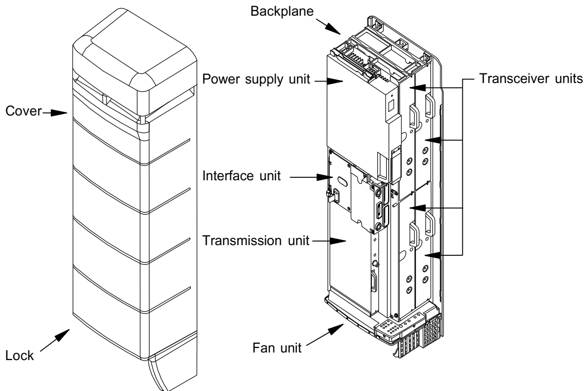
Figure 17. Arrangement of units
