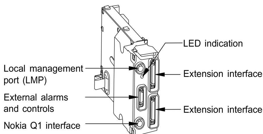
Figure 22. Interface unit of the Nokia MetroSite EDGE Base Station
