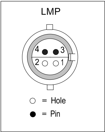
Figure 23. Pin order of the LMP connector
