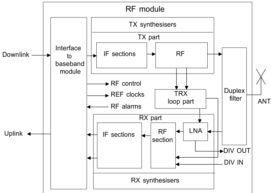
Figure 21. Block diagram of the RF module
