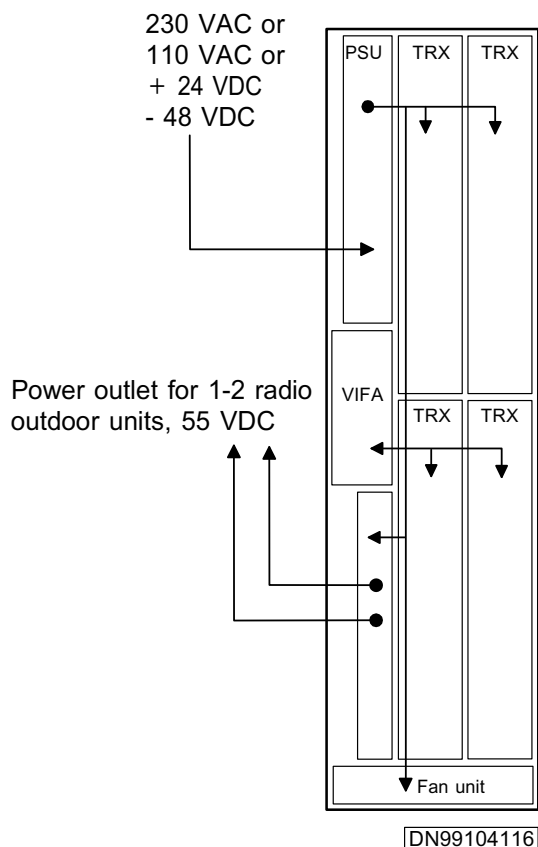
Figure 15. Power distribution in the Nokia MetroSite EDGE Base Station
