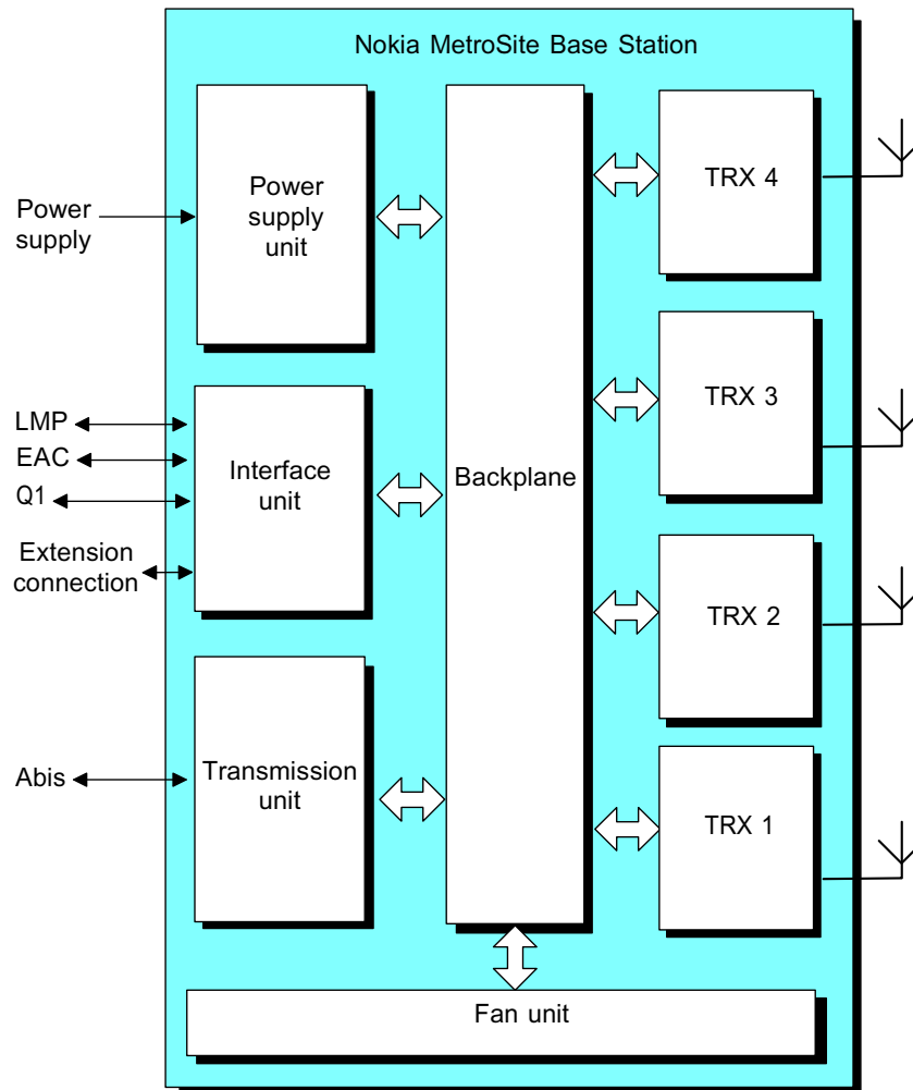
Figure 14. Nokia MetroSite EDGE Base Station block diagram
