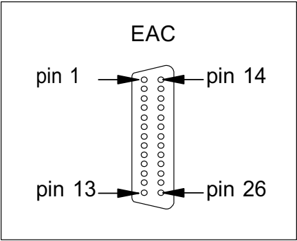
Figure 25. Pin order of the EAC connector
