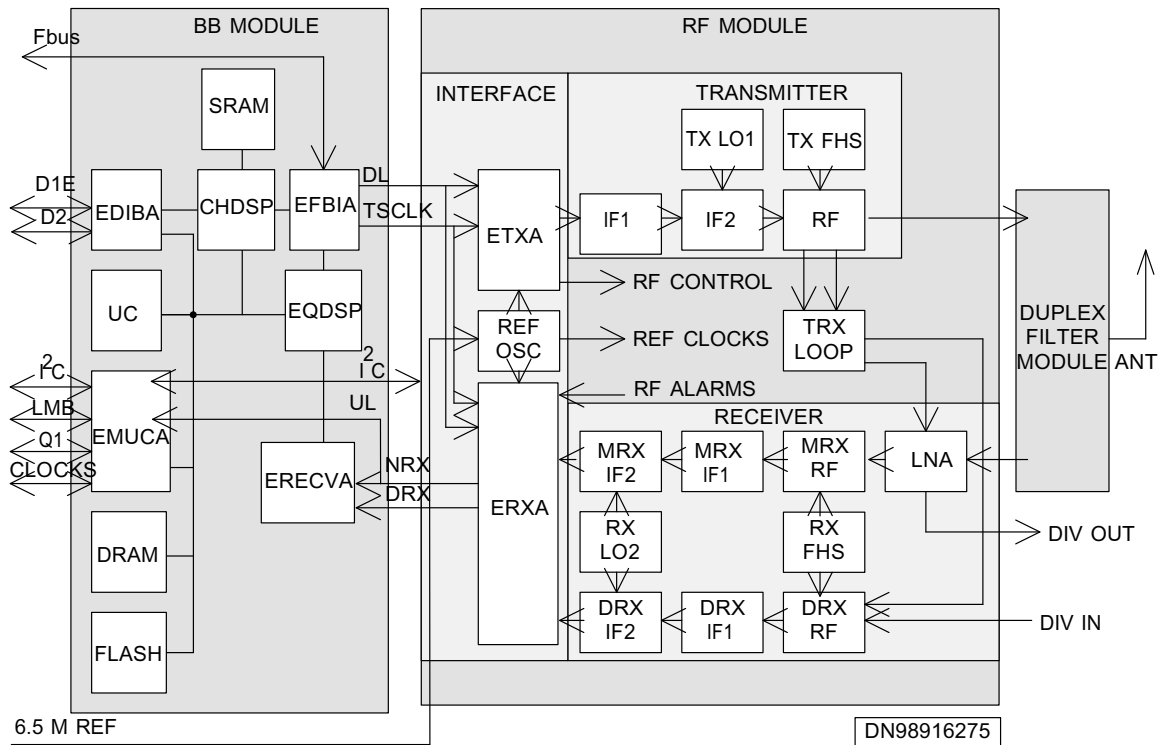
Figure 19. Block diagram of a Nokia MetroSite TRX
