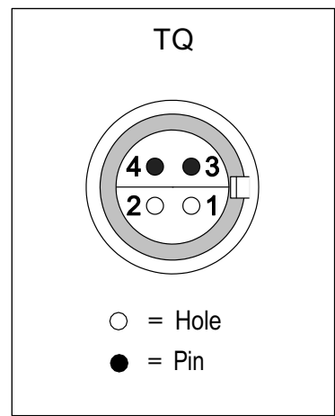
Figure 27. Pin order of a balanced TQ connector
