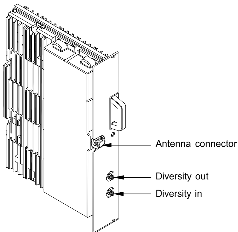
Figure 18. Transceiver unit
