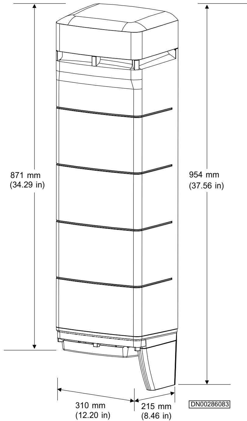
Figure 16. Dimensions of the Nokia MetroSite EDGE Base Station
