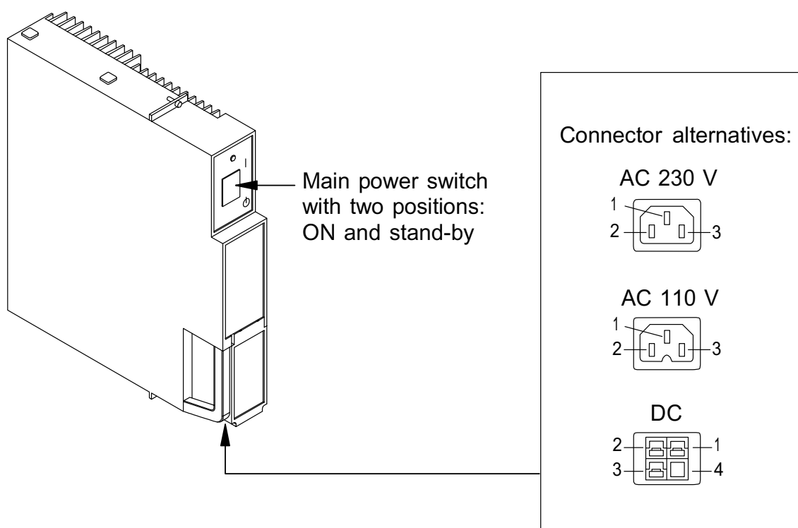
Figure 29. Power supply unit
