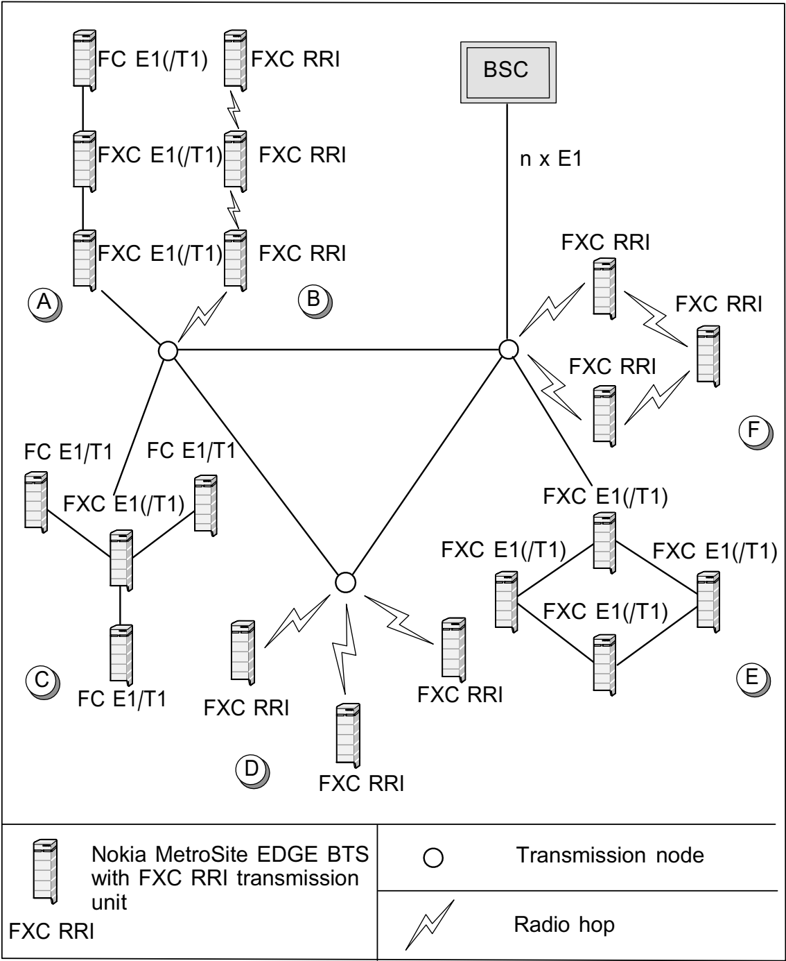
Figure 11. Examples of transmission connections
