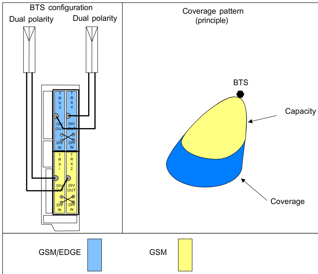
Figure 10. Intelligent coverage enhancement configuration
