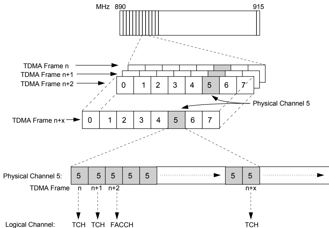
Figure 4-1 The TDMA channel concept
