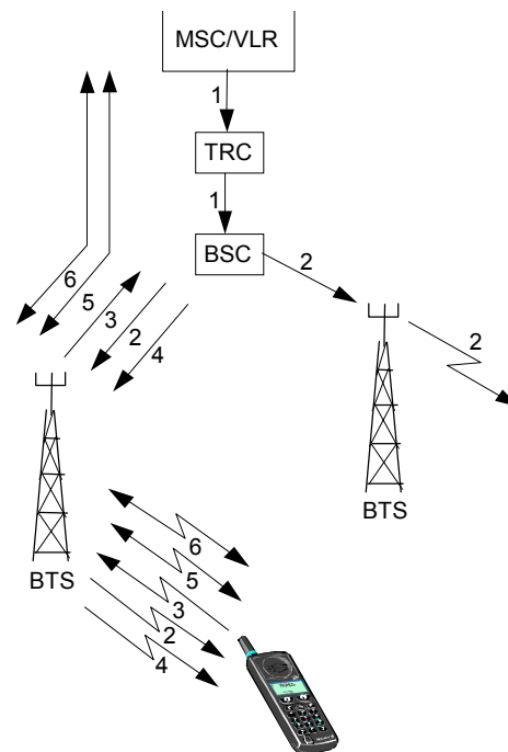
Figure 4-7 Call to an MS
