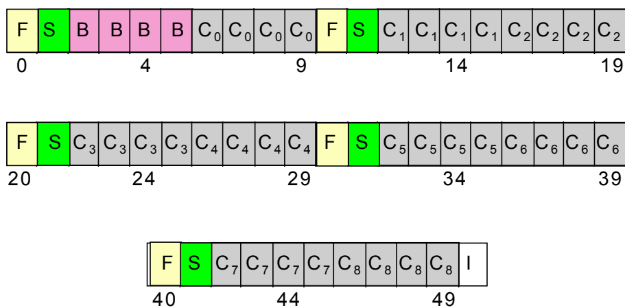
Figure 4-4 Multiplexing of BCH's and CCCHs on TS0
