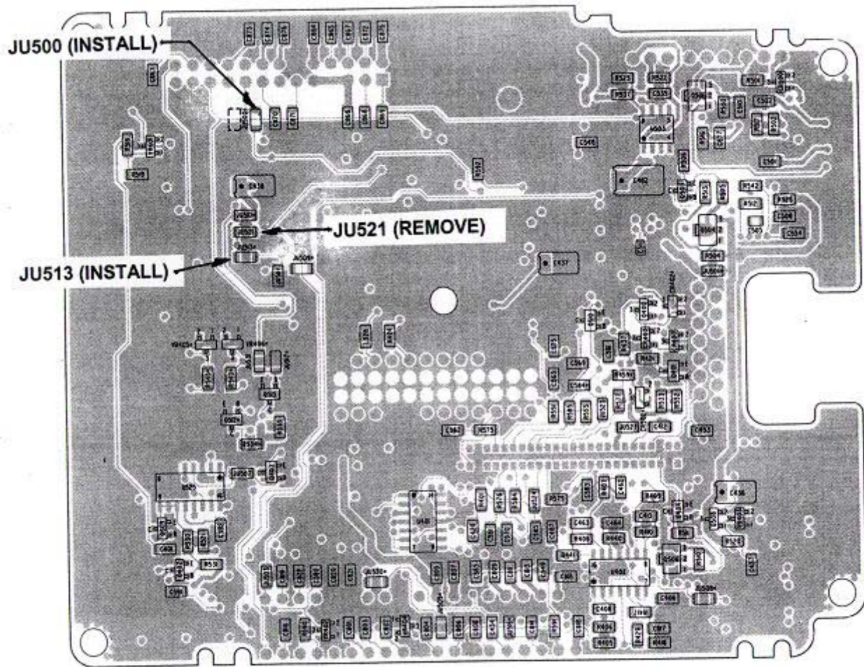
FIGURE 2. COMMAND BOARD - BOTTOM VIEW
