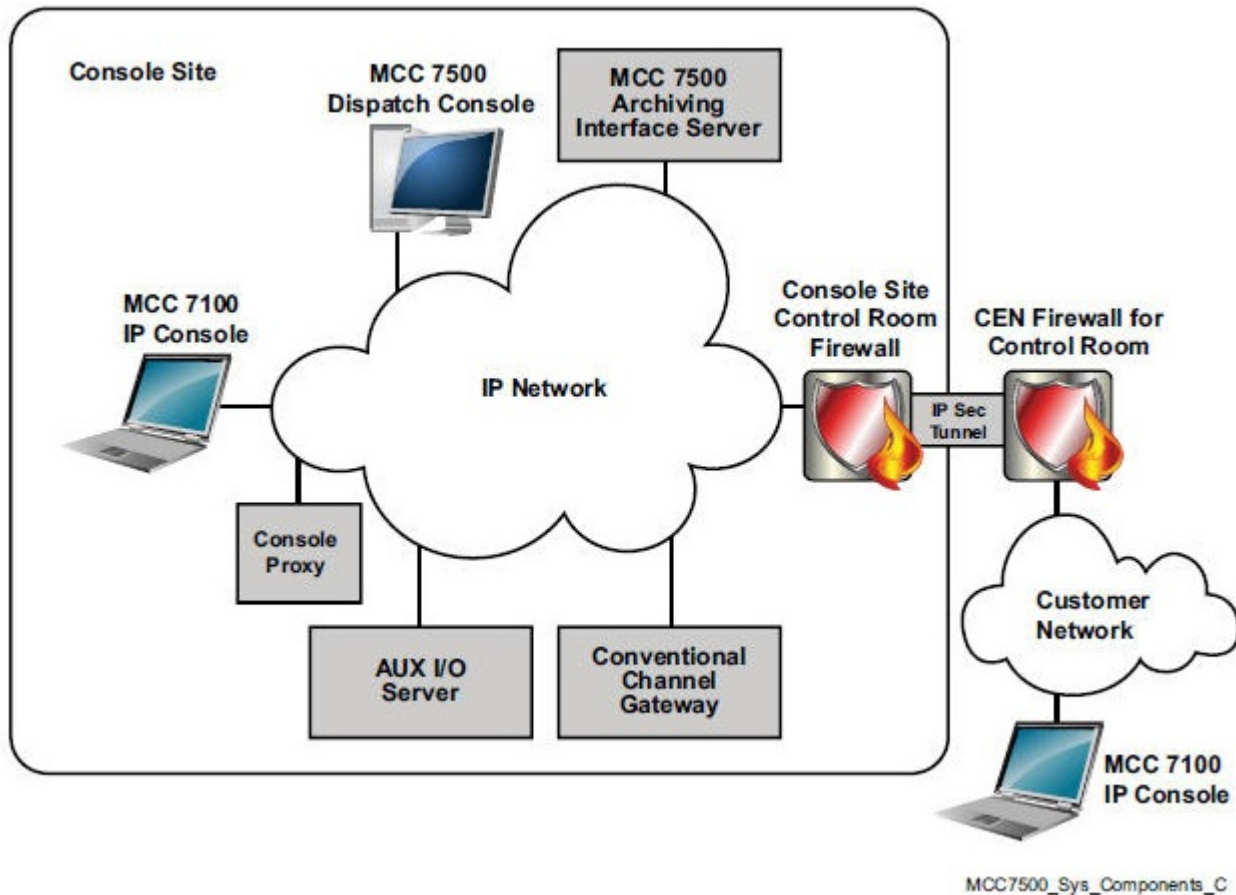
Figure 1: Key Components of Console Sites
