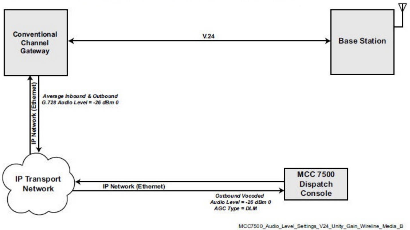
Figure 14: Audio Level Settings for V.24 with Unity-Gain Wireline Media
