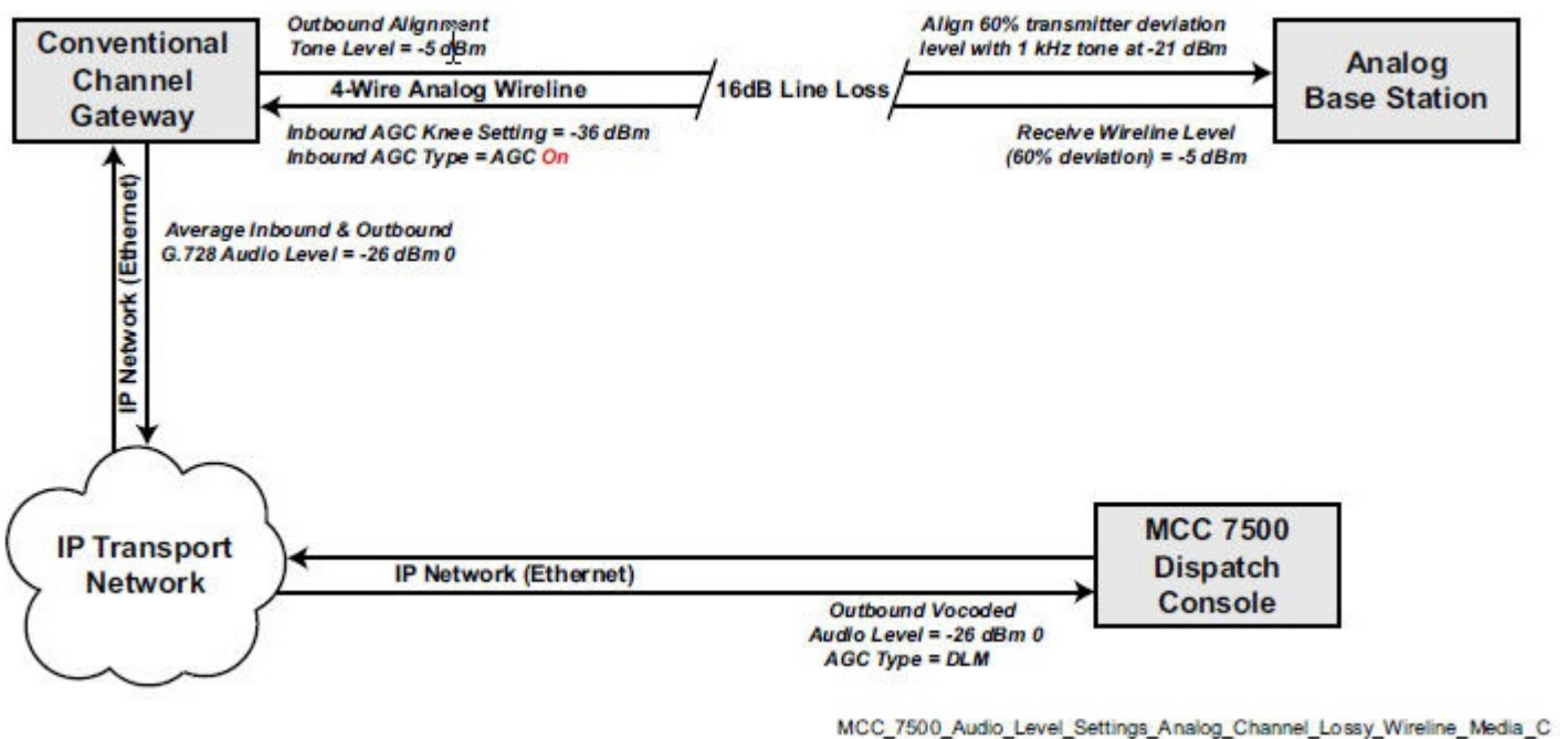
Figure 13: Audio Level Settings for Analog Channel with Lossy Wireline Media
