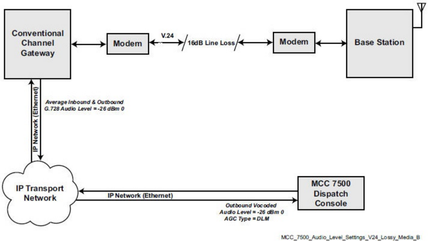
Figure 15: Audio Level Settings for V.24 with Lossy Wireline Media
