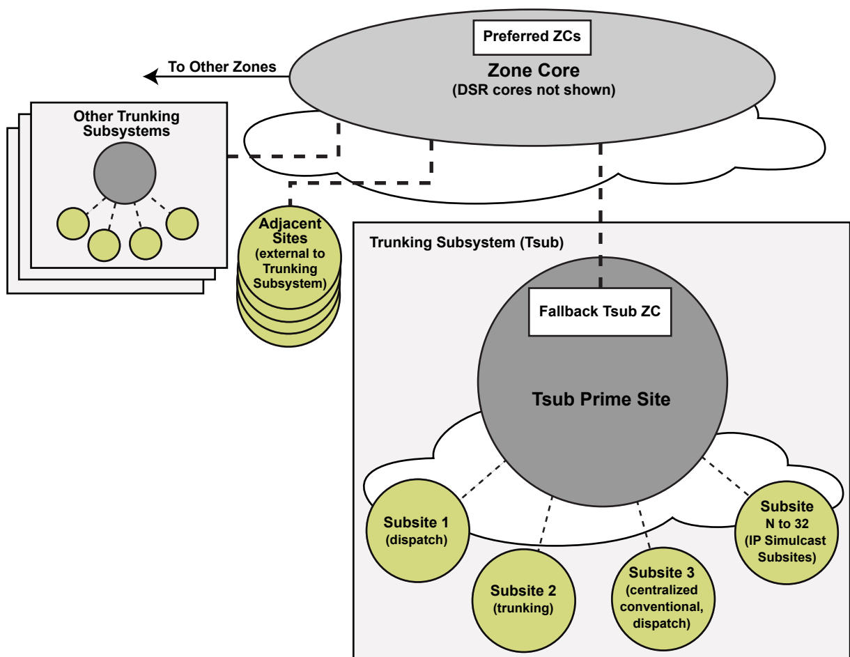
Figure 10: Trunking Subsystem Overview
