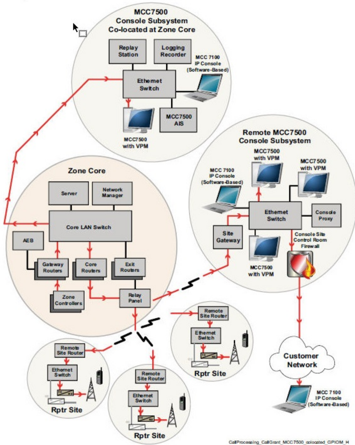
Figure 6: Console Call Grant in a Console Site Colocated at Master Site
