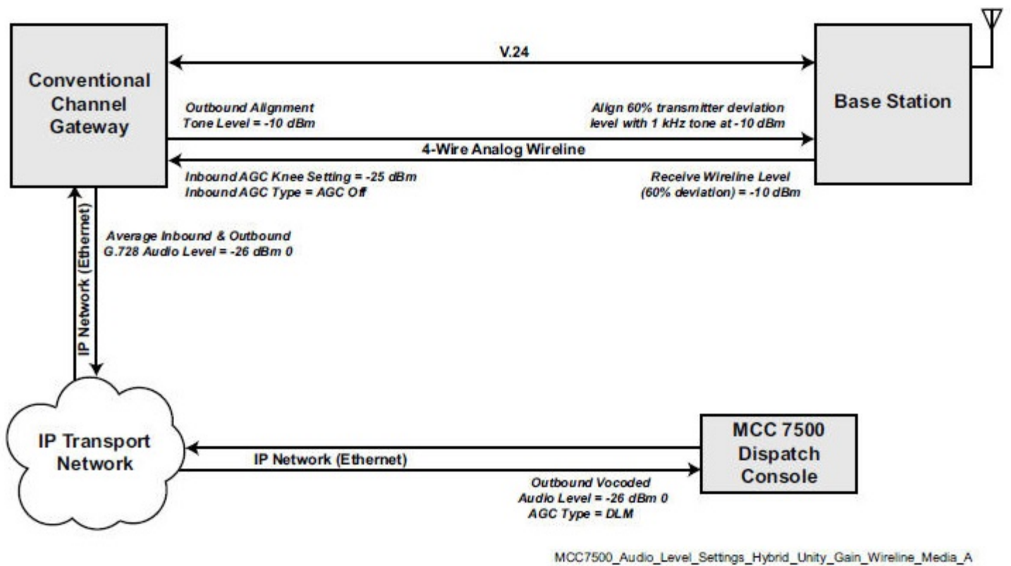
Figure 16: Audio Level Settings for Hybrid Link with Unity-Gain Media
