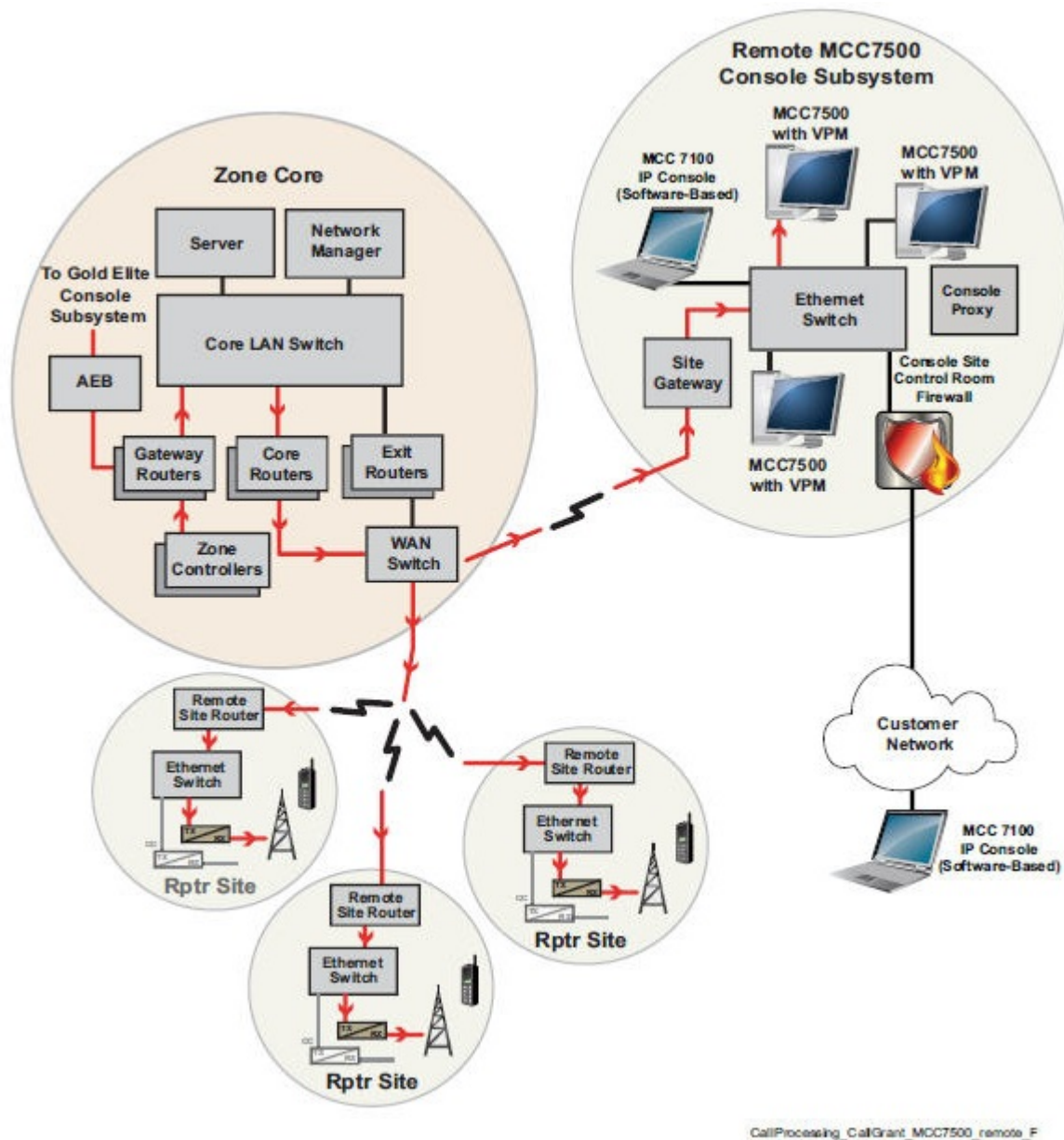
Figure 8: Console Call Grant in a Remote Console Site
