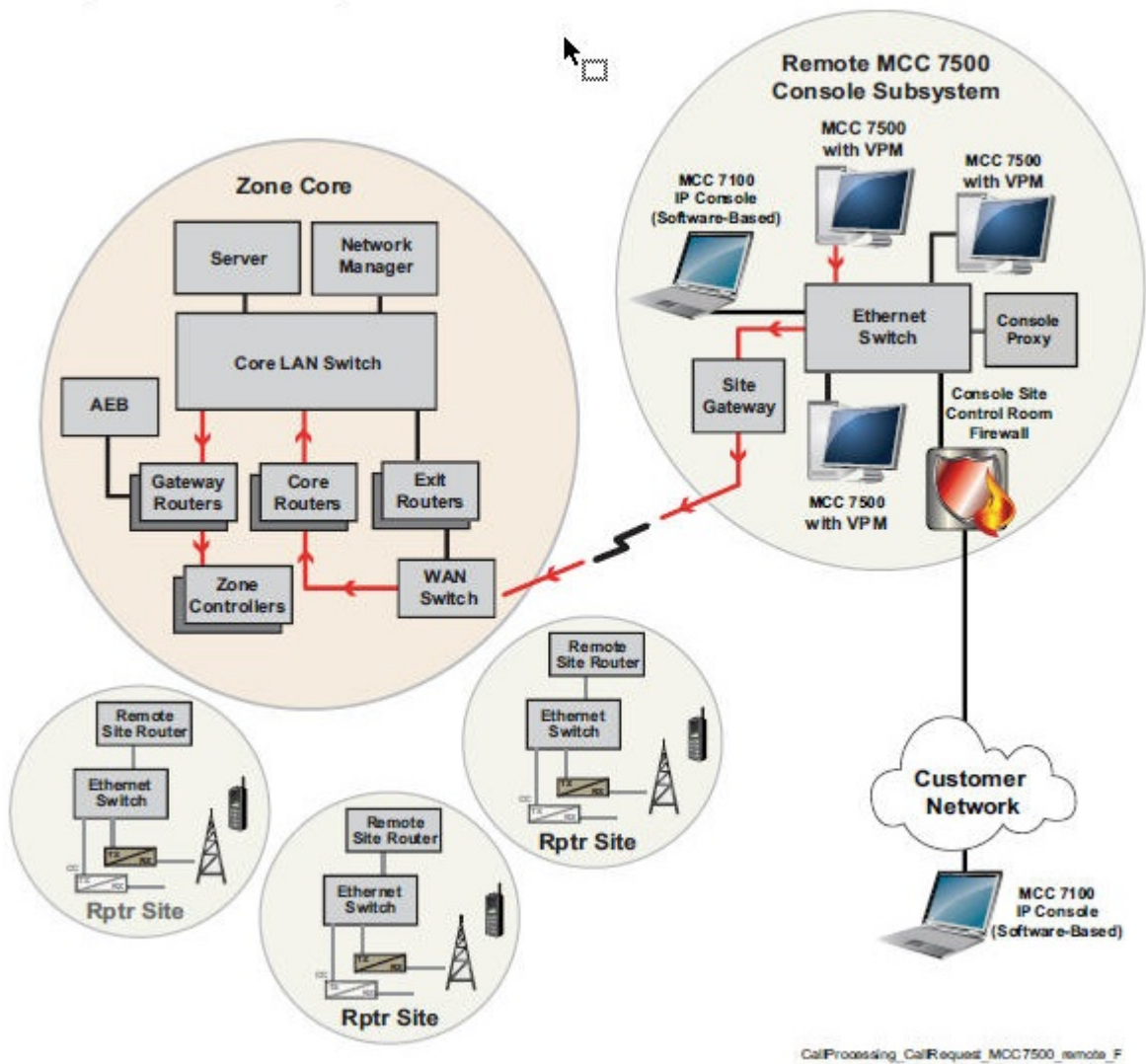
Figure 7: Console Call Request in a Remote Console Site
