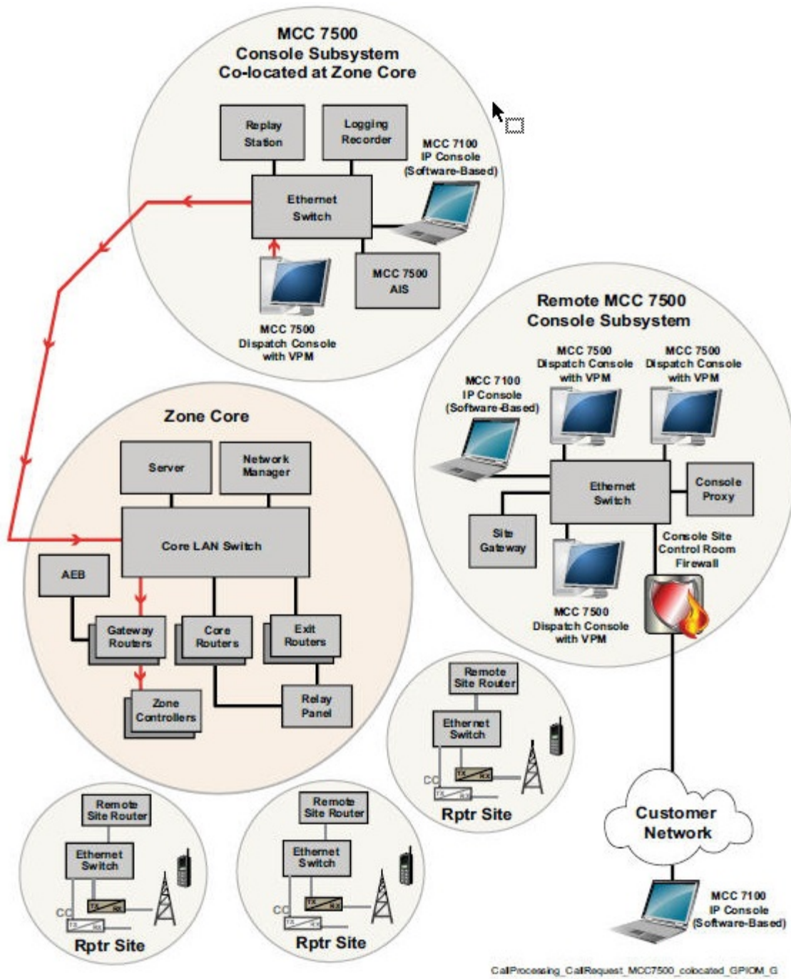
Figure 5: Console Call Request in a Console Site Colocated at Master Site
