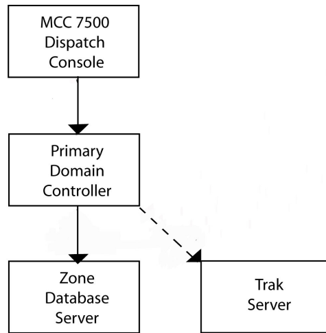
Figure 18: Dispatch Console Time Synchronization
