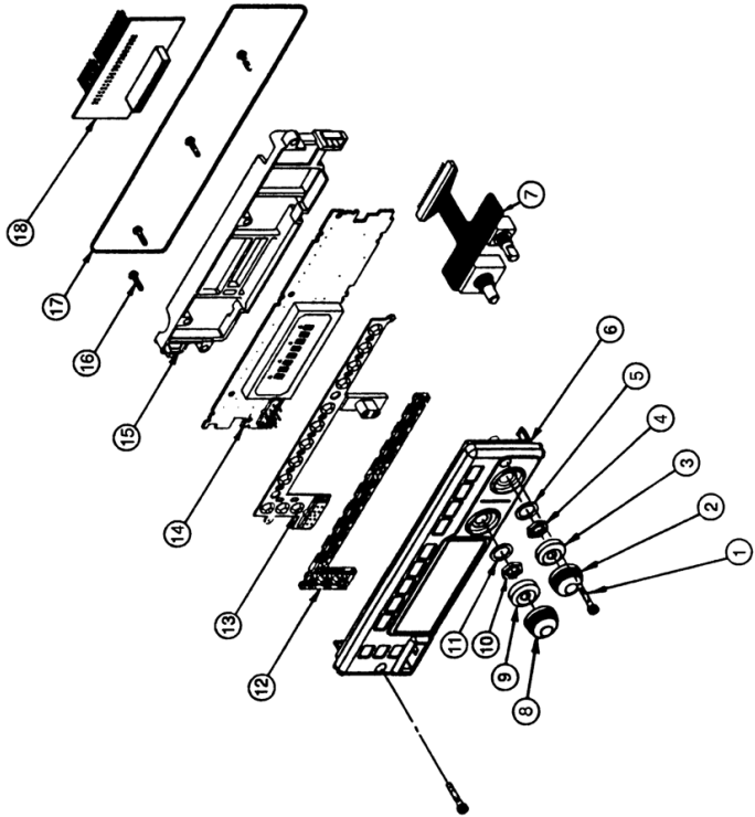
Figure 7-2. W4 Rotary Control Head Exploded View
