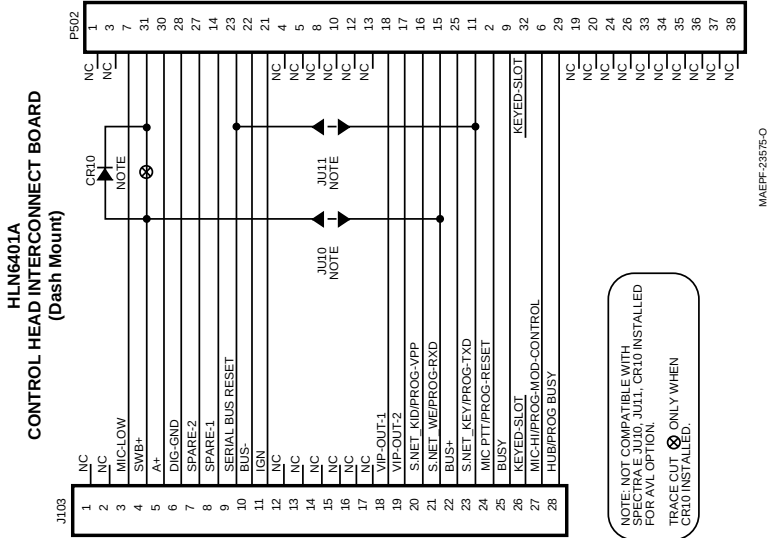
Figure 8-22. HLN6401A Control Head Interconnect Board, (Dash-Mount)
