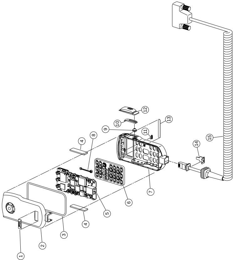
Figure 7-1. W3 Hand-Held Control Head Exploded View
