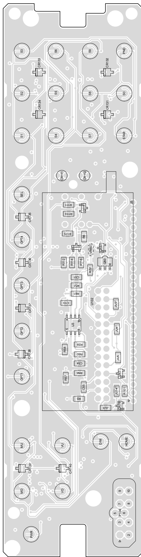
Figure 8-13. HLN6396H_HLN6814C_HLN6563C W5W7 Control Head Component Location Diagram (Viewed from Side 2)
