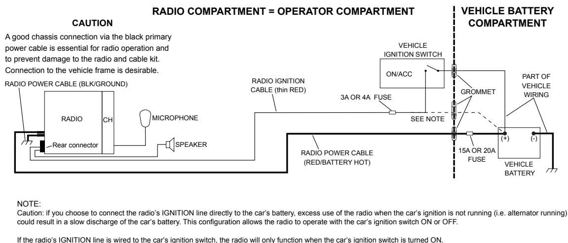
Figure 3-2. Cabling Interconnect Diagram for Dash Mount
