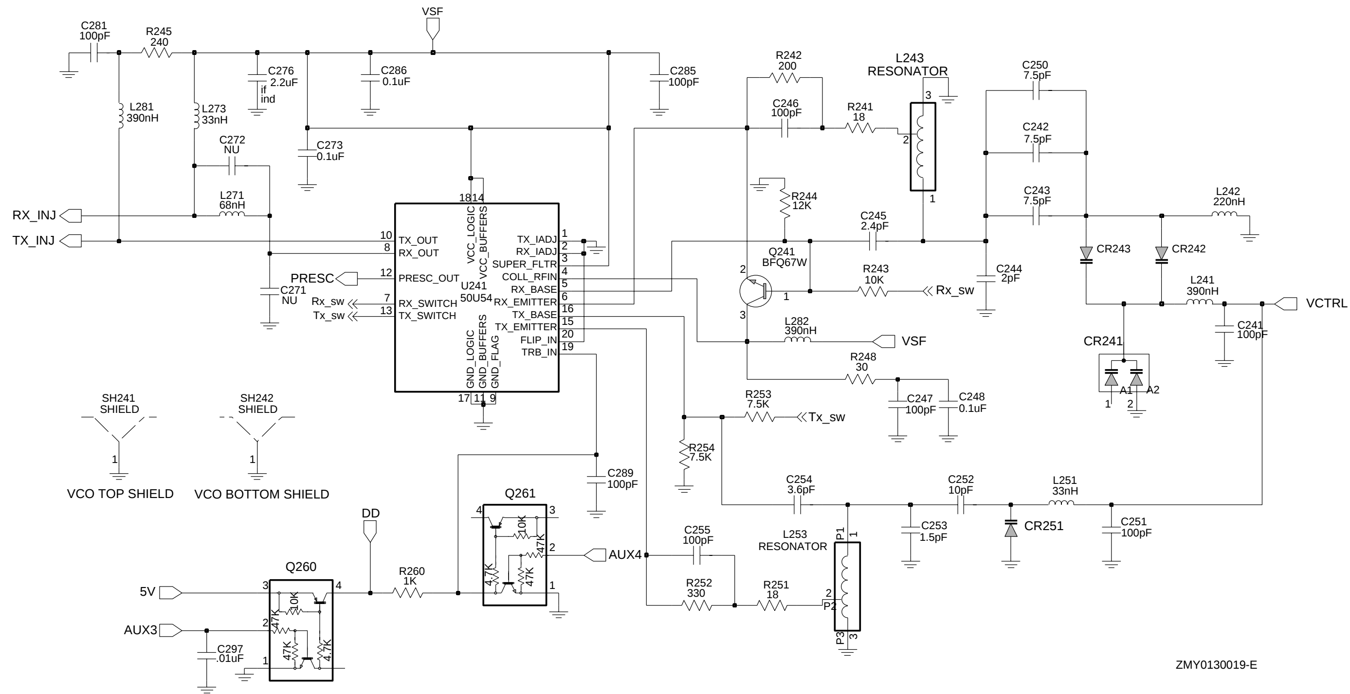
UHF (403-470 MHz) Voltage Controlled Oscillator
