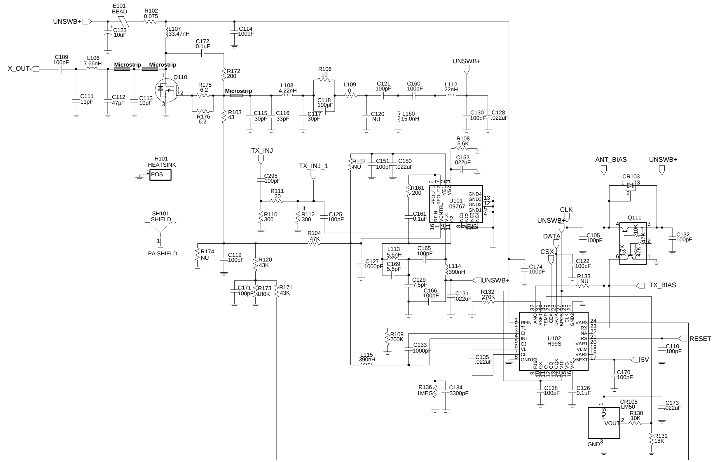
UHF (403-470 MHz) Transmitter
