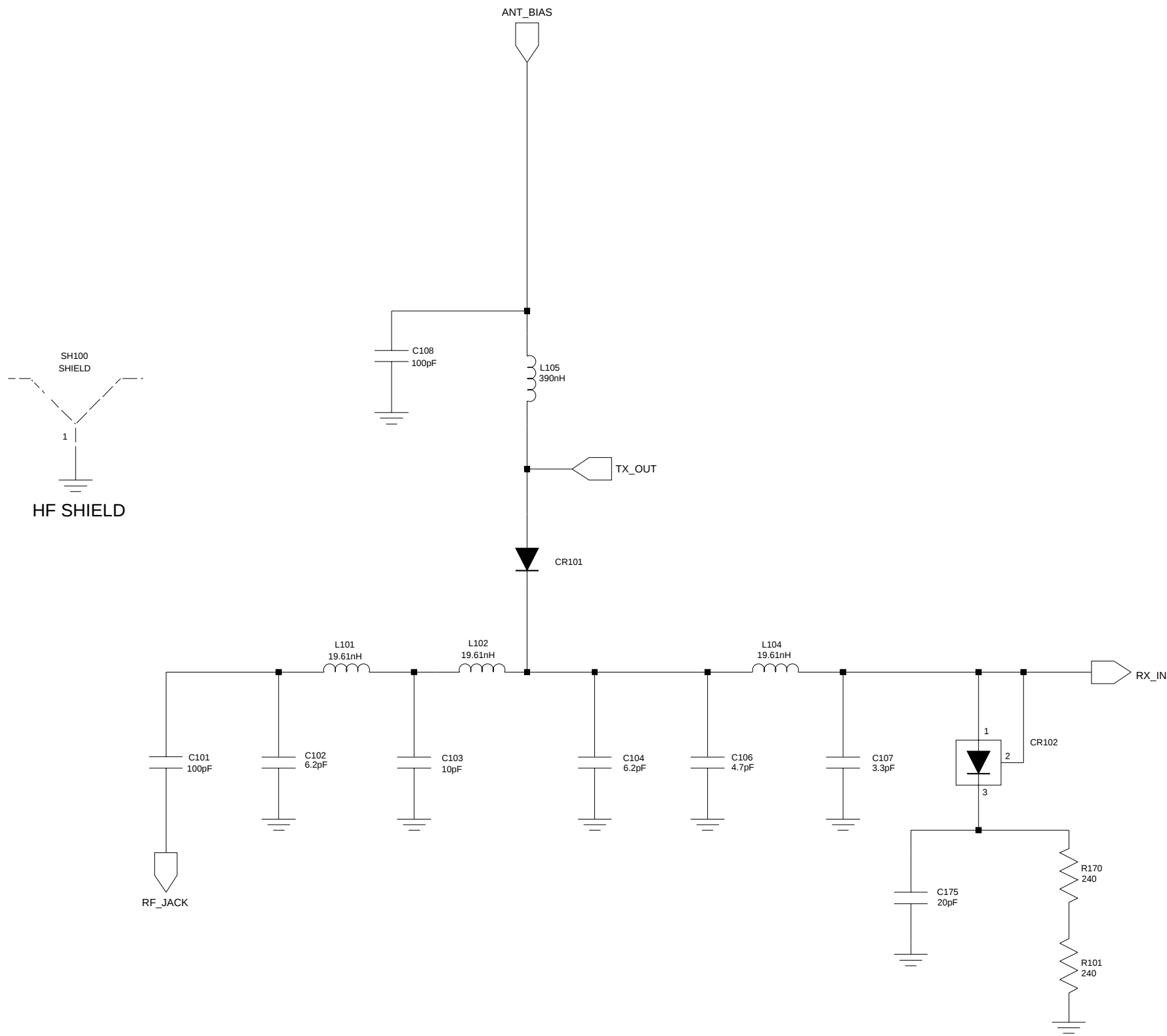
UHF (403-470 MHz) Harmonic Filter
