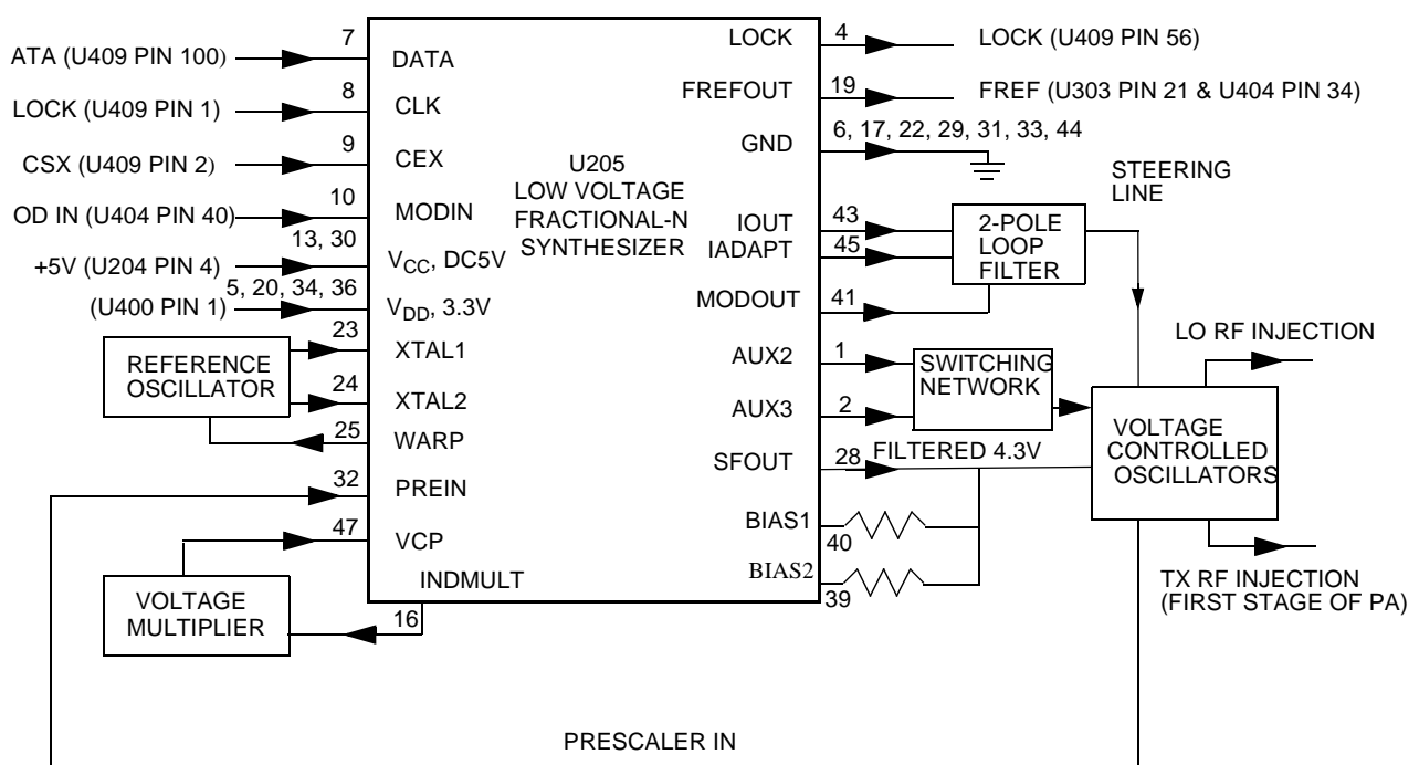
Figure 2-4 Lowband Synthesizer Block Diagram.
