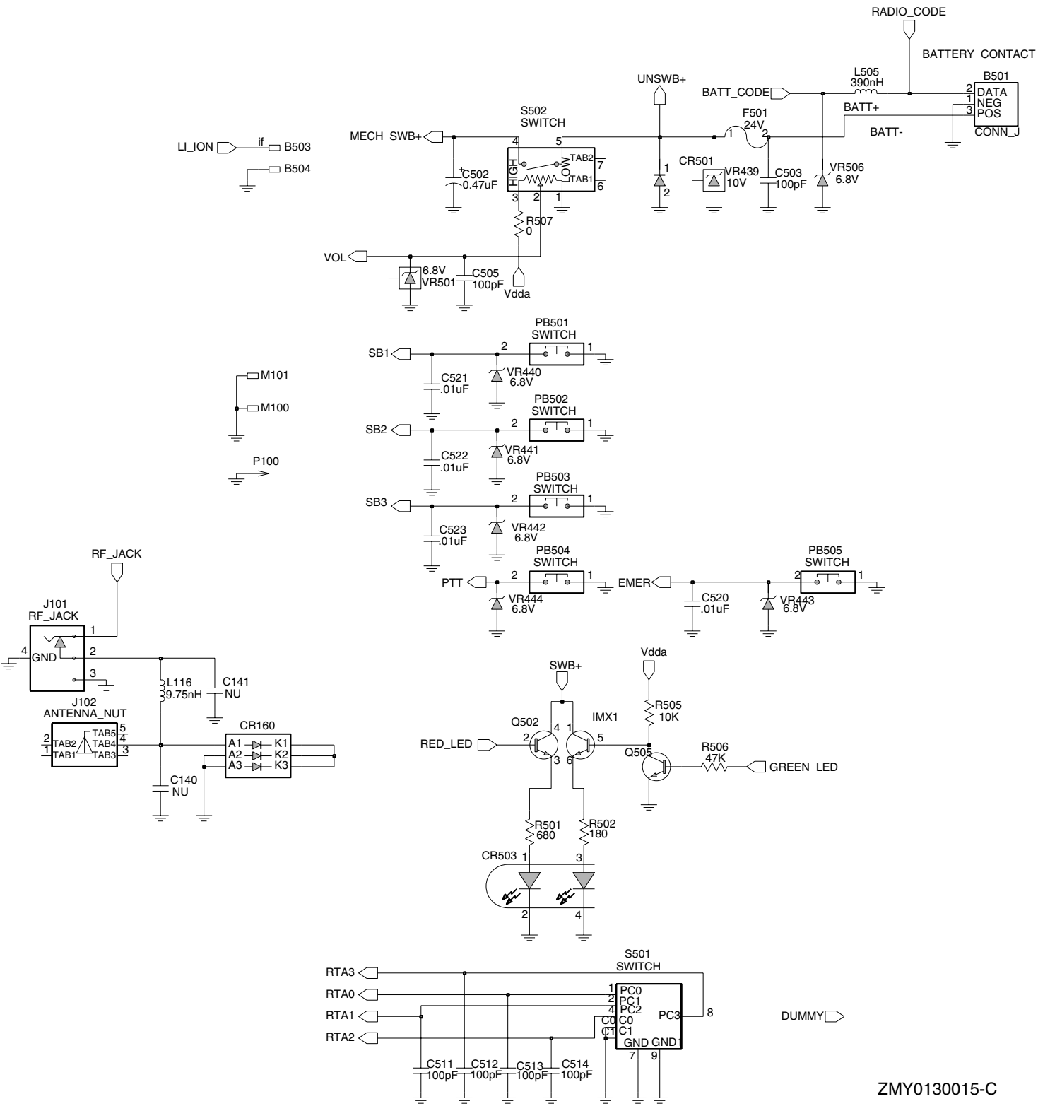
UHF (403-470 MHz) Controls and Switches
