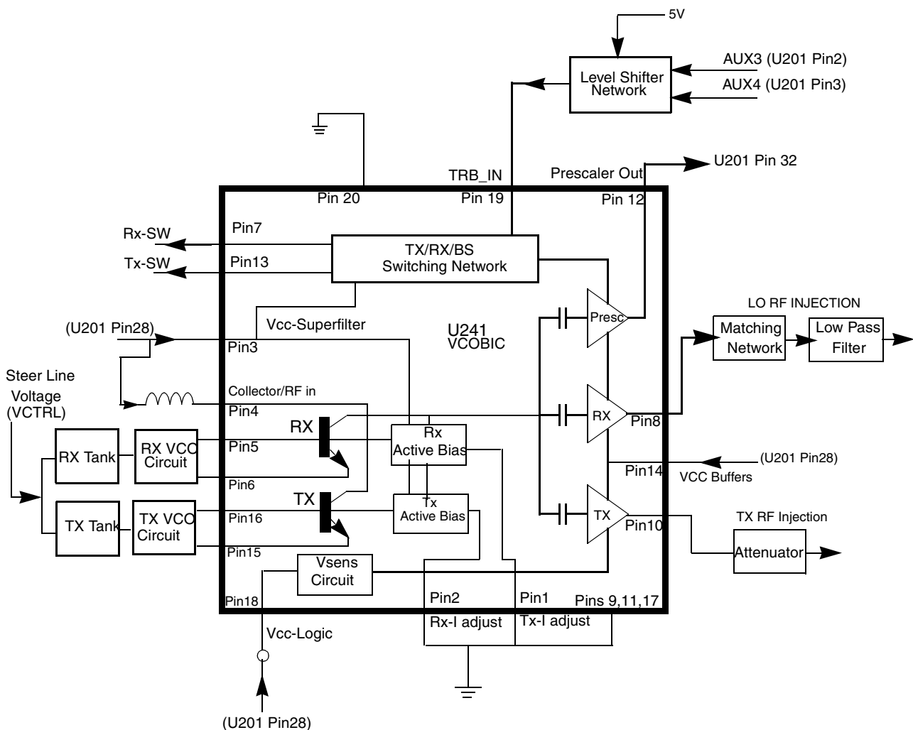
Figure 2-5 UHF VCO Block Diagram
