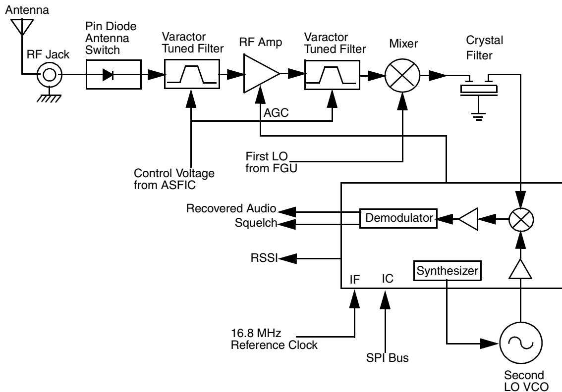
Figure 2-2 UHF Receiver Block Diagram.
