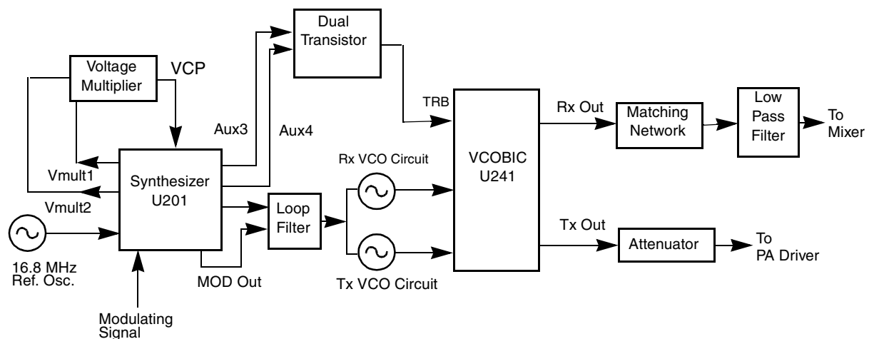
Figure 2-3 UHF Frequency Generation Unit Block Diagram
