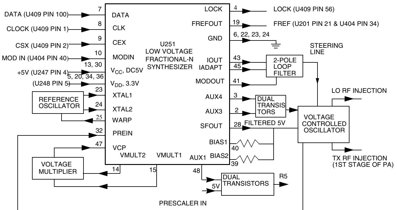
Figure 2-4 UHF Synthesizer Block Diagram
