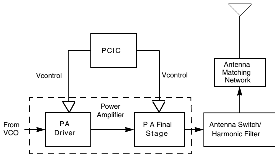
Figure 2-1 UHF Transmitter Block Diagram.
