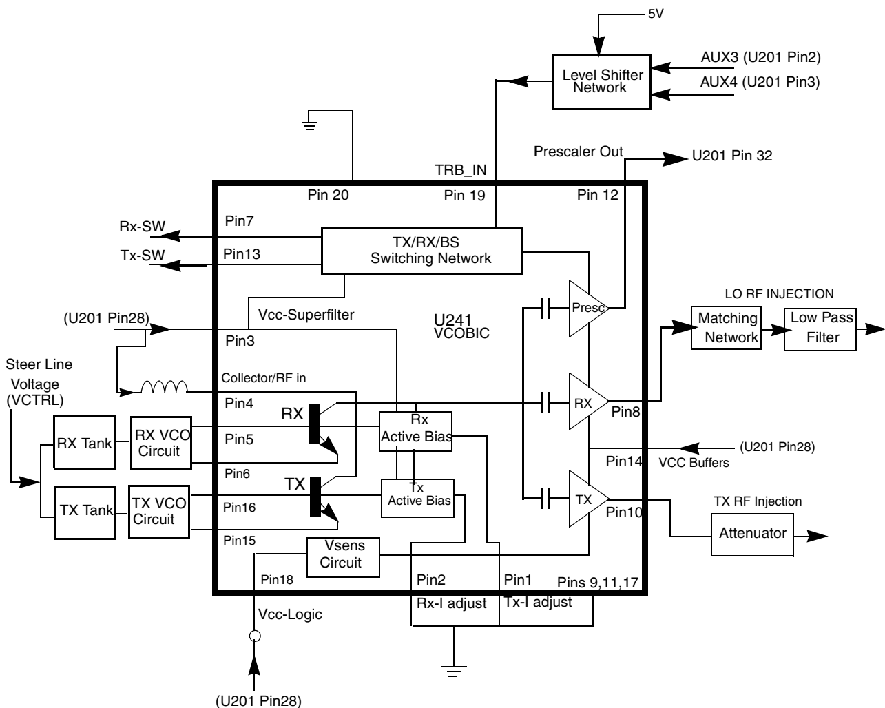
Figure 2-5 UHF2 VCO Block Diagram
