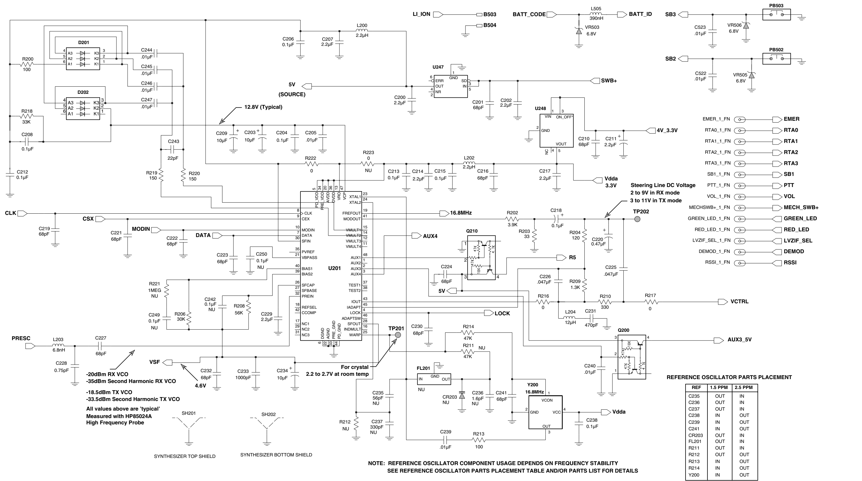
800 MHz (806-870 MHz) Synthesizer
