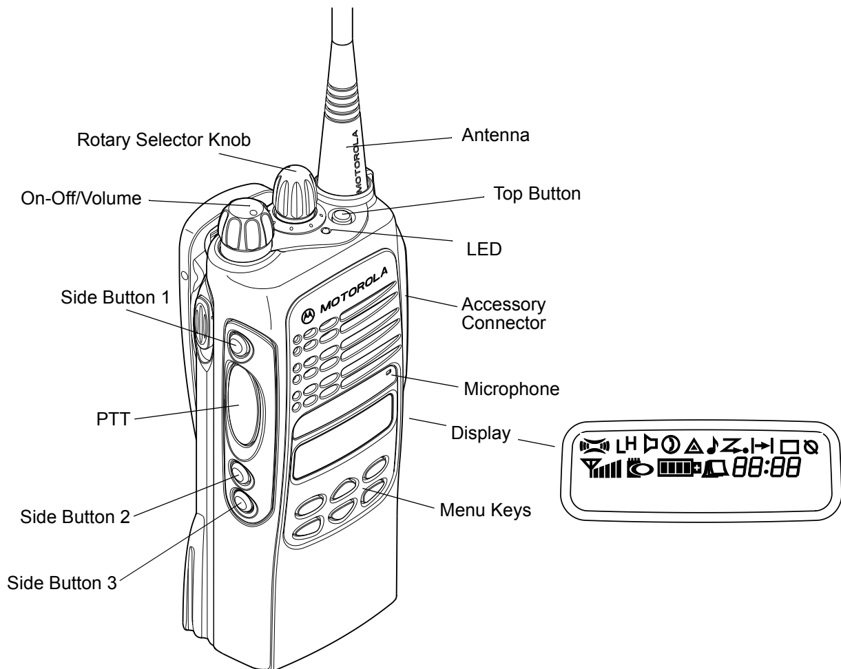
Figure 1-5 GP360 Radio Features
