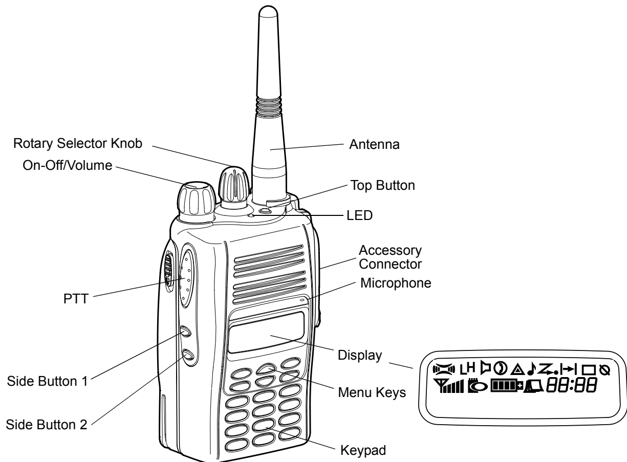
Figure 1-7 GP388 Radio Features
