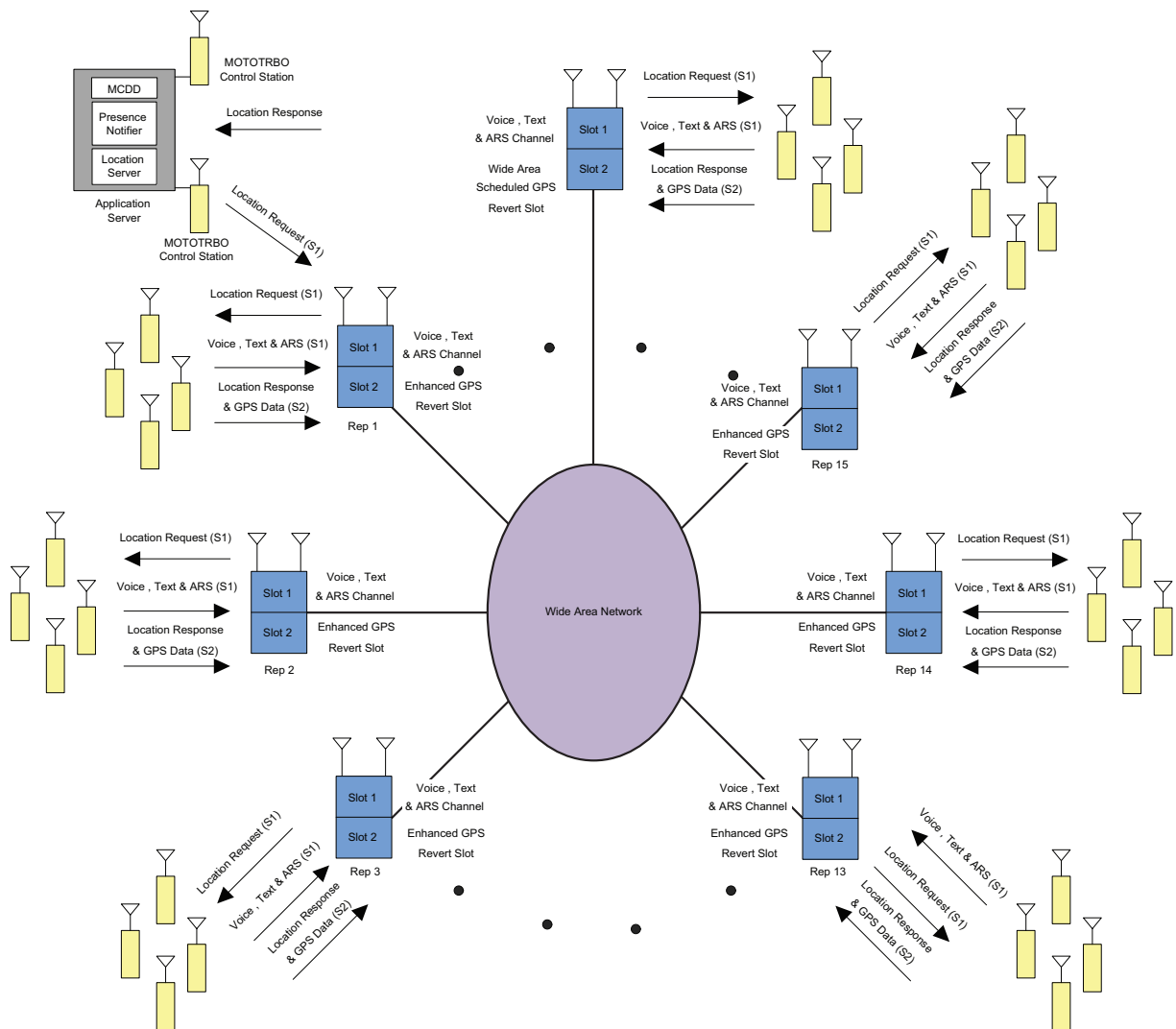
Figure 3-32 IP Site Connect System with an Enhanced GPS Revert Channel
