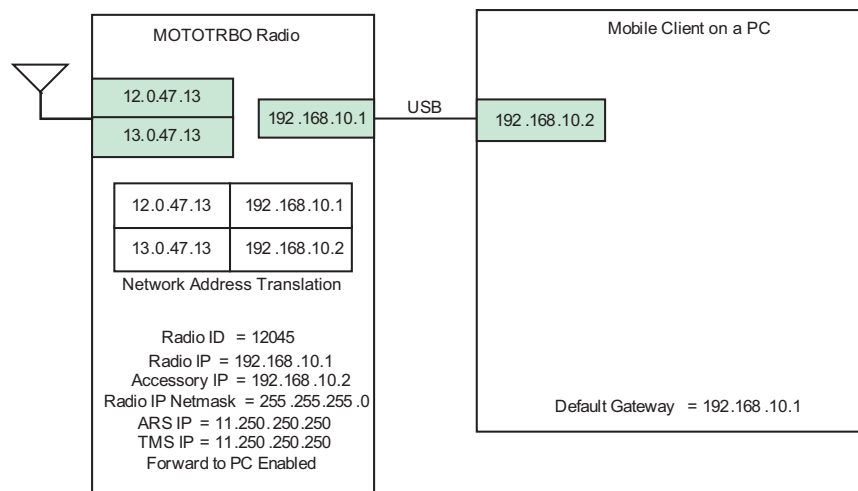
Figure 4-25 Air Interface Network Connectivity
