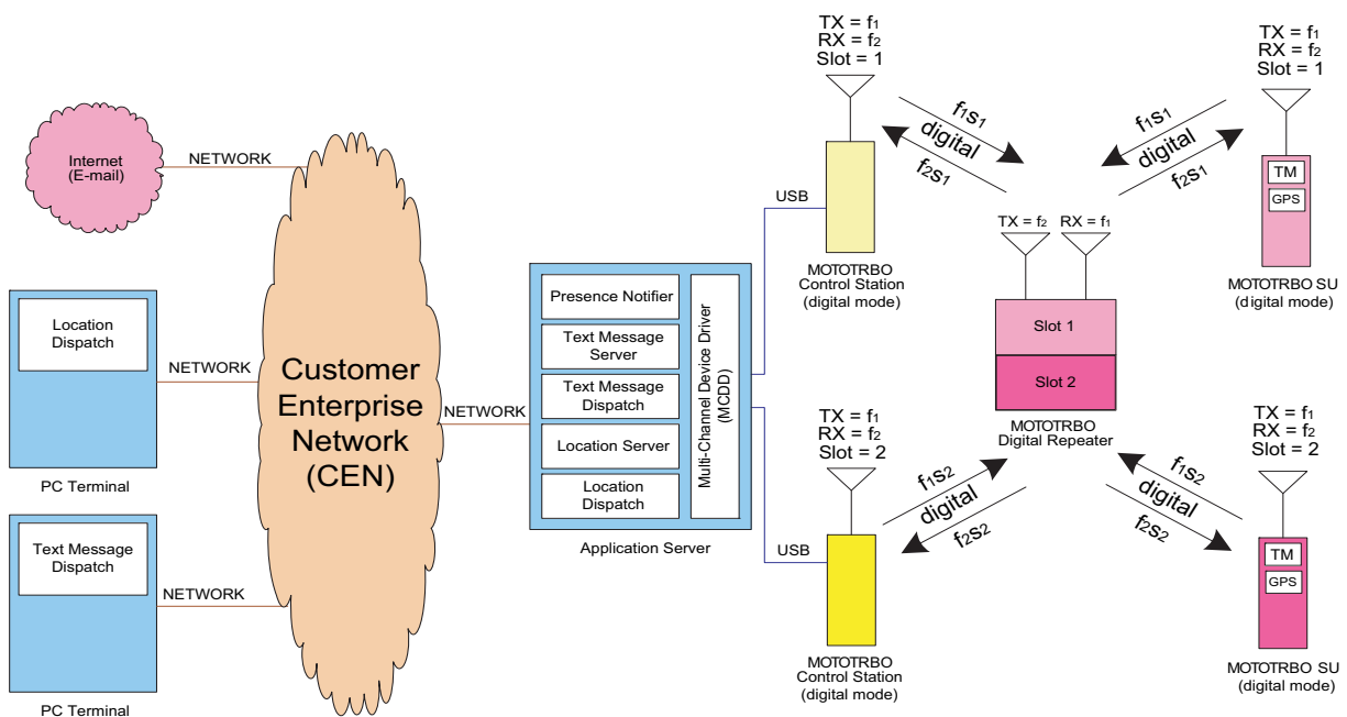
Figure 3-28 MOTOTRBO Radios in Digital Two-Slot Digital Repeater Mode with a Server-Based Configuration Using Control Stations and Remote Dispatchers
