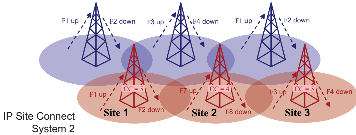
Figure 4-18 Example of Two IP Site Connect Systems with Overlapping Coverage Areas
