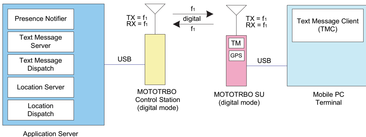
Figure 3-15 MOTOTRBO Radios In Digital Direct Mode with Text Message Server, Location Server and Local Dispatchers
