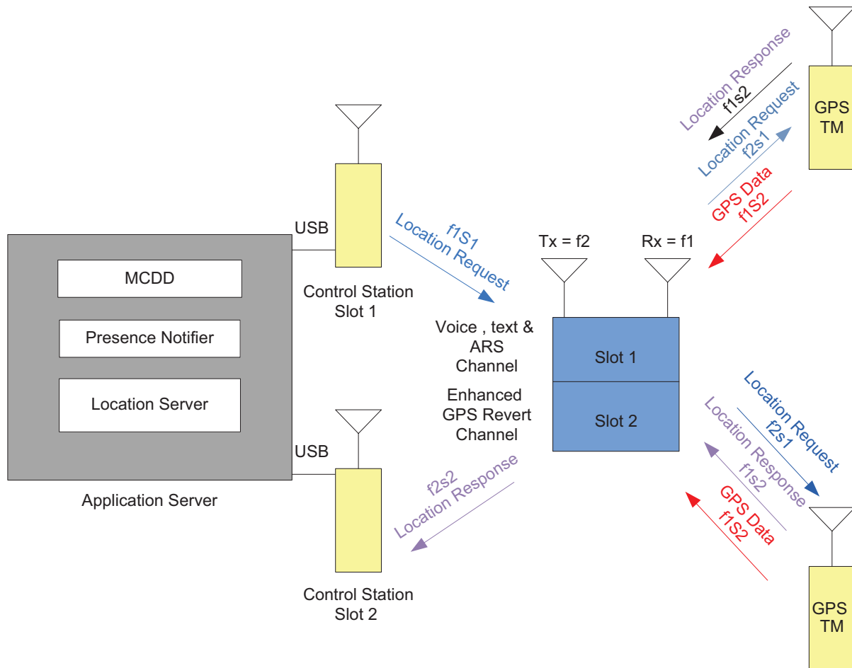
Figure 3-31 Single Site Conventional System with an Enhanced GPS Revert Channel
