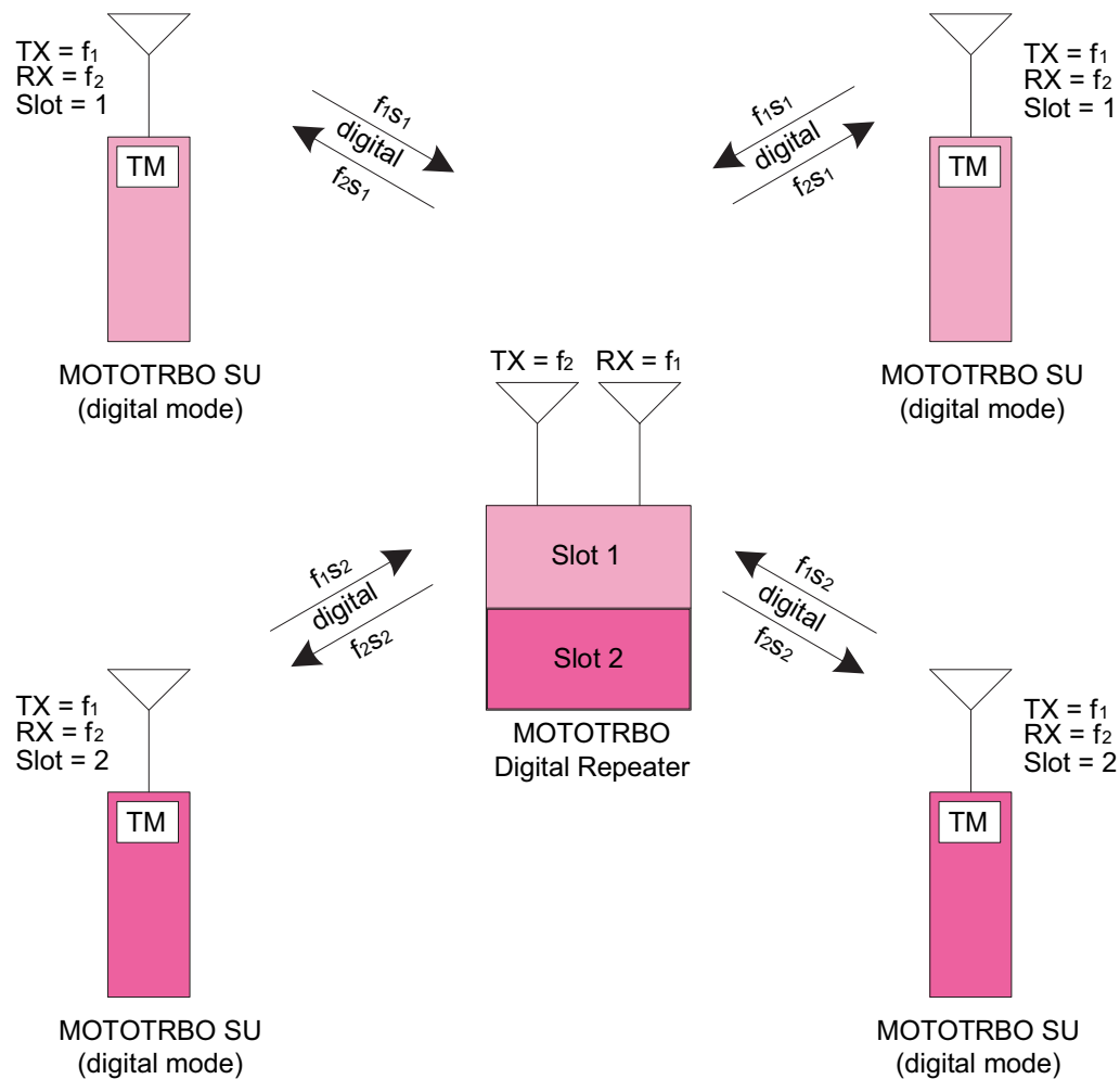
Figure 3-24 MOTOTRBO Radios in Digital Two-Slot Digital Repeater Mode with Built-In Text Messaging
