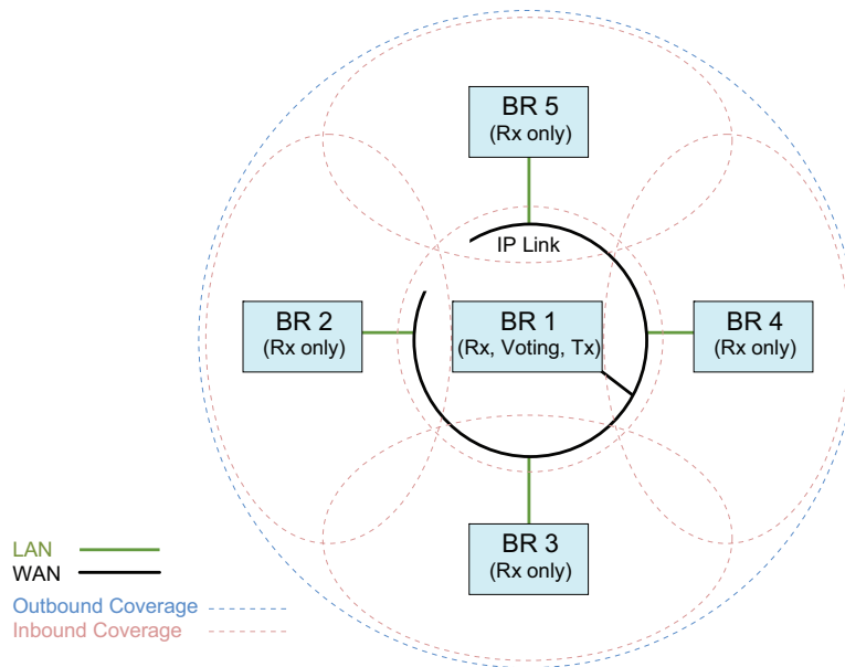
Figure 3-53 Digital Voting Topology for Conventional Single Site or IP Site Connect Local Channel
