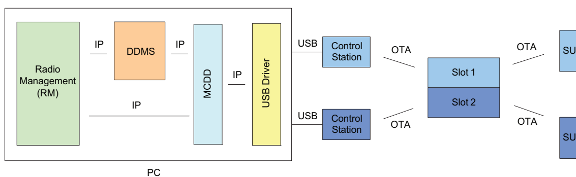
Figure 4-43 Multi-Channel RM Application with Control Stations in Single Site Repeater Mode
