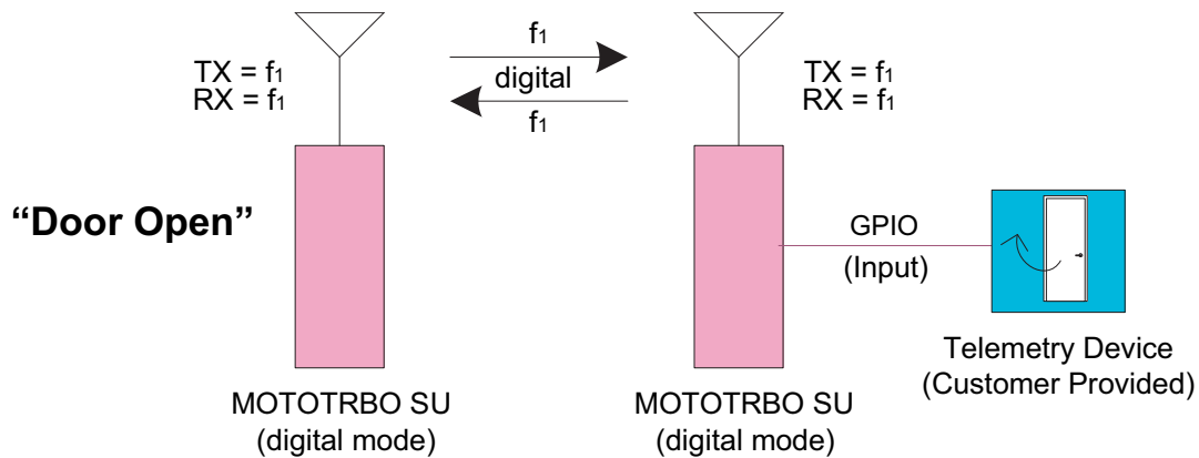
Figure 3-12 Send Telemetry Message from MOTOTRBO Radio to Another MOTOTRBO Radio when Input Pin State Changes
