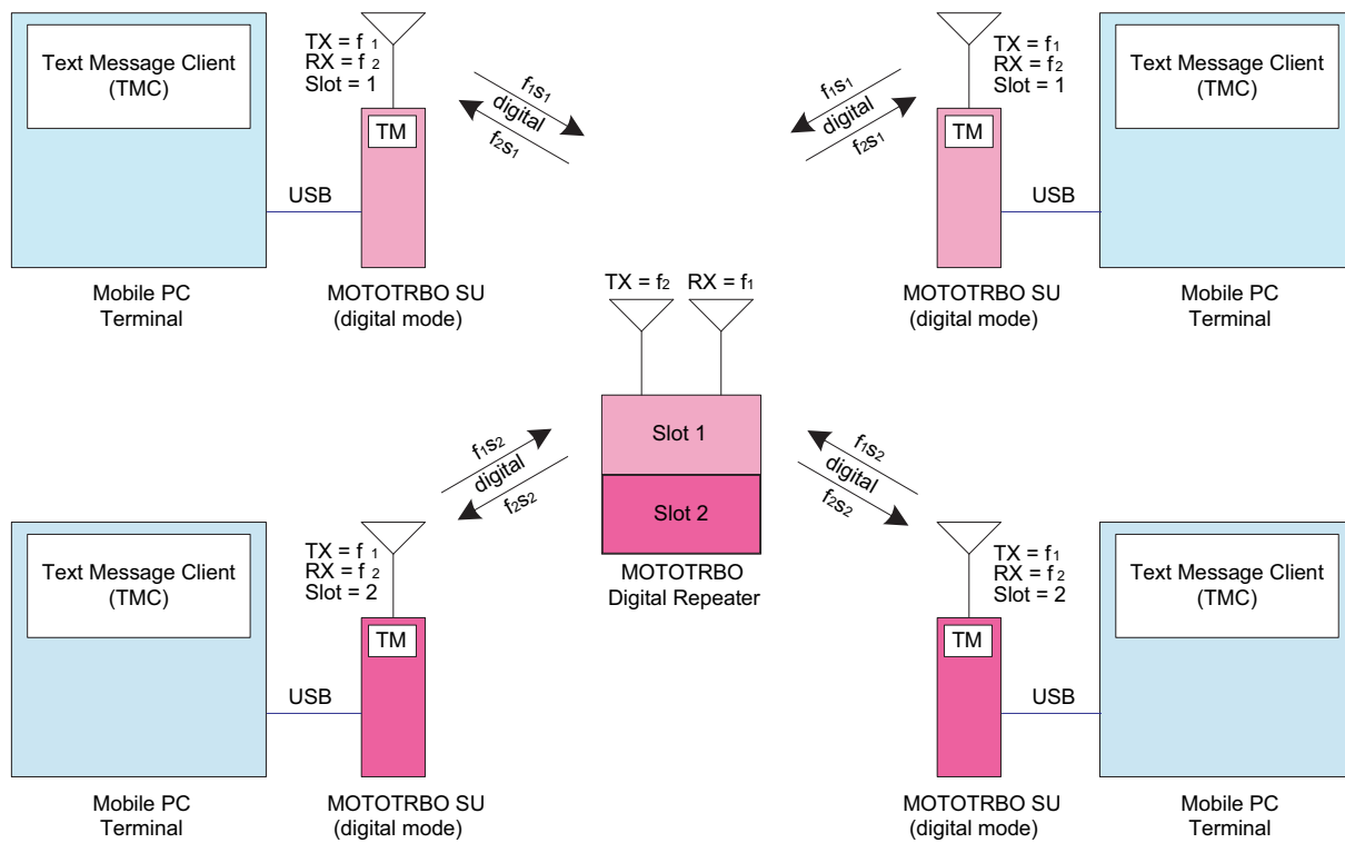
Figure 3-25 MOTOTRBO Radios in Digital Two-Slot Digital Repeater Mode with Text Messaging
