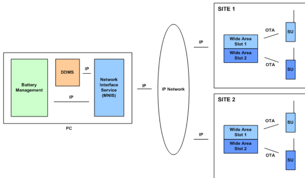
Figure 2-22 BMA Deployment in IP Site Connect with MNIS
