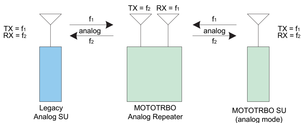
Figure 3-35 MOTOTRBO Analog and Legacy Analog Radios on MOTOTRBO Analog Repeater
