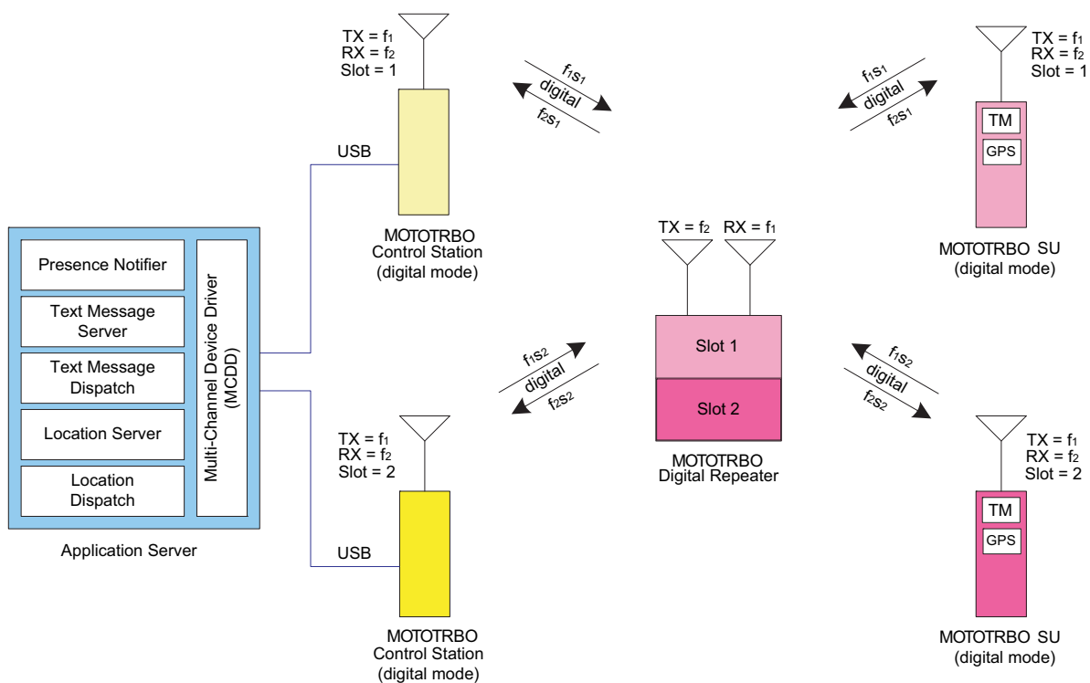
Figure 3-27 MOTOTRBO Radios in Digital Two-Slot Digital Repeater Mode with a Server-Based Configuration Using Control Stations
