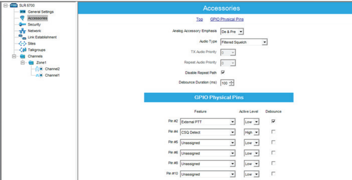
Figure 2-61 CPS Configuration for TSCC03 Channel Controller (1 of 2)
