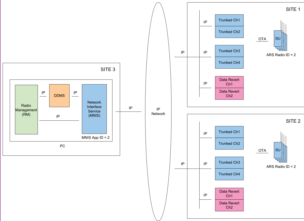
Figure 4-63 RM Application with MNIS in a Linked Capacity Plus System with Presence and Wide or Local Area Data Revert Channels
