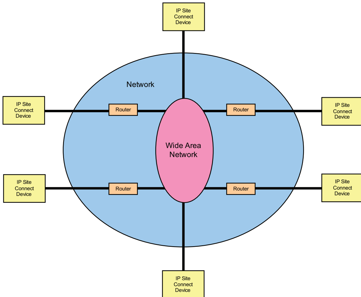
Figure 3-41 IP Site Connect Devices connected through Wide Area Network
