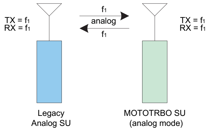
Figure 3-19 Legacy Analog Radios and MOTOTRBO Radios (in analog mode) in Direct Mode
