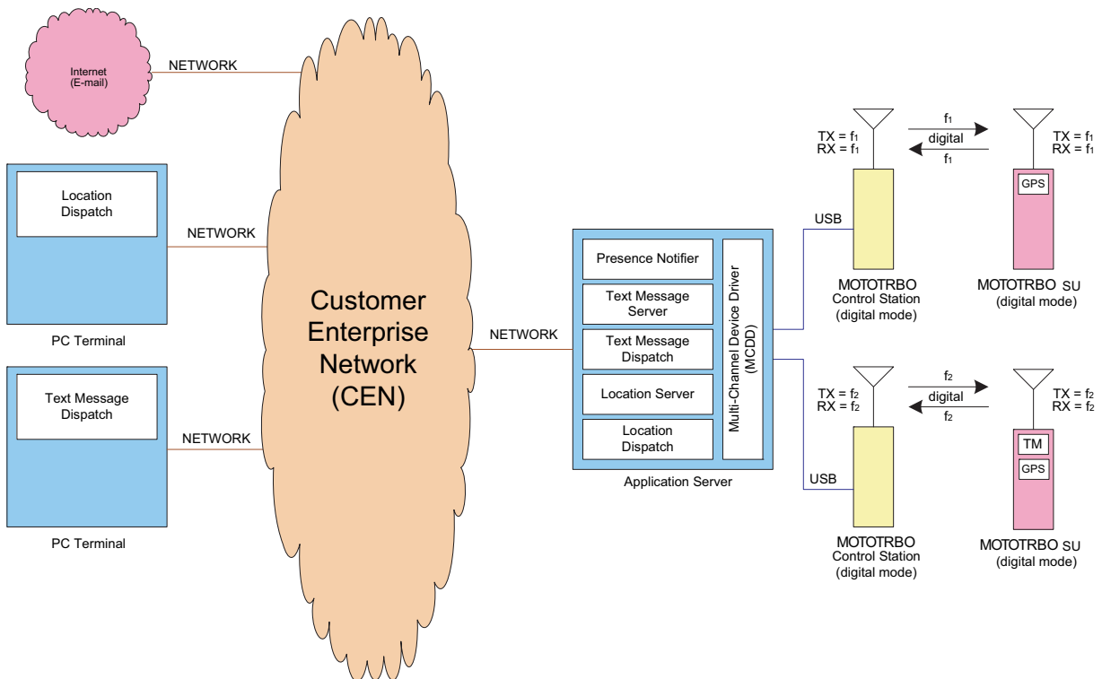
Figure 3-17 MOTOTRBO Radios in Two Channel Digital Direct Mode Server-Based Configuration with Remote Dispatchers
