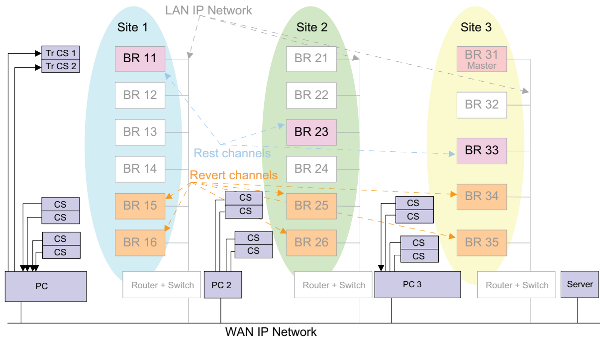
Figure 3-51 A Linked Capacity Plus System with Data over Local Revert Channels
