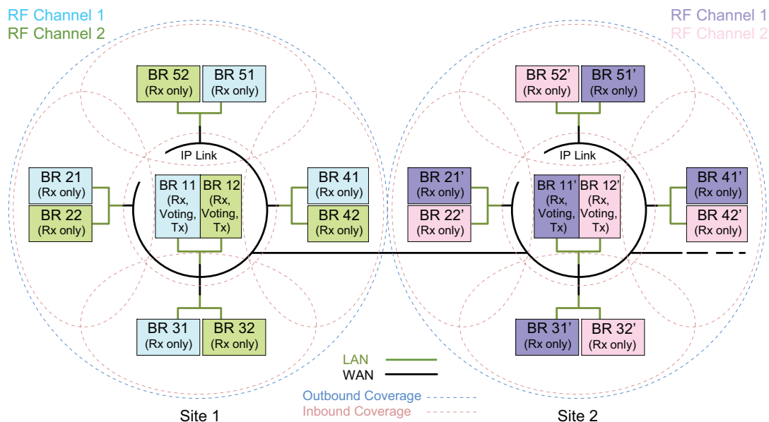
Figure 3-56 Digital Voting Topology for a Two-Site Linked Capacity Plus System
