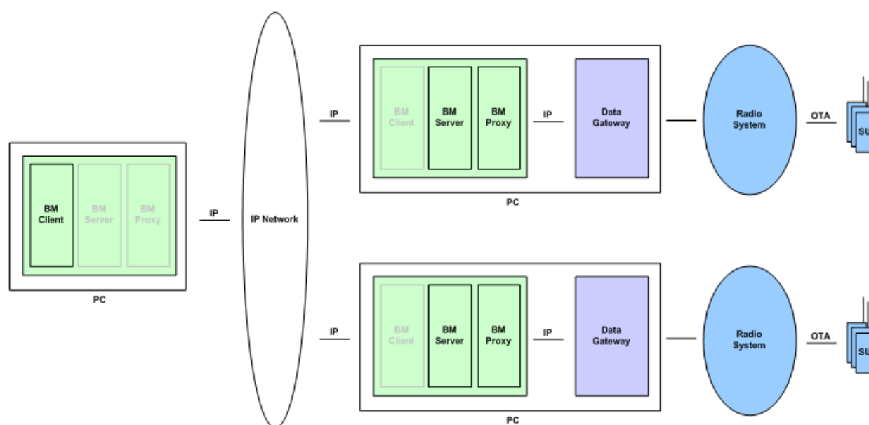
Figure 2-34 BMA Deployment with Client Remote from Multiple Server and Proxies
