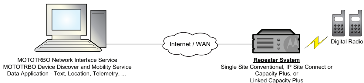
Figure 3-3 MOTOTRBO Network Interface Service (MNIS)
