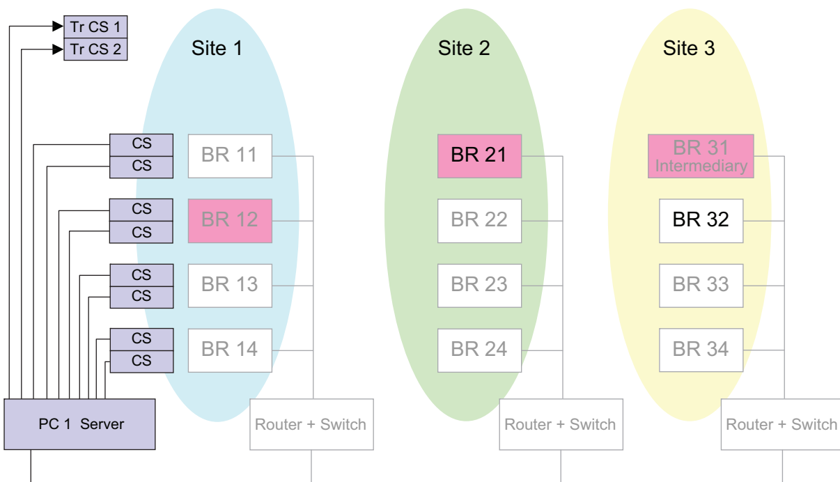
Figure 3-50 A Linked Capacity Plus System with Data over Trunked Channels
