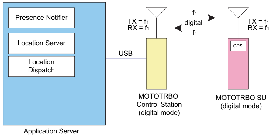
Figure 3-14 MOTOTRBO Radios In Digital Direct Mode/Dual Capacity Direct Mode with Location Server and Local Location Client
