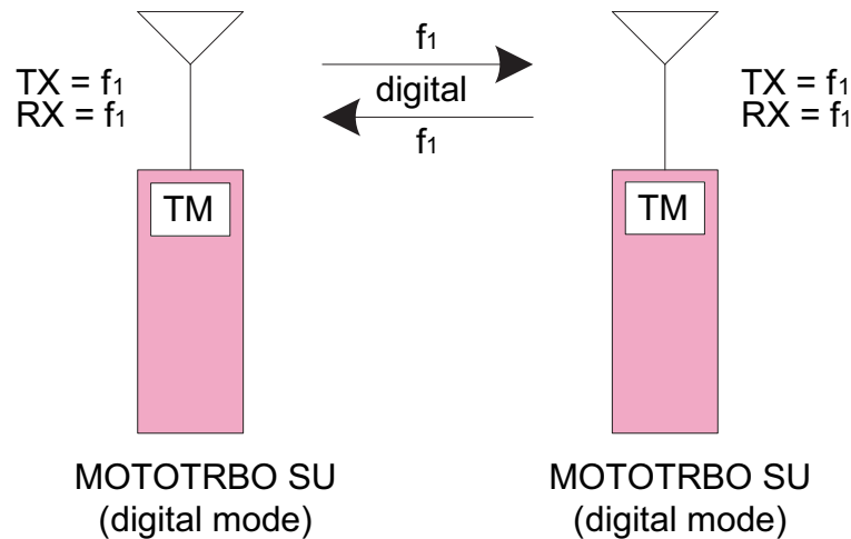
Figure 3-9 MOTOTRBO Radios (in digital mode) Text Messaging In Direct Mode/Dual Capacity Direct Mode
