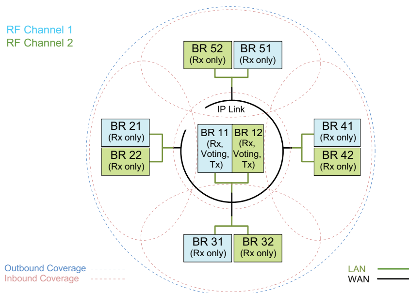
Figure 3-55 Digital Voting Topology for a Capacity Plus System
