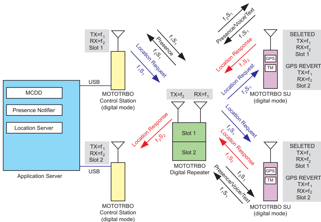
Figure 3-30 MOTOTRBO Radios in Two-Slot Digital Repeater Mode with GPS Revert Configuration
