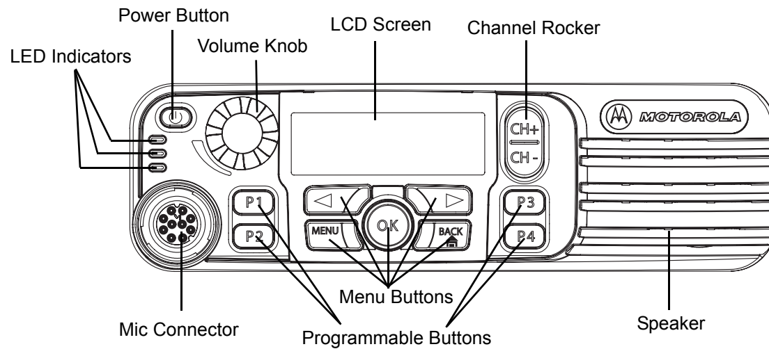
Figure 3-6 MOTOTRBO Mobile Control Head (Full Display Model)
