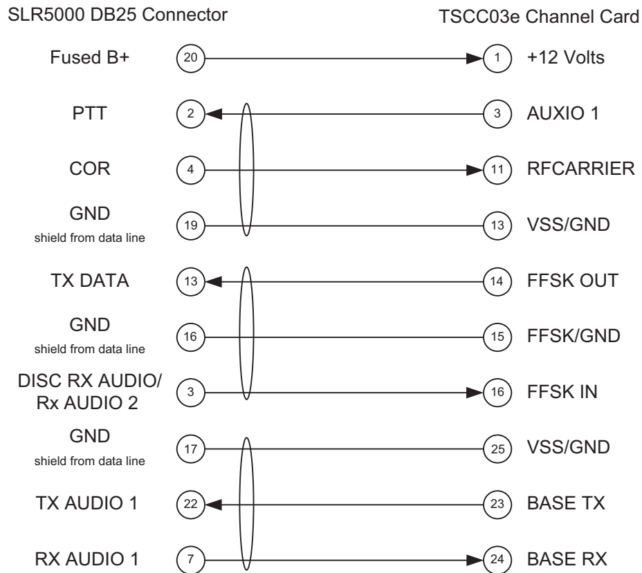
Figure 2-60 Hardware Connections between SLR 5000 and TSCC03 Channel Controller
