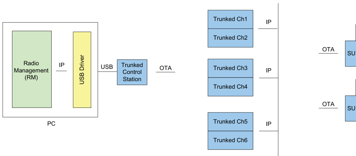
Figure 4-53 RM Application in a Capacity Plus System with No DDMS and One Trunked Control Station
