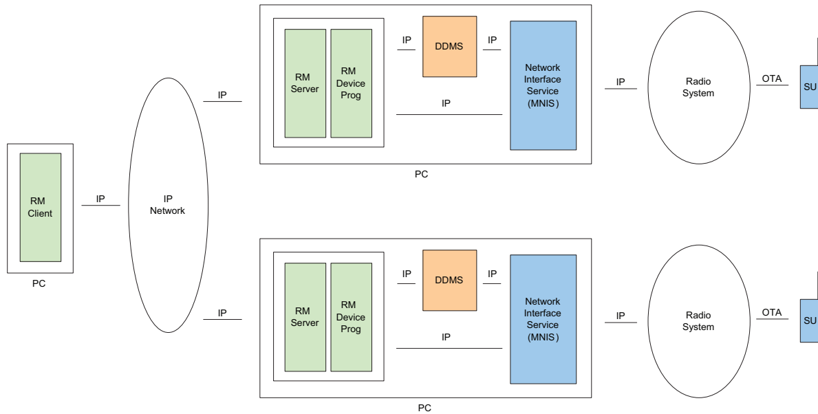
Figure 2-44 Remote RM Client with Multiple RM Servers with MNIS
