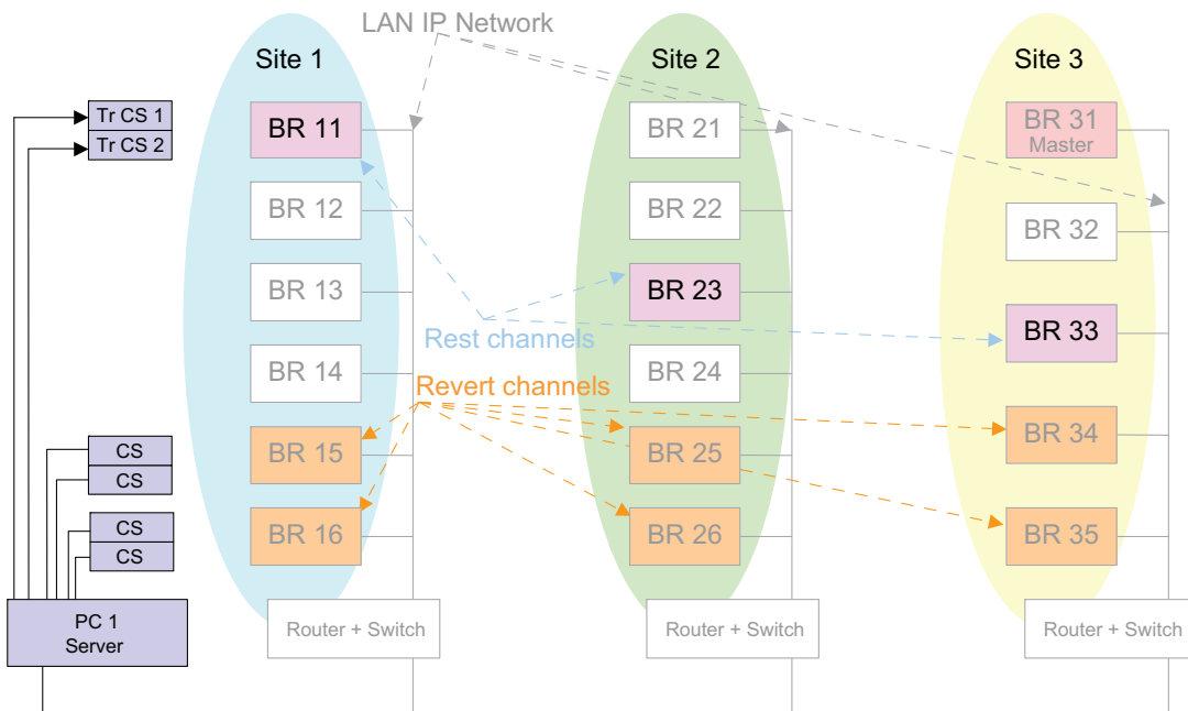
Figure 3-52 A Linked Capacity Plus System with Data over Wide Area Revert Channels
