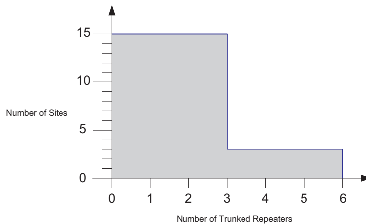
Figure 4-23 Valid Combinations of Sites and Trunked Repeaters for Linked Capacity Plus
