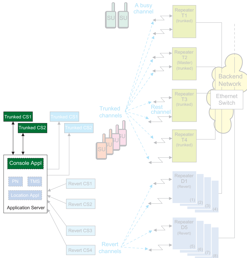
Figure 3-49 Capacity Plus Devices with a Dispatch Station (Console)
