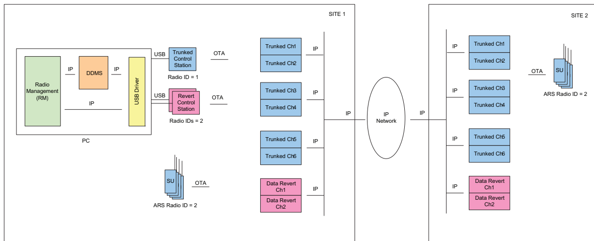
Figure 4-61 RM Application with Control Stations in a Linked Capacity Plus System with Presence (DDMS) and Wide Area Data Revert Channels
