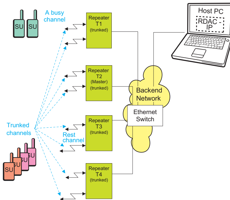
Figure 3-43 Capacity Plus Devices with Local RDAC and no Data Application Server
