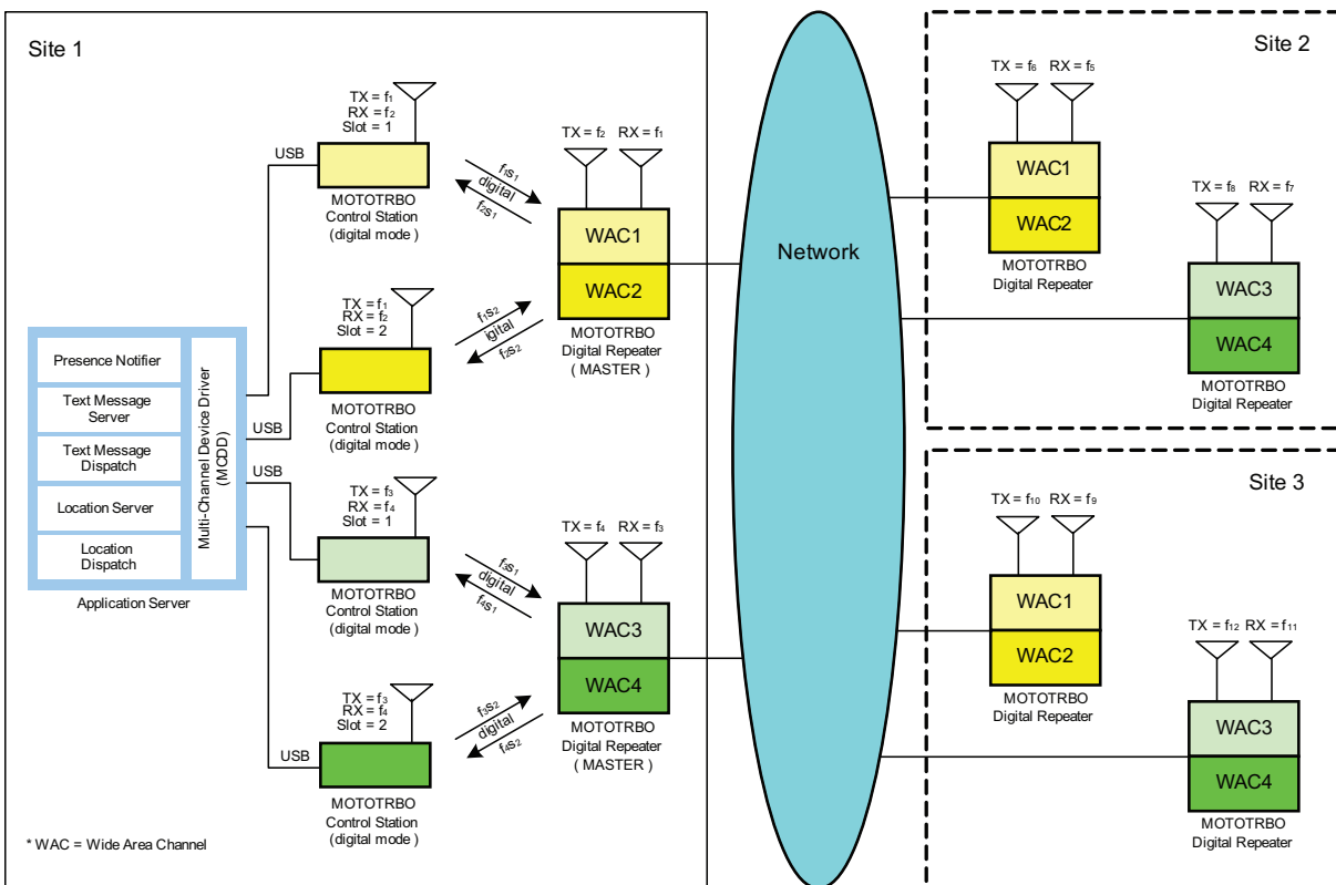
Figure 3-39 Multiple Wide Area Systems with Centralized Data Application Server
