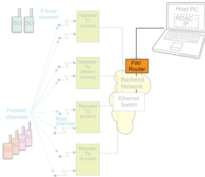
Figure 3-45 Capacity Plus Devices with Remote RDAC and no Data Application Server
