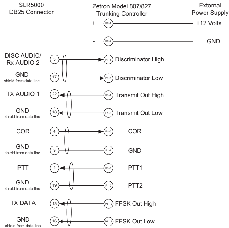
Figure 2-57 Hardware Connections between SLR 5000 and M827/M807 Controller
