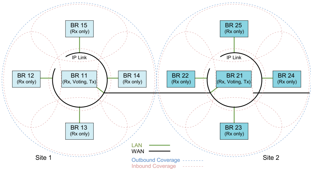
Figure 3-54 Digital Voting Topology for a Two-Site IP Site Connect System
