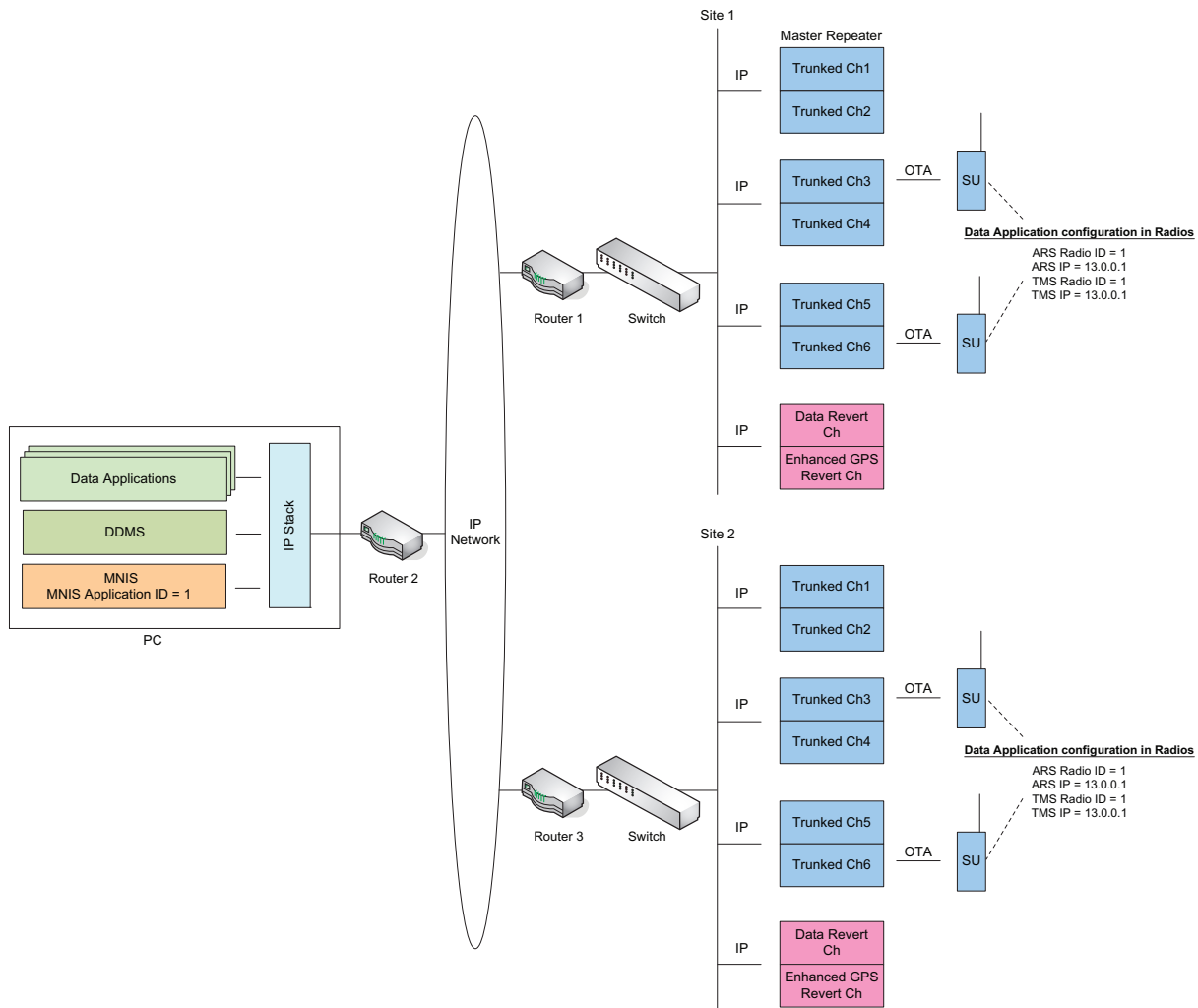
Figure 4-34 Linked Capacity Plus System with MNIS
