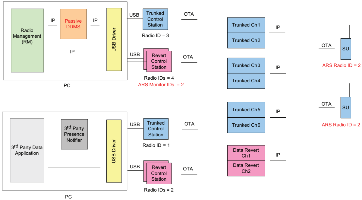
Figure 4-65 RM Application with Control Stations and Passive Presence Configuration with Third-Party Data Application on a Capacity Plus Data Revert Configuration
