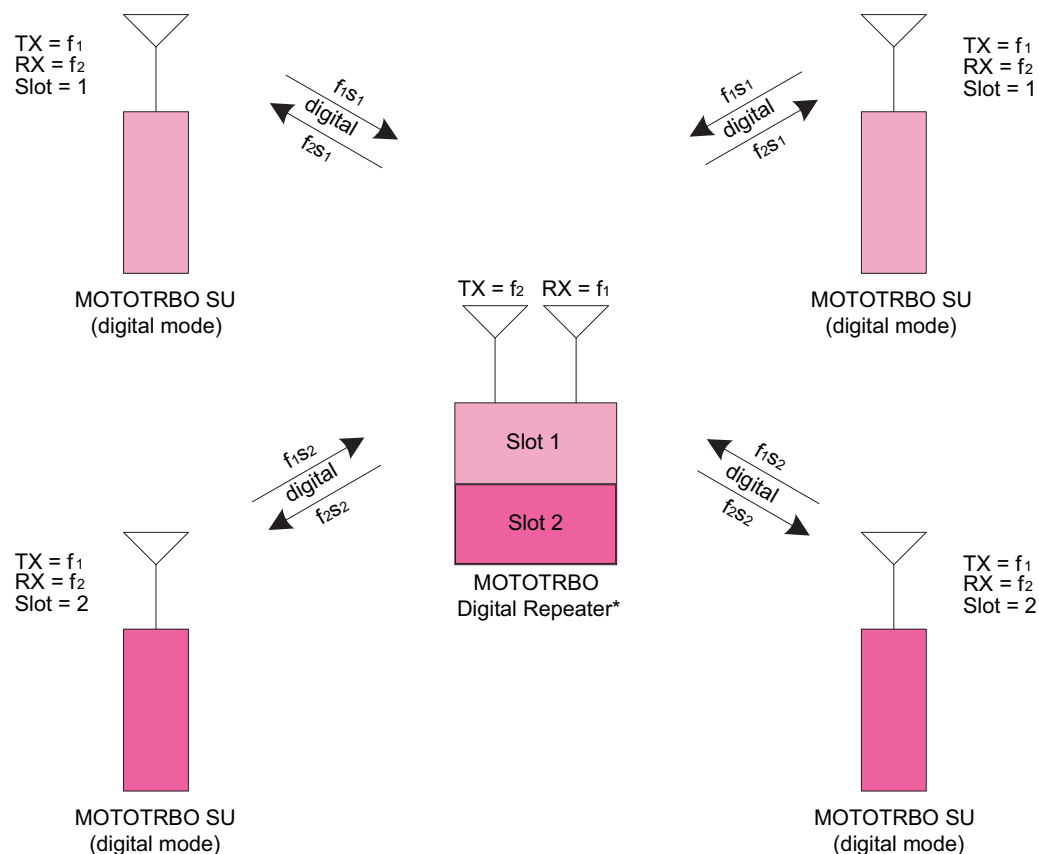
Figure 3-23 MOTOTRBO Digital Radios on MOTOTRBO Two-Slot Digital Repeater
