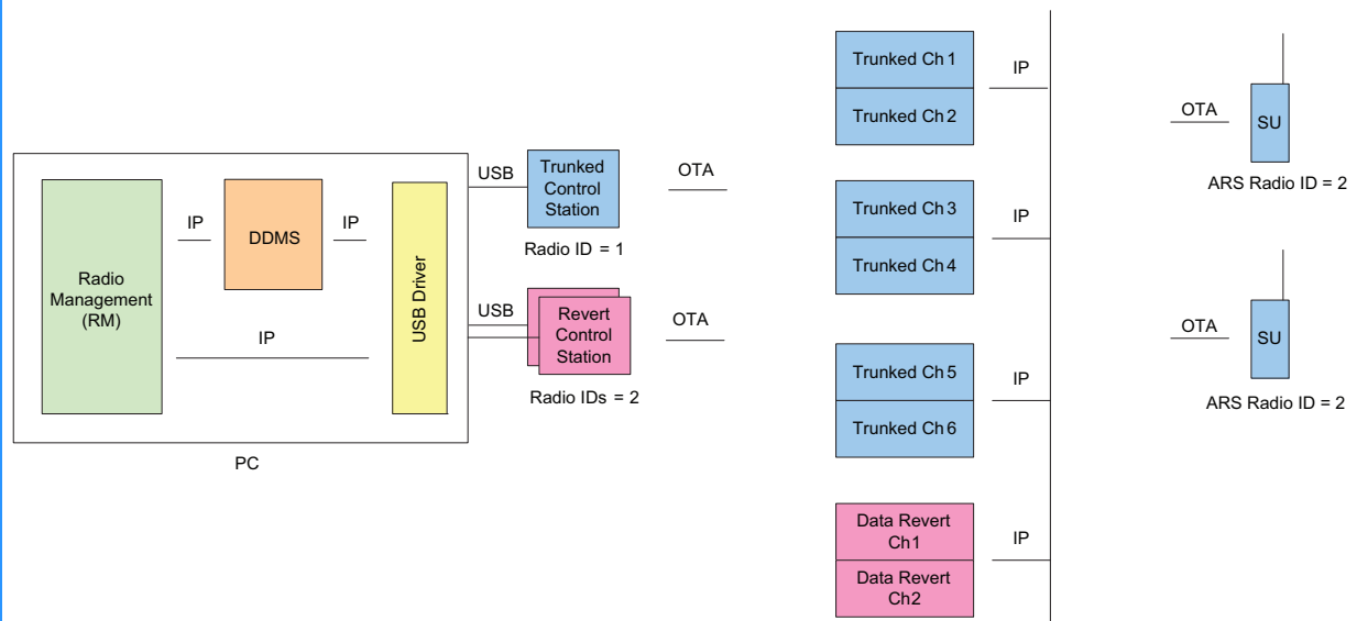
Figure 4-57 RM Application in a Capacity Plus System with a DDMS, Data Revert Channels, and Control Stations
