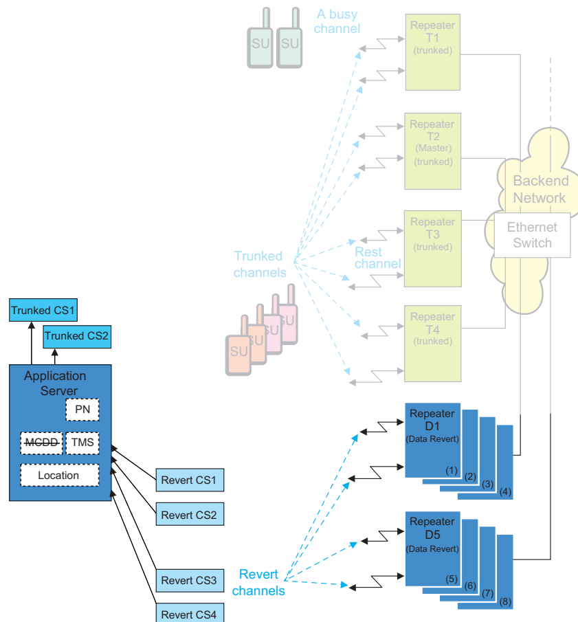
Figure 3-48 Capacity Plus Devices with Data over Revert Channels
