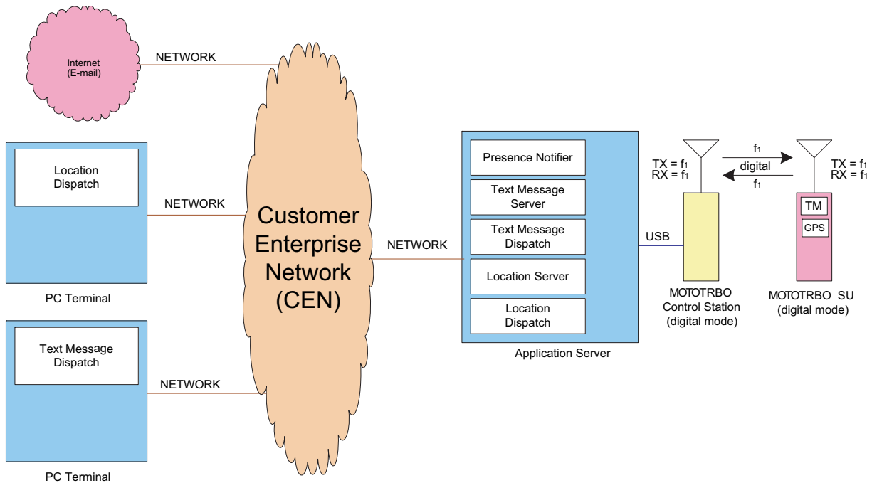
Figure 3-16 MOTOTRBO Radios In Digital Direct Mode/Dual Capacity Direct Mode Server Based Configuration with Remote Dispatchers
