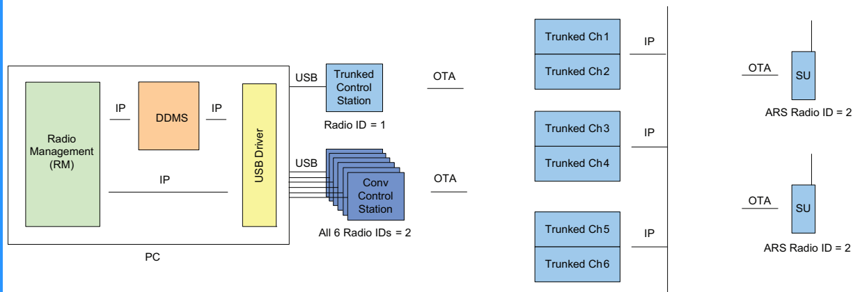
Figure 4-56 RM Application in a Capacity Plus System with a DDMS and One Trunked and Numerous Conventional Control Stations
