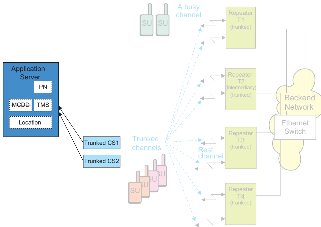
Figure 3-46 Capacity Plus Devices with Data over Trunked Channels
