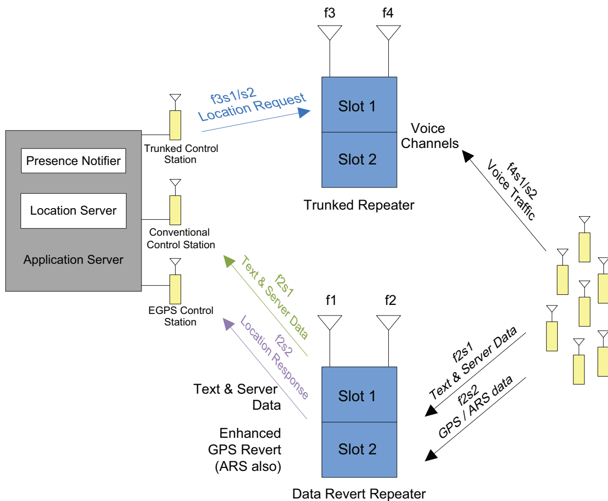
Figure 3-33 A Capacity Plus System with an Enhanced GPS Revert Channel
