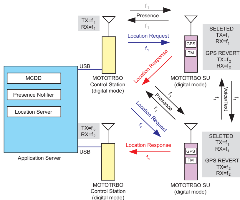
Figure 3-18 MOTOTRBO Radios in Two Channel Direct Mode GPS Revert Configuration
