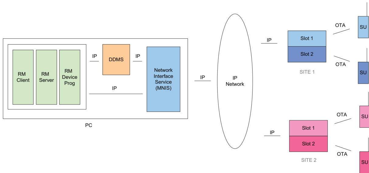
Figure 4-48 RM Application with MNIS Covering RF Isolated Single Site Repeater
