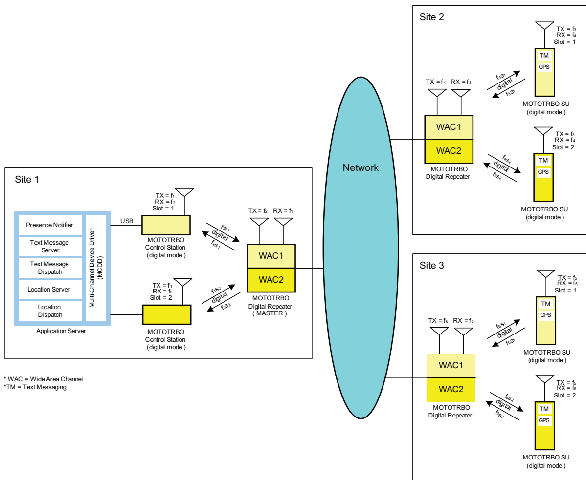
Figure 3-37 Wide Area System with Centralized Data Application Server
