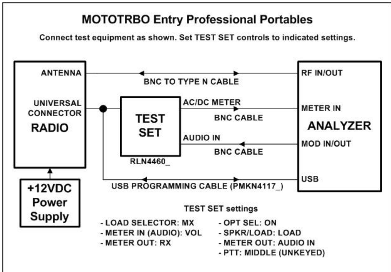
Figure 4-2. MOTOTRBO™ Portable Entry Professional Test Setup Diagram.
