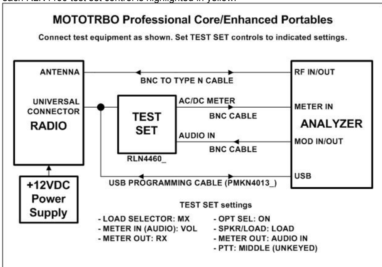
Figure 4-1. MOTOTRBO™ Portable Professional Core/Enhanced Test Setup Diagram
