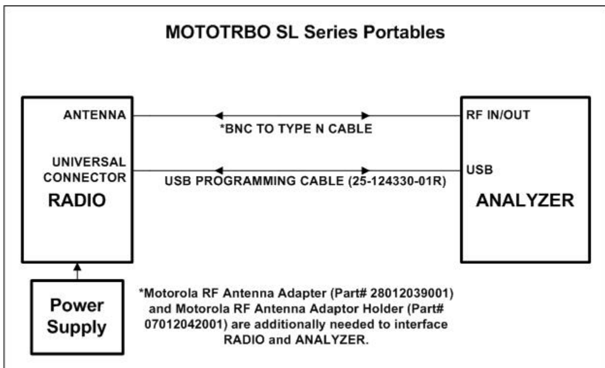
Figure 4-3. MOTOTRBO™ Portable SL Series Radio Test Setup Diagram.
