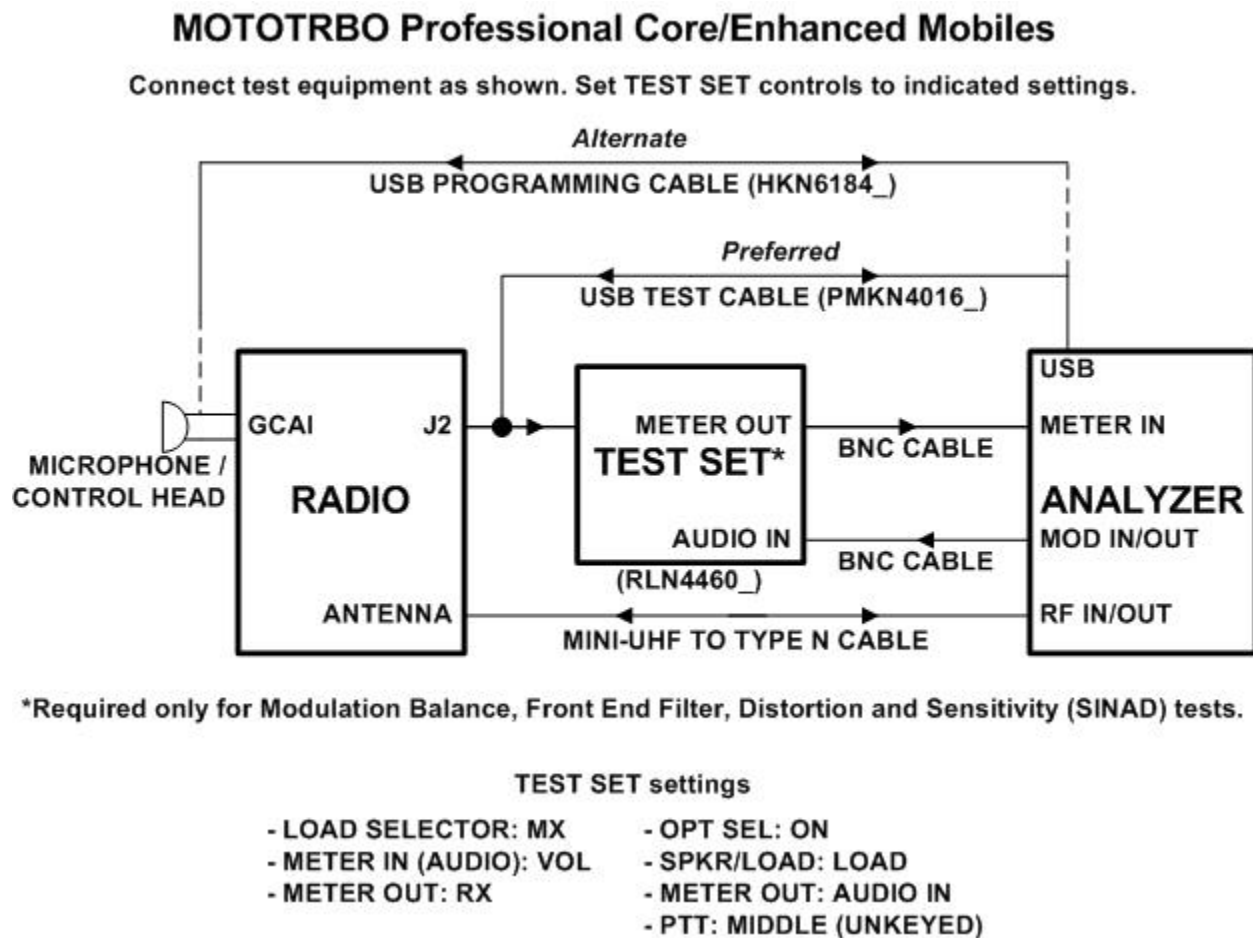
Figure 6-1. MOTOTRBO™ Mobile Professional Core/Enhanced Test Setup Diagram.
