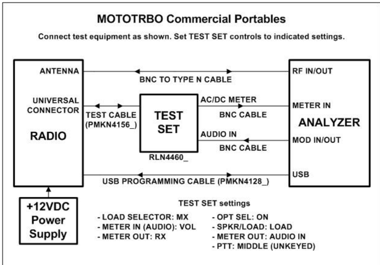
Figure 4-4. MOTOTRBO™ Portable Commercial Test Setup Diagram.
