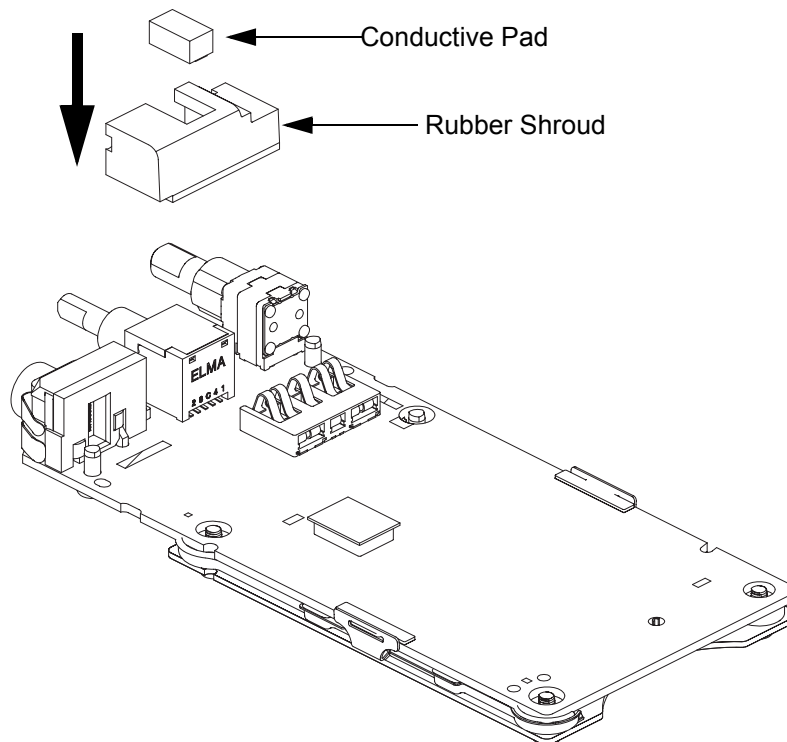
Figure 5-16. Conductive Pad and Rubber Shroud Reassembly.
