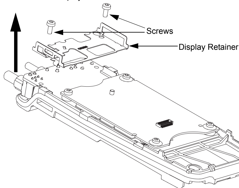
Figure 5-6. LCD Retainer removal.
