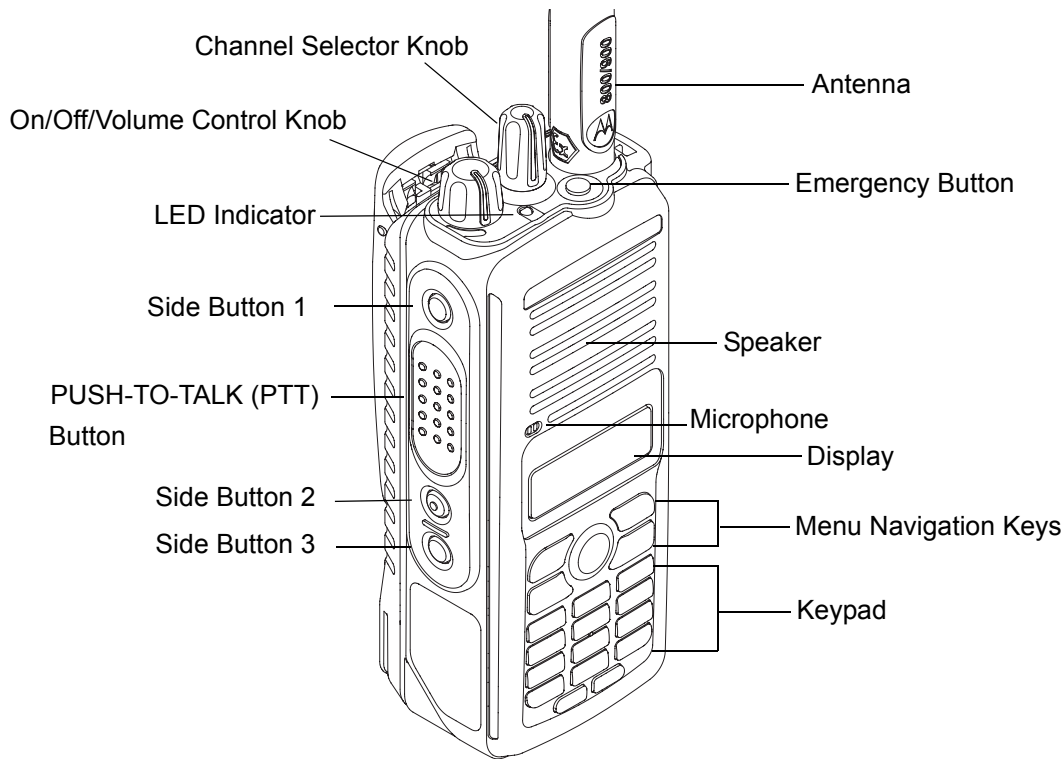
Figure 1-2. Display Model (IECEX/CSA 800/900)
