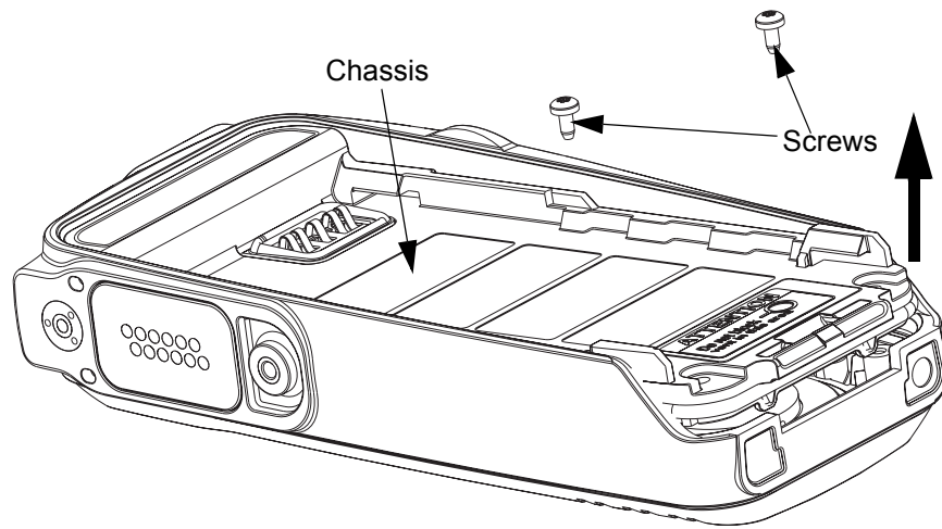
Figure 5-4. Chassis removal.
