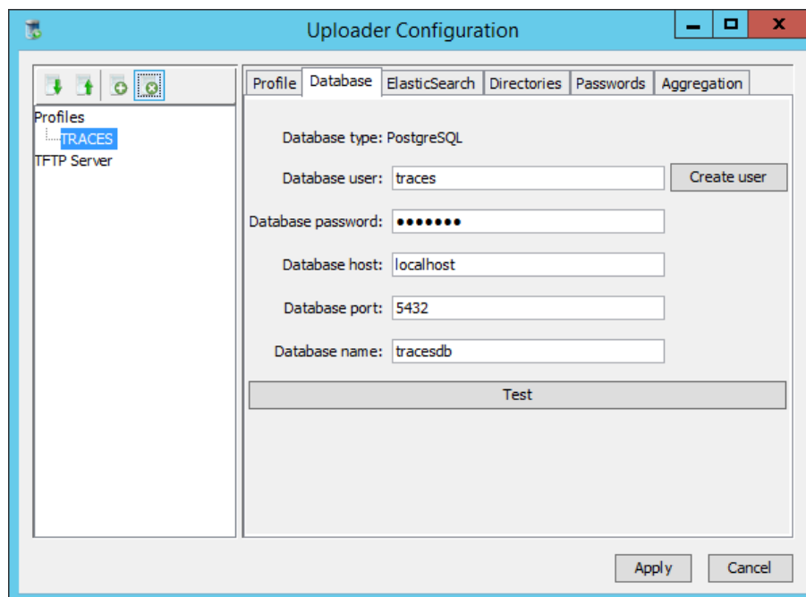
Figure 3: Uploader Configuration – Database tab
