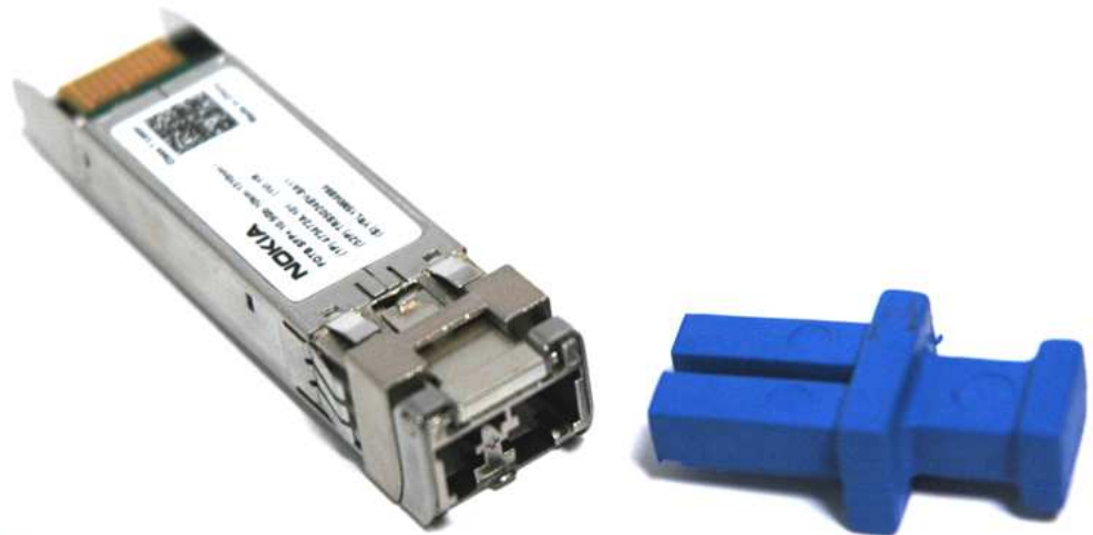
Figure 2 10GBase interface
