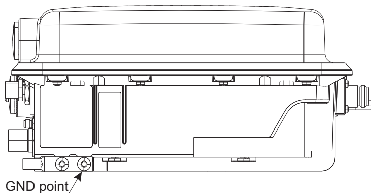
Figure 12 Flexi Zone Micro BTS (FWFA, FWEA, FWHE, FWHF, FWHO, FWHN) side view interfaces
