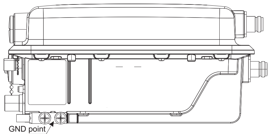
Figure 18 Flexi Zone Micro BTS (FWHC, FWHM) side view interfaces
