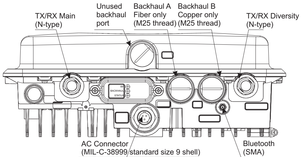
Figure 10 Flexi Zone Micro BTS (FWFA, FWEA, FWHE, FWHF, FWHO, FWHN) bottom view interfaces
