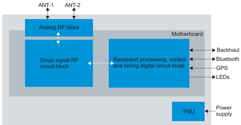
Figure 6 Flexi Zone Micro BTS (FWHD) functional diagram
