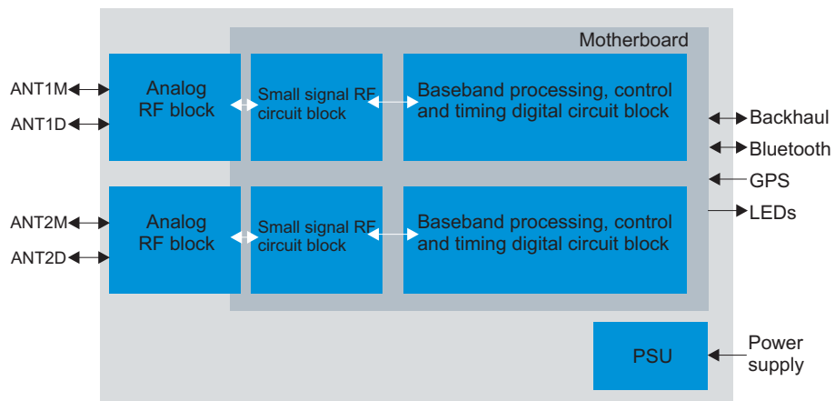
Figure 6 Flexi Zone Micro BTS (FWHD) functional diagram
