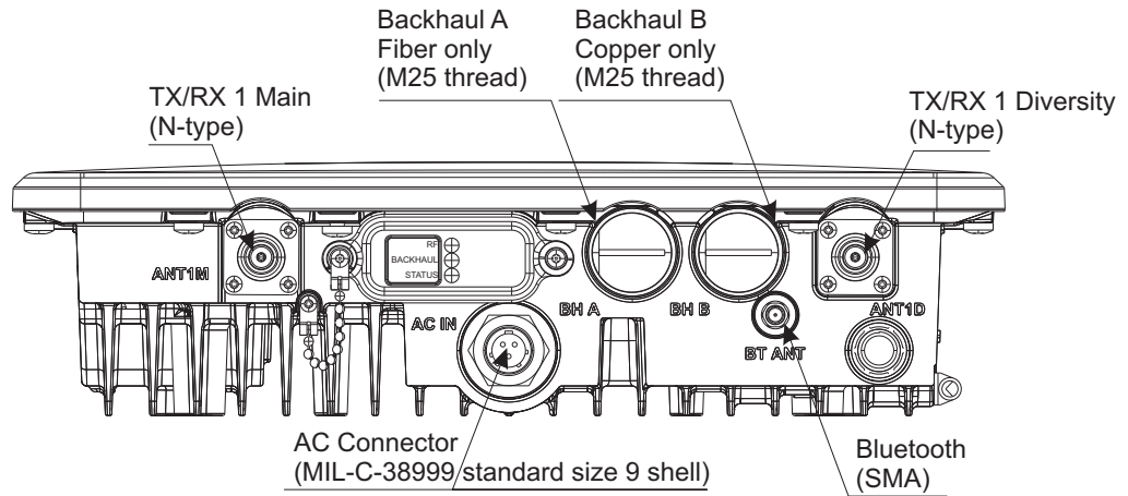
Figure 14 Flexi Zone Micro BTS (FWHD) top view interfaces
