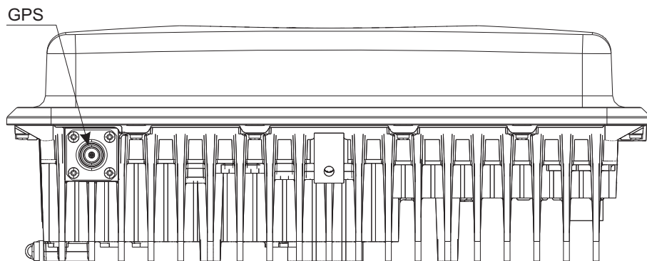
Figure 12 Flexi Zone Micro BTS (FWFA, FWEA, FWHE, FWHF, FWHO, FWHN) side view interfaces
