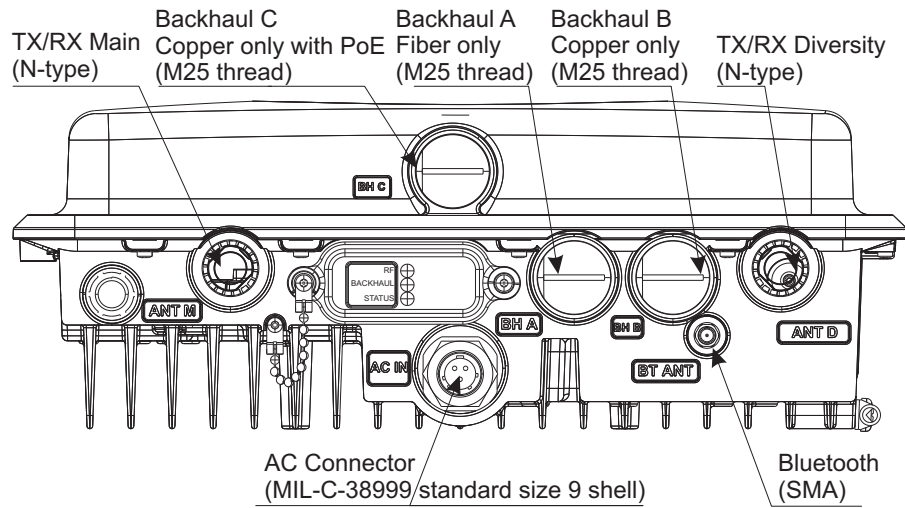
Figure 17 Flexi Zone Micro BTS (FWHC, FWHM) top view interfaces
