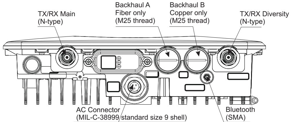
Figure 8 Flexi Zone Micro BTS (FWGB, FWHA, FWIB) top view interfaces
