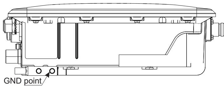
Figure 9 Flexi Zone Micro BTS (FWGB, FWHA, FWIB) side view interfaces
