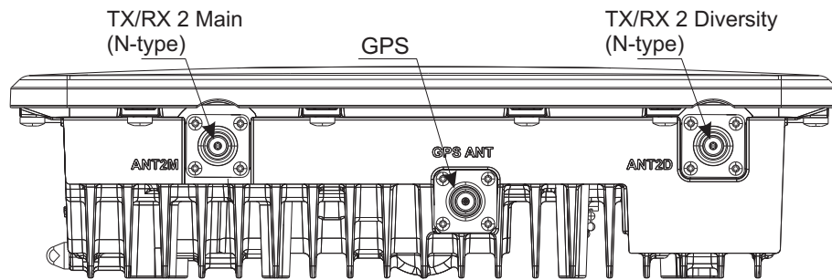
Figure 15 Flexi Zone Micro BTS (FWHD) side view interfaces
