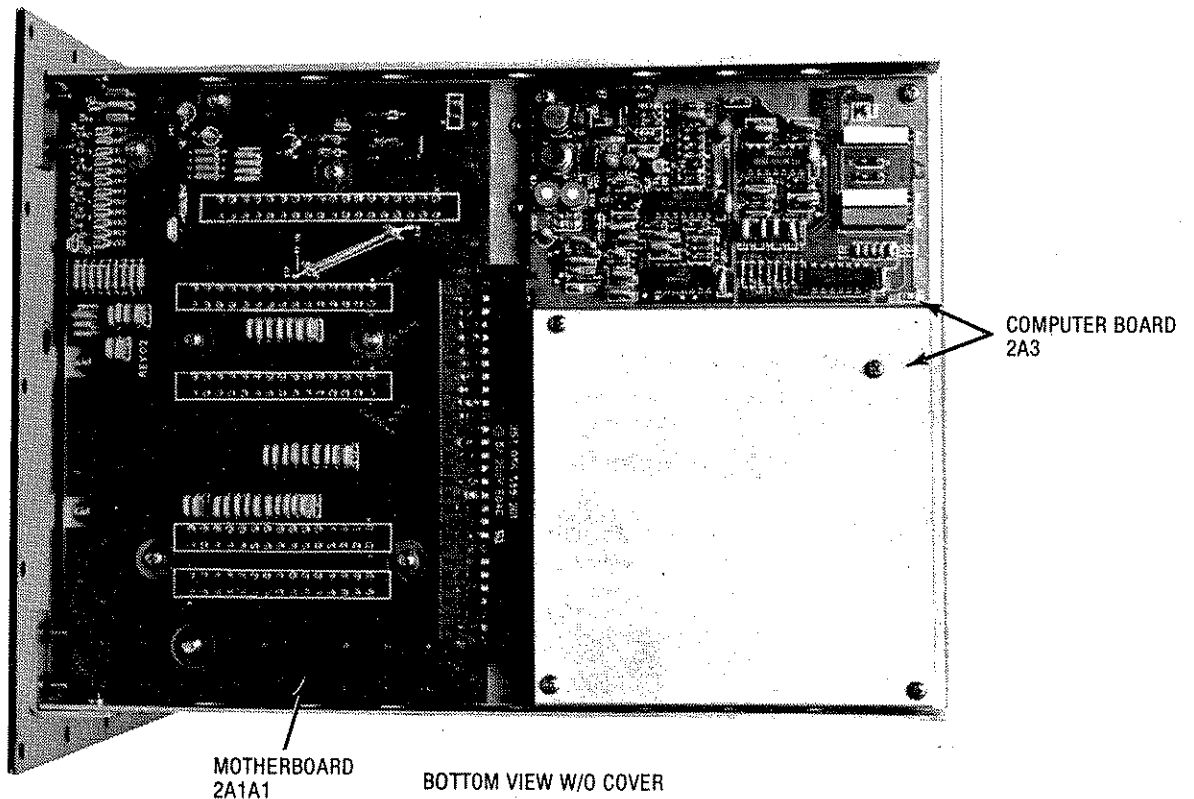
Figure 1.1 DCU-100 Major Assembly Locations
