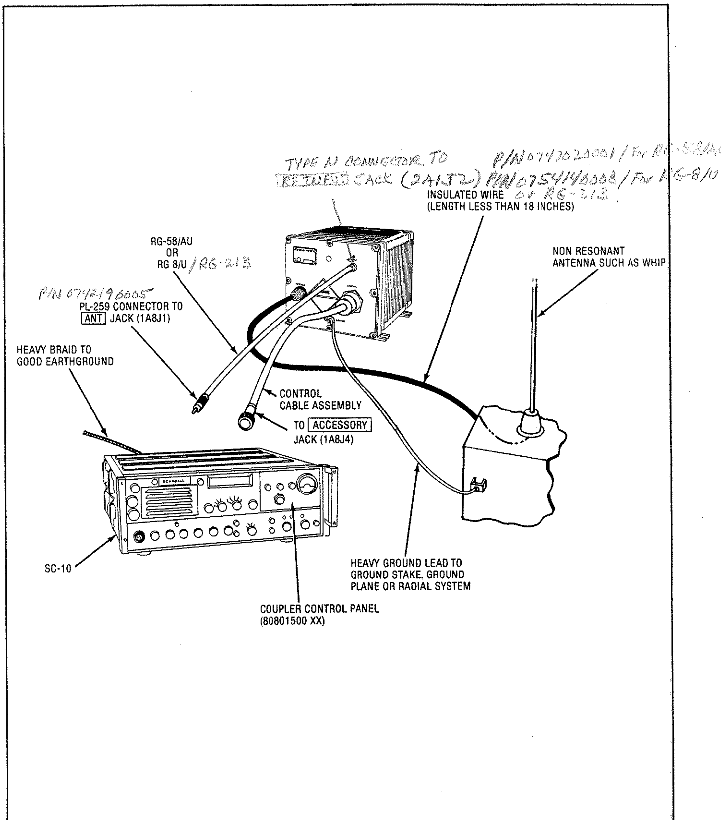
Figure 2.2 Typical Base Station Installation Using Non-Resonant Antennas
