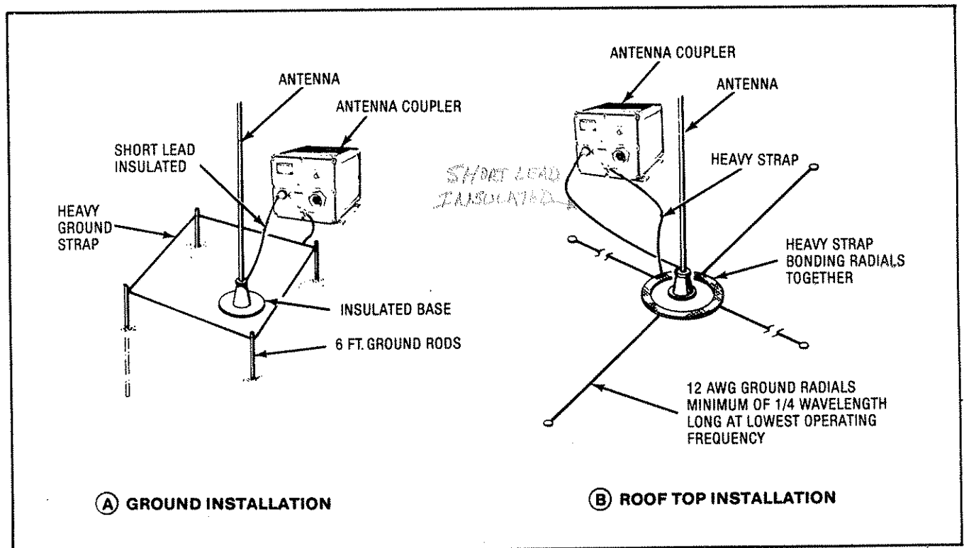
Figure 2.5 Whip Antenna
