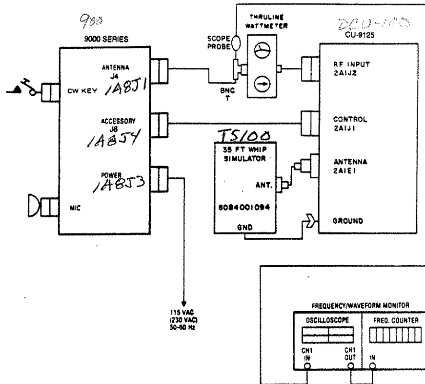
ANTENNA COUPLER TEST SETUP
