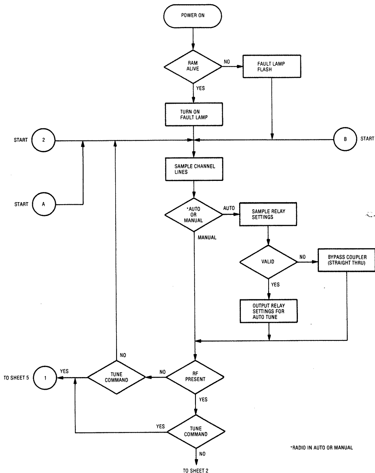
Figure 4.2 DCU-100 Flow Chart (Sheet 1 of 5)
