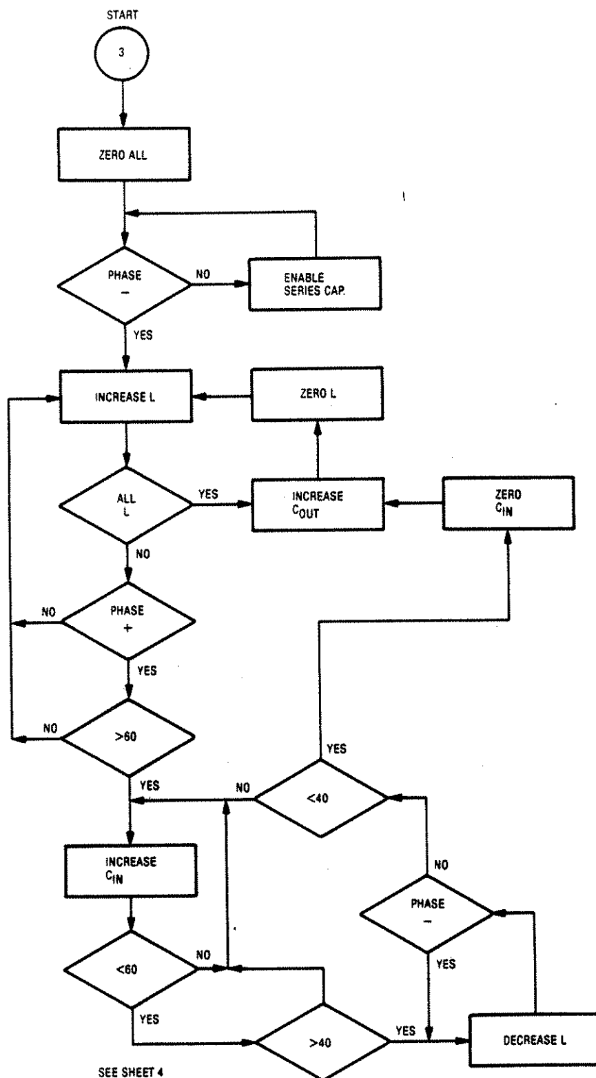
Figure 4.2 DCU-100 Flow Chart (Sheet 3 of 5)
