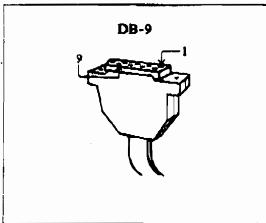
DB-9 PIN
