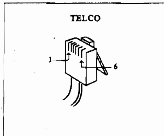
TELCO PIN
