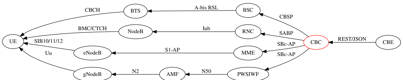
Figure 1: Role of the CBC inside the 3GPP network architecture (3GPP TS 23.041 §3)
