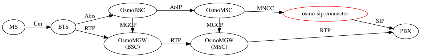
Figure 1: Typical GSM network architecture used with OsmoSIPConnector
