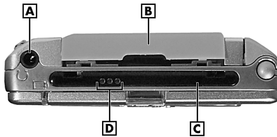
MobilePro P300 Top Features
