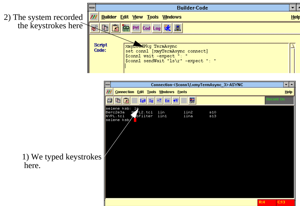
Figure 12-24. Capturing Events on the Remote Asynchronous System
