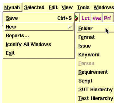
Figure 1-1. Cascading Menu Example
