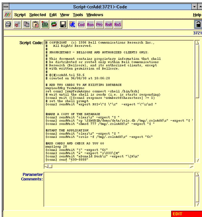
Figure 10-5. Script Object Code View
