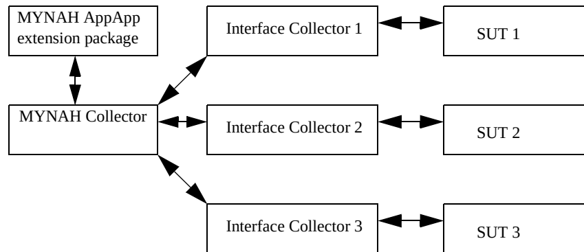
Figure 12-1. MYNAH General AppApp Interactions
