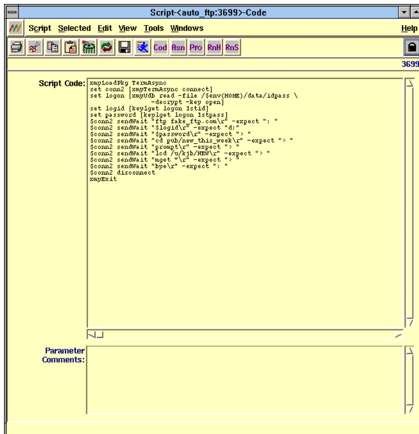
Figure 2-1. MYNAH GUI Script Object Code View
