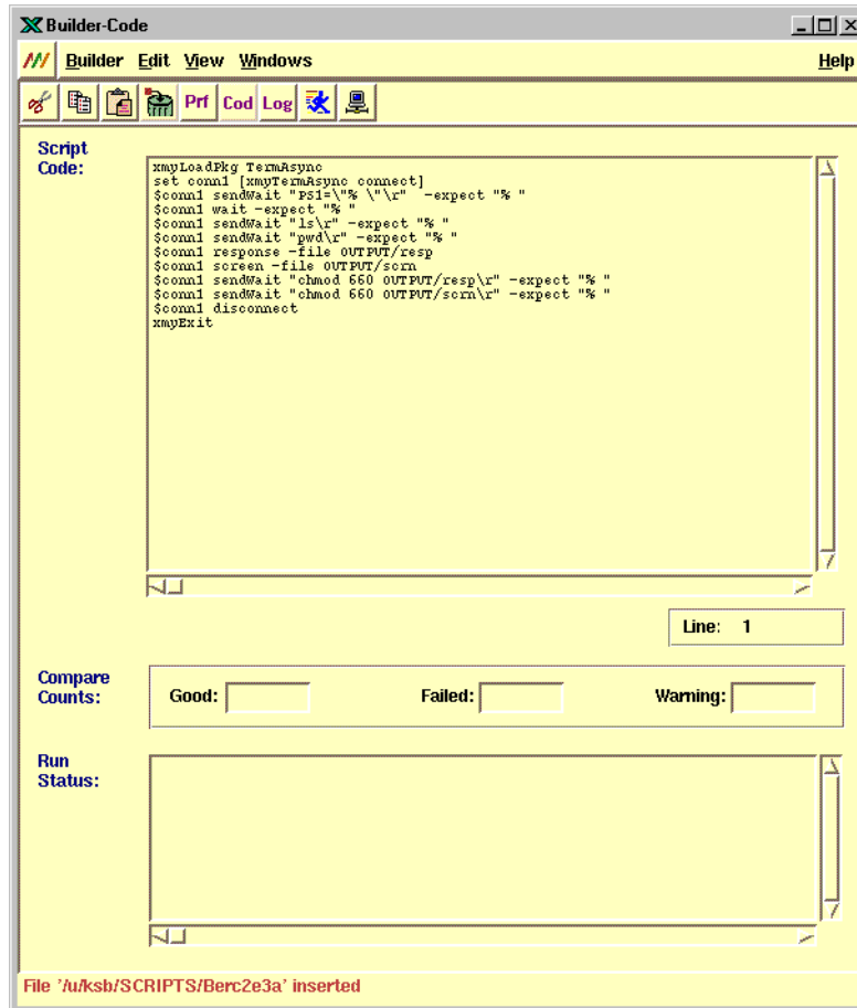
Figure 2-2. MYNAH Script Builder Code View
