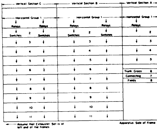
Fig. 2—Apparatus Side of District Group Frame
