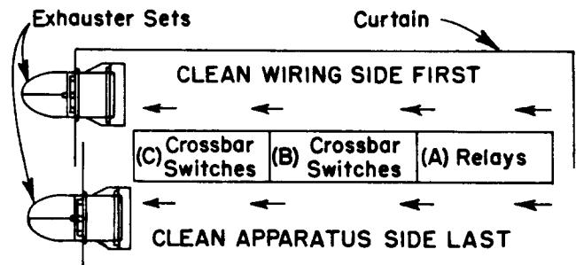
Fig. 1—Curtain Enclosed Frame With Exhaustor Sets in Place
