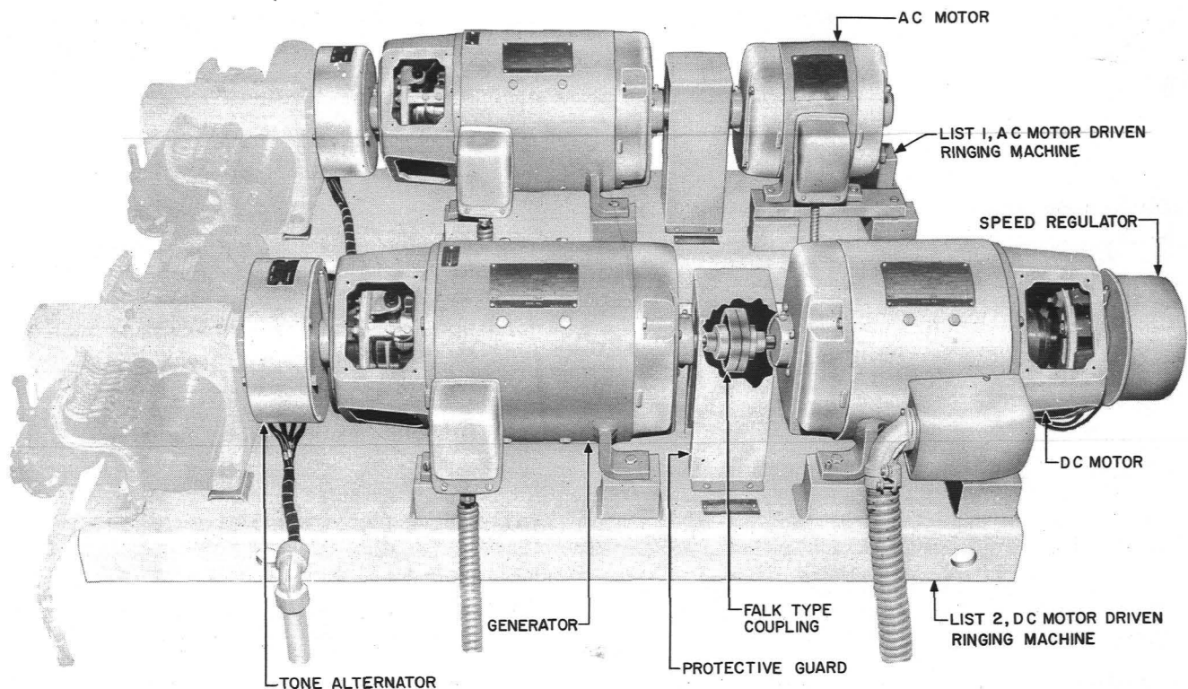
Fig. 1 - KS-15816 Ringing Machines
