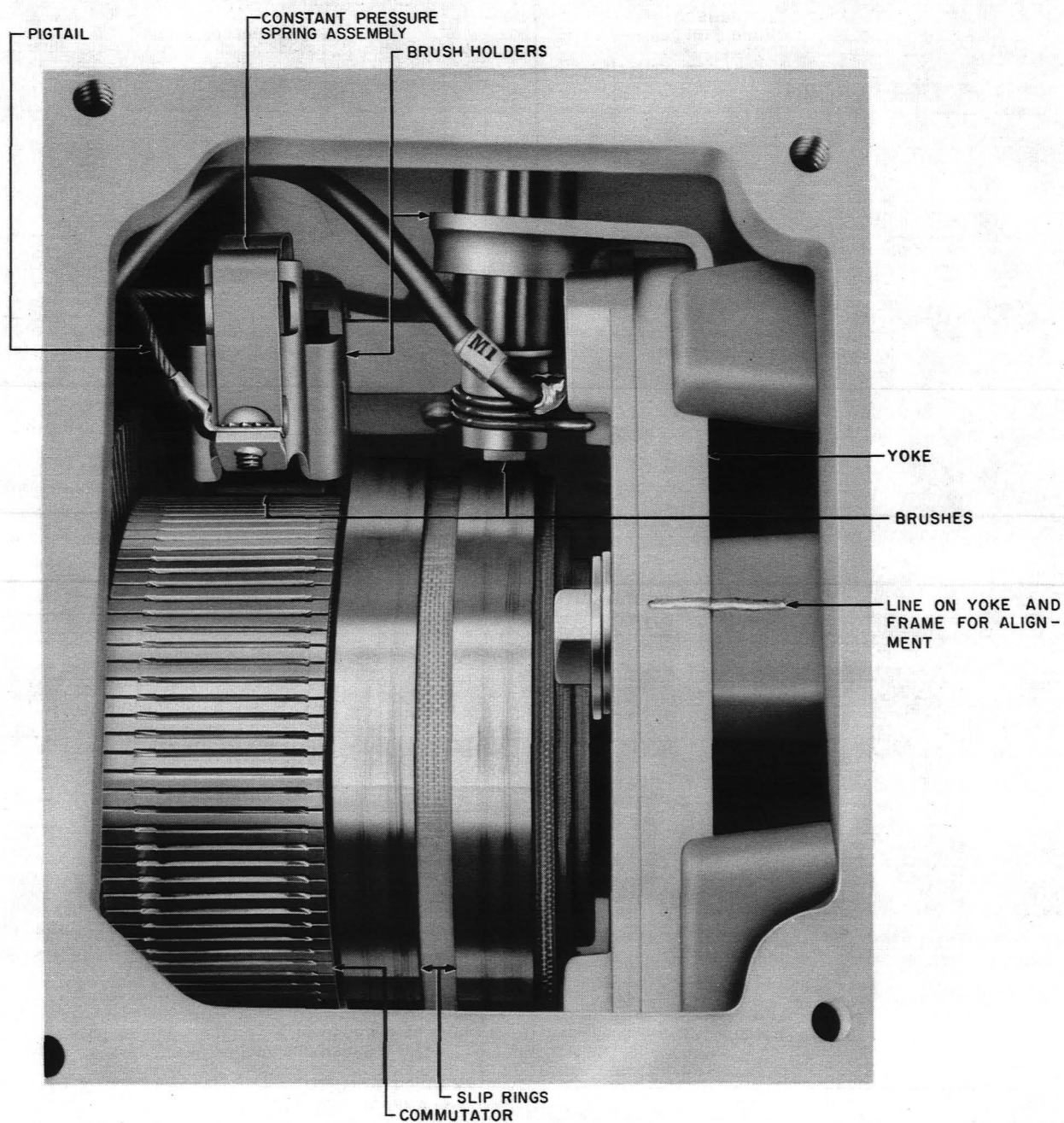
Fig. 4 - Yoke, Slip Rings, and Commutator
