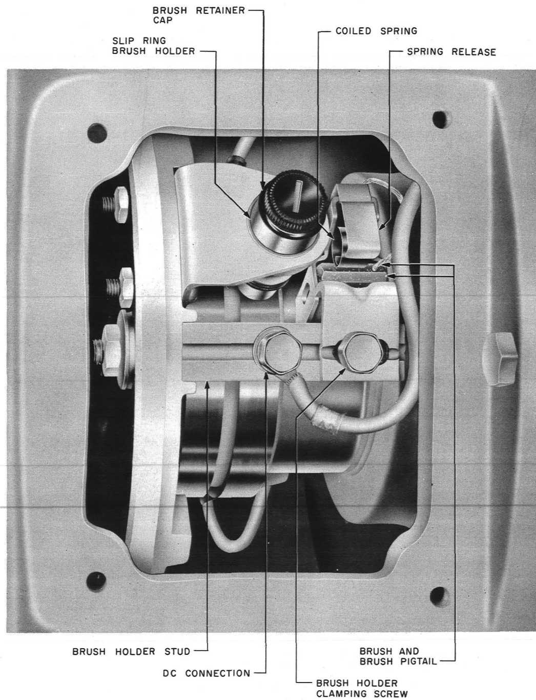
Fig. 3 – Yoke and Brush Rigging
