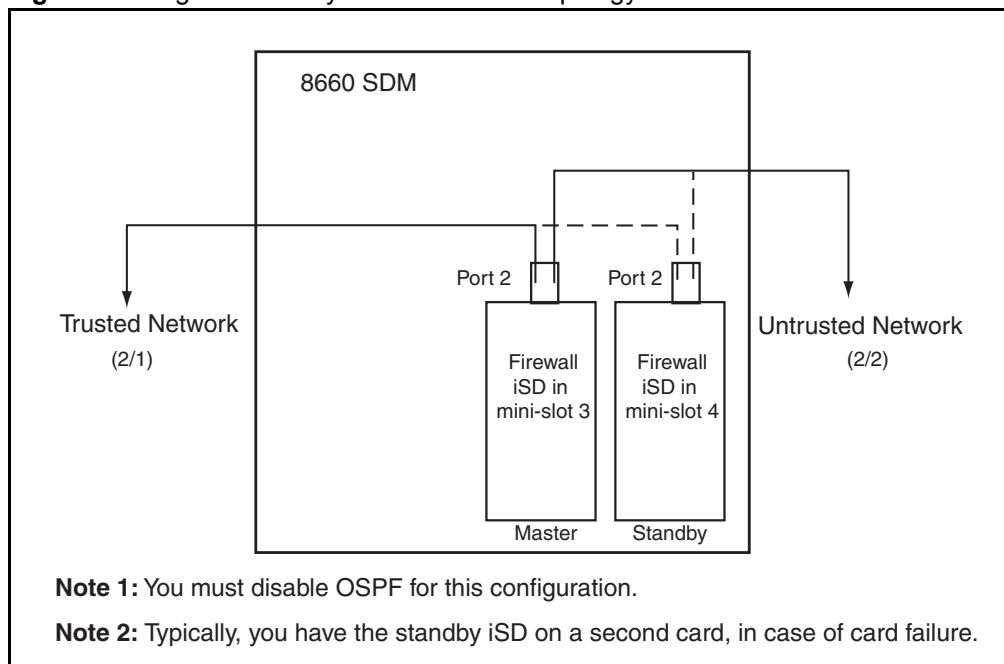
Figure 9-1 High-Availability firewall network topology
