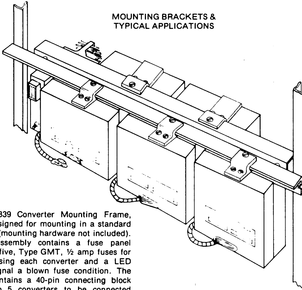
FIGURE 6 100339 MOUNTING FRAME ASSEMBLY
