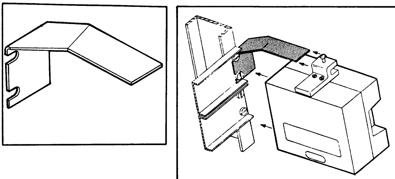
FIGURE 8 201067 CROSSBAR ADAPTER
