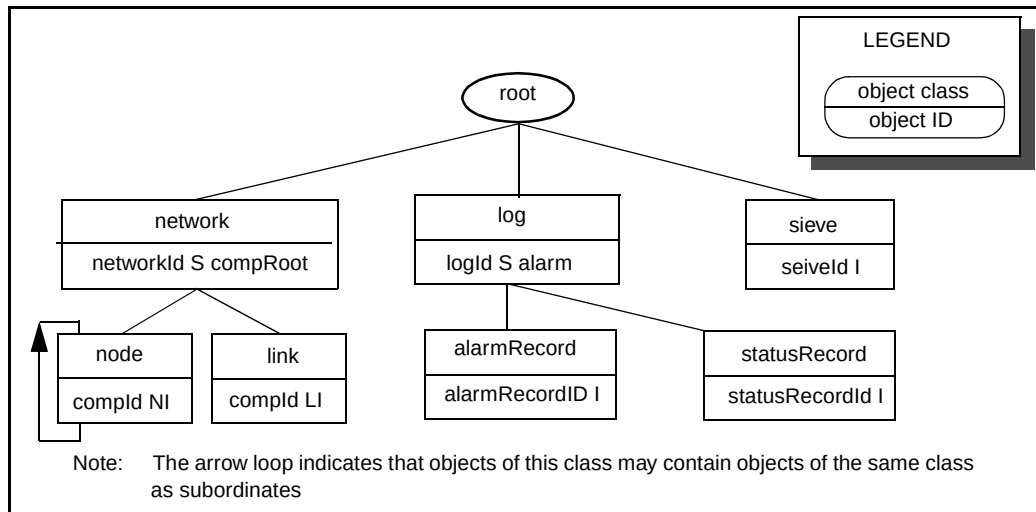
Figure 3 Alarm and Status API object model naming hierarchy
