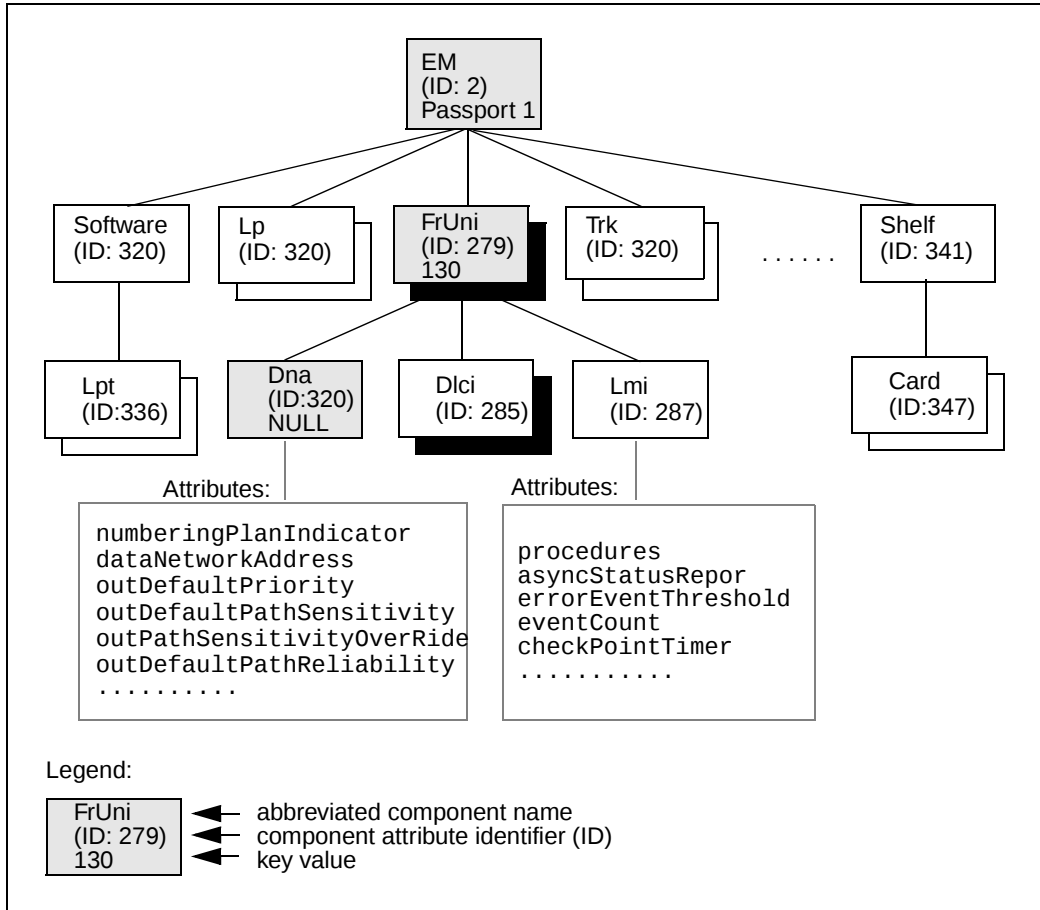
Figure 4 Example of a service data containment hierarchy
