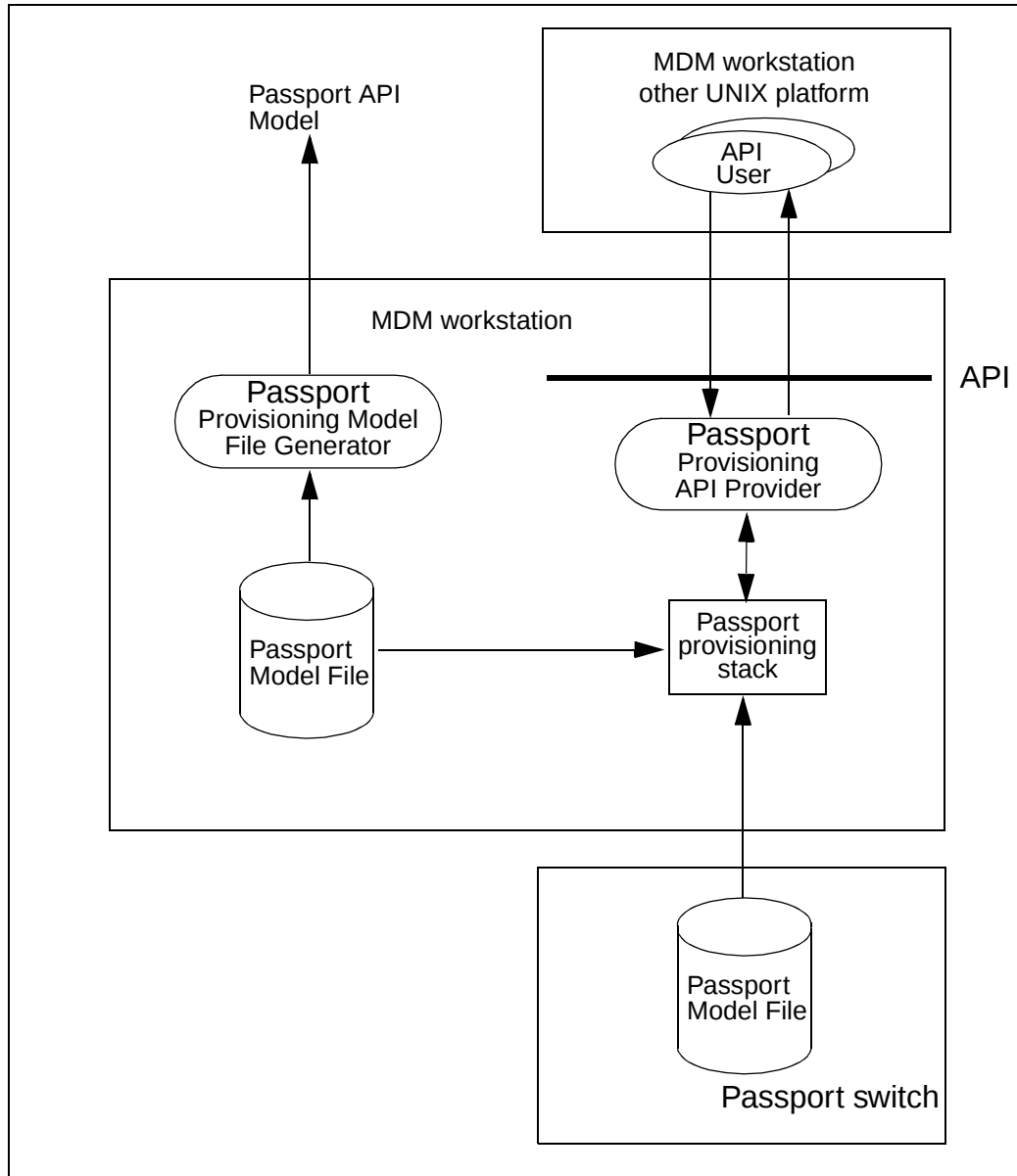
Figure 2 Generating Provisioning API Model files from Passport Model files
