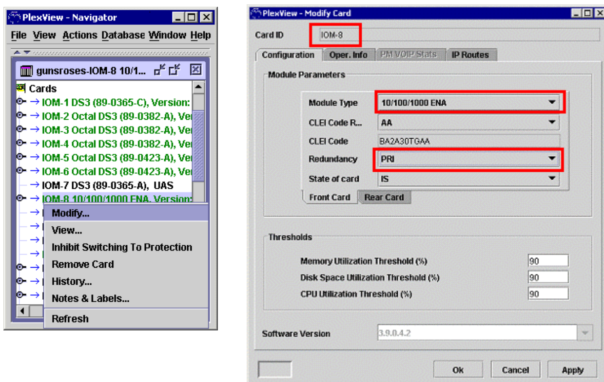
Figure 8. Ethernet IOM Module Front Card
