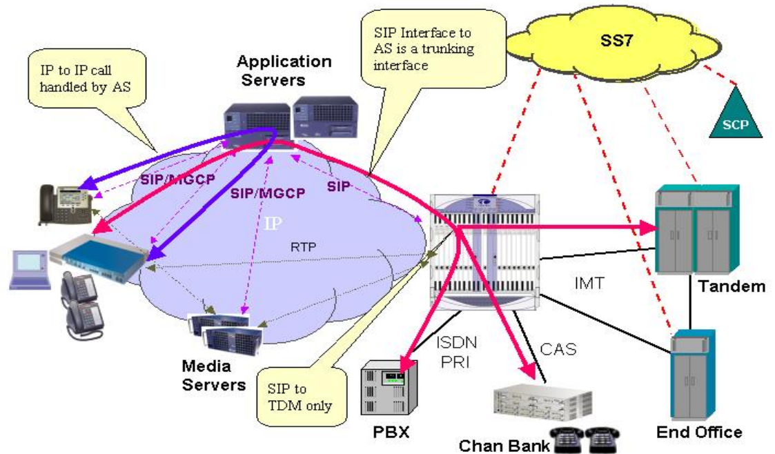
Figure 1 - The Switch Provides IP Centrex and PSTN Access for IP
