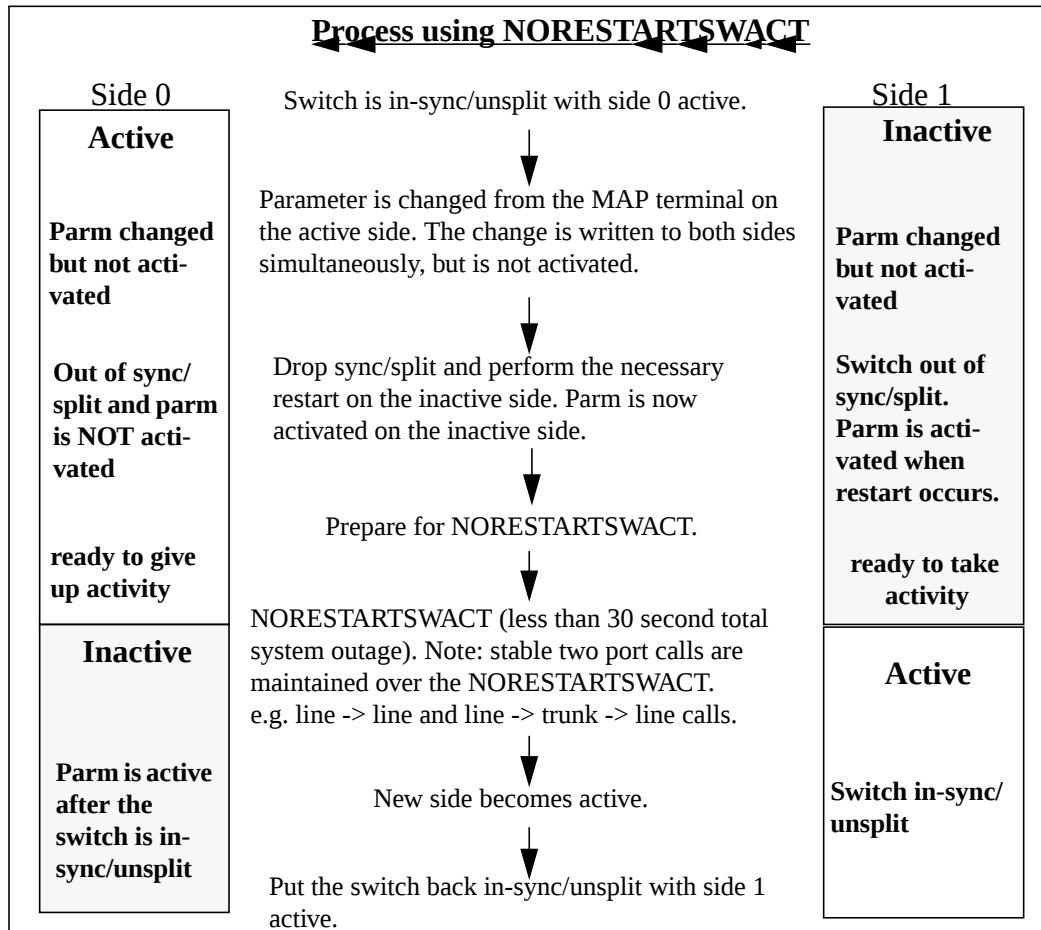
FIGURE 3. NORESTARTSWACT change activation
