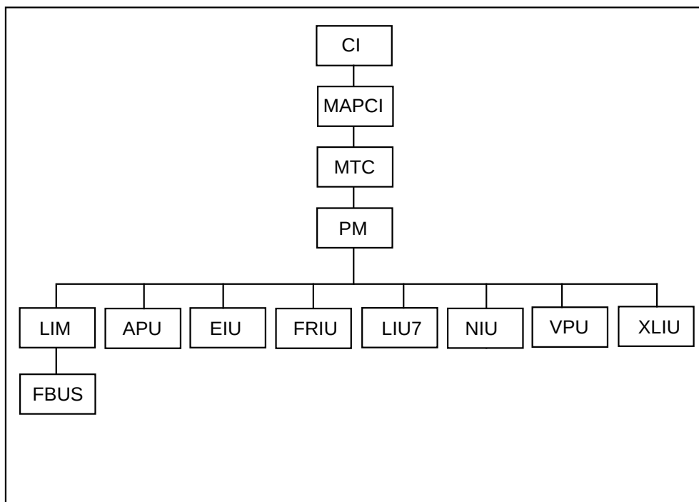
Figure 41-5 F-bus-related MAP levels
