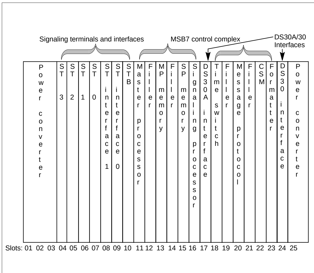
Figure 13-7 MSB7 STA7 shelf
