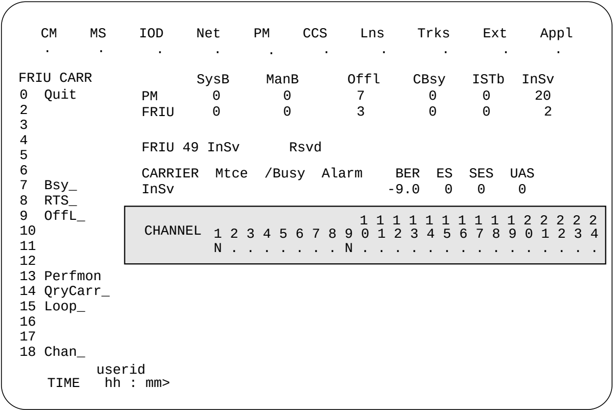
Figure 41-14 FRIU CARR level system status display
