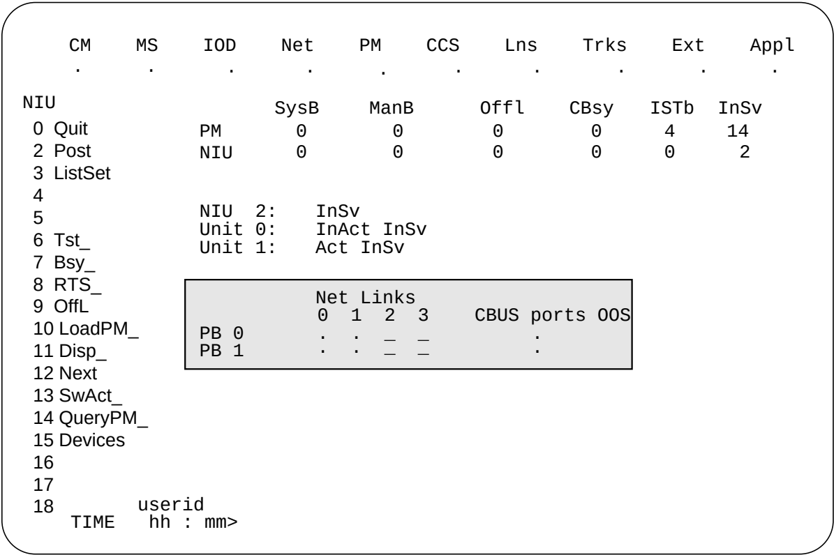
Figure 41-17 NIU-level system status display
