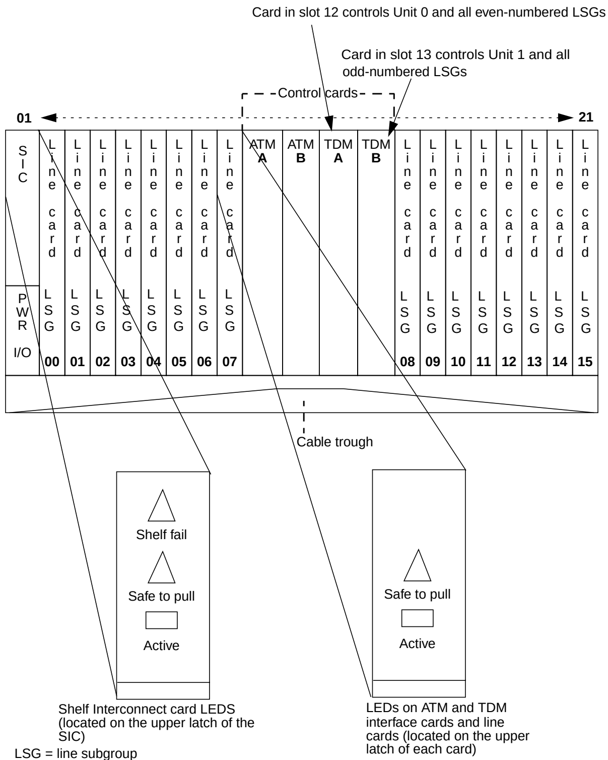
Figure 24-3 NTNP10BA UE9000 DMS shelf
