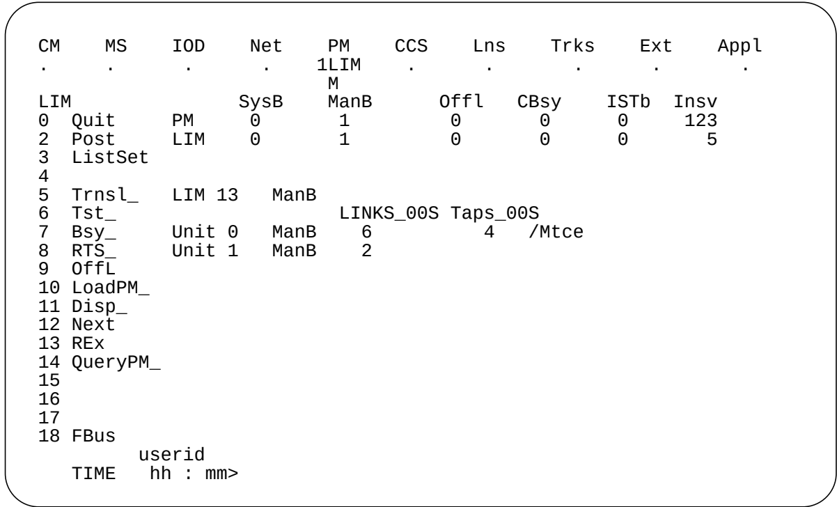
Figure 41-4 LIM-level system status display
