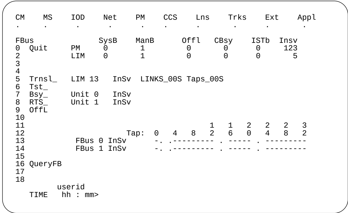
Figure 41-6 FBUS-level system status display
