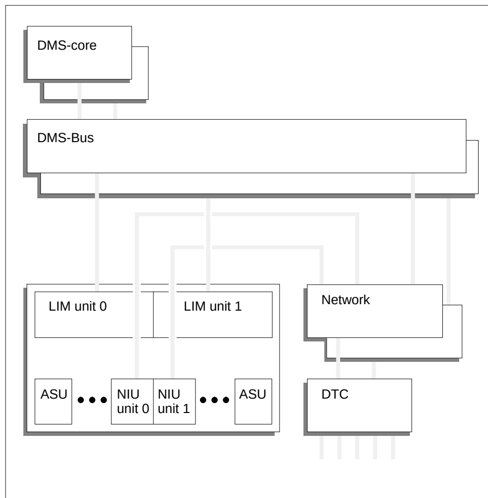
Figure 36-16 Functional architecture of NIU-supported LPP
