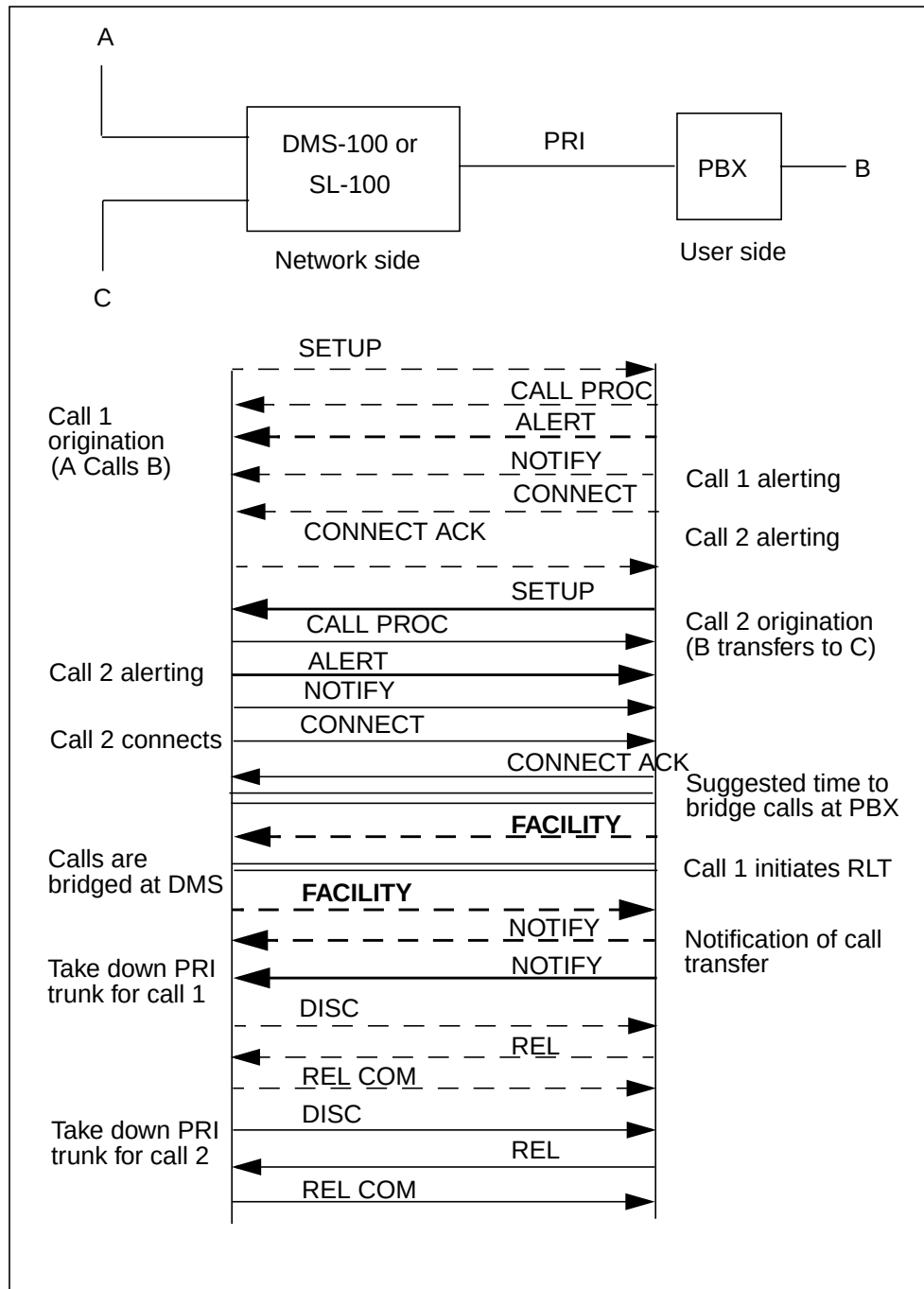
Figure 6-21 Messaging sequence for RLT with Call Transfer
