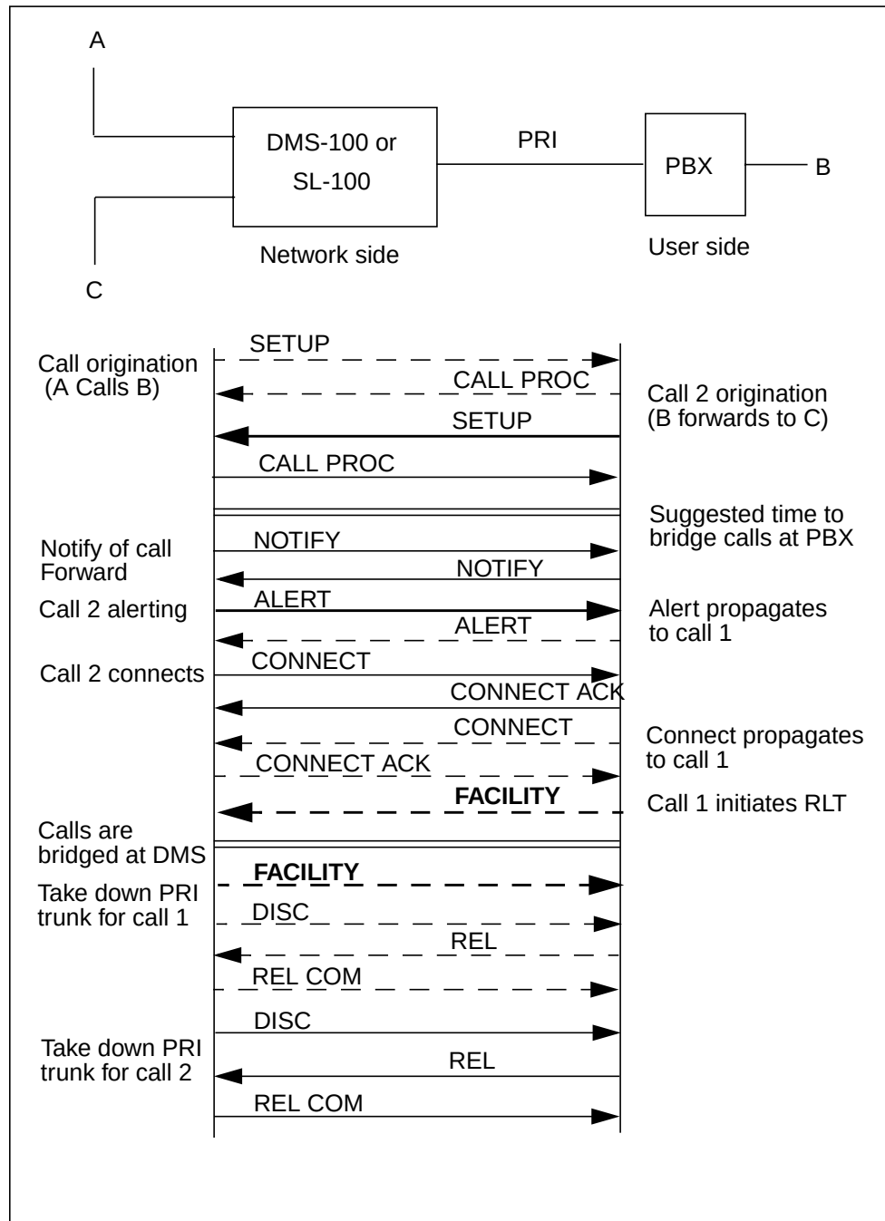
Figure 6-19 Messaging sequence for RLT with Call Forward
