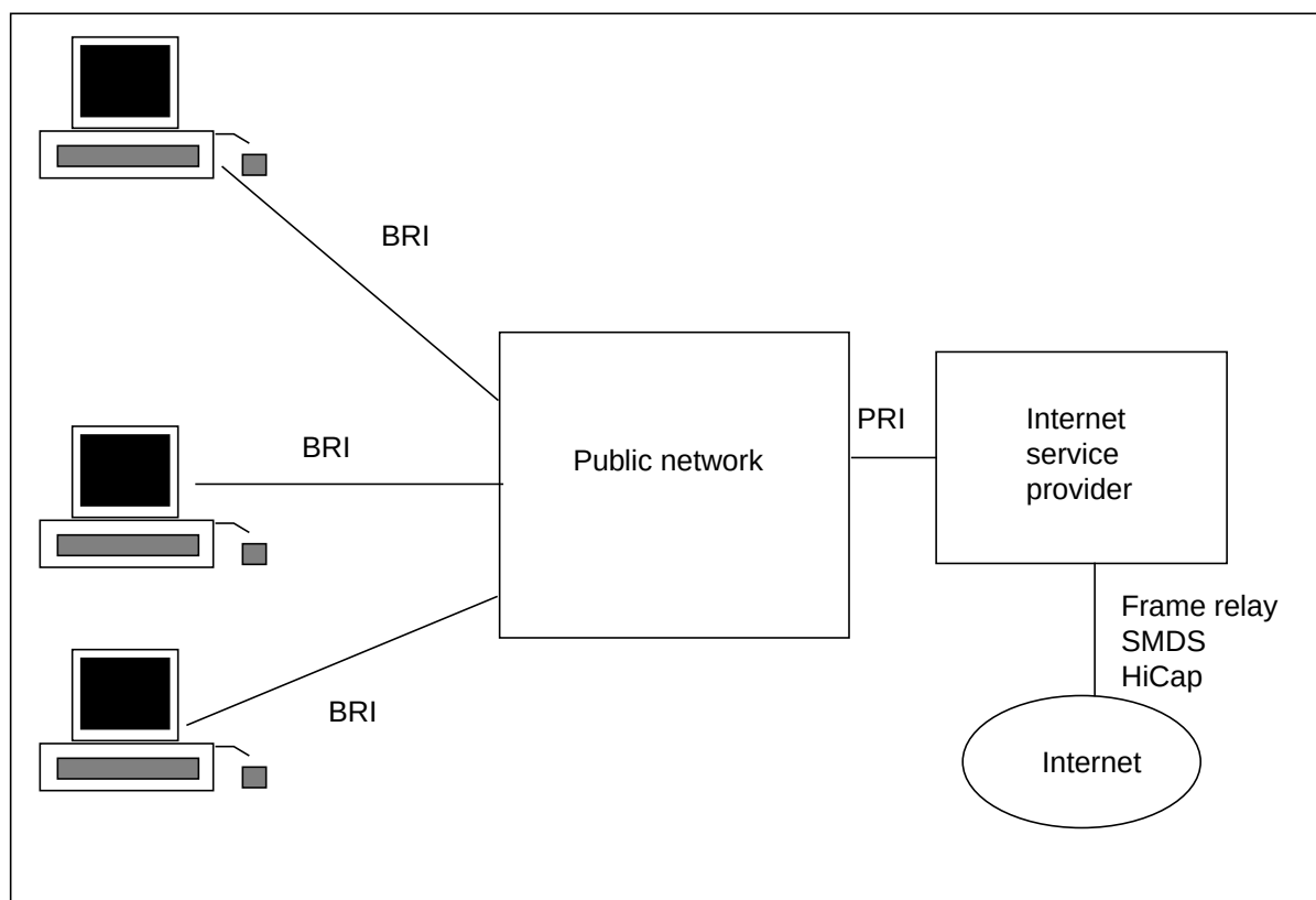
Figure 1-11 PRI Internet access application
