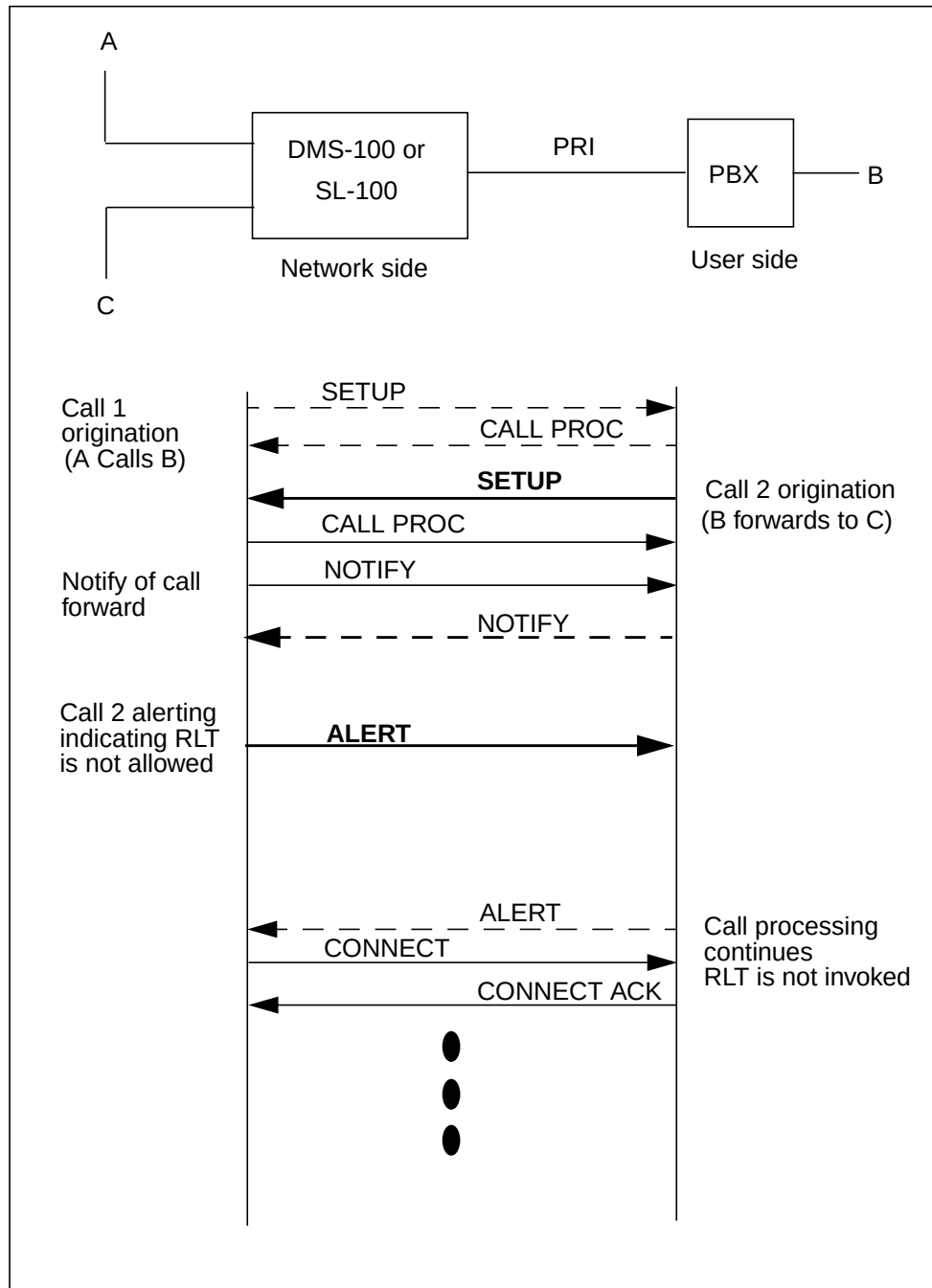
Figure 6-22 RLT not allowed scenario
