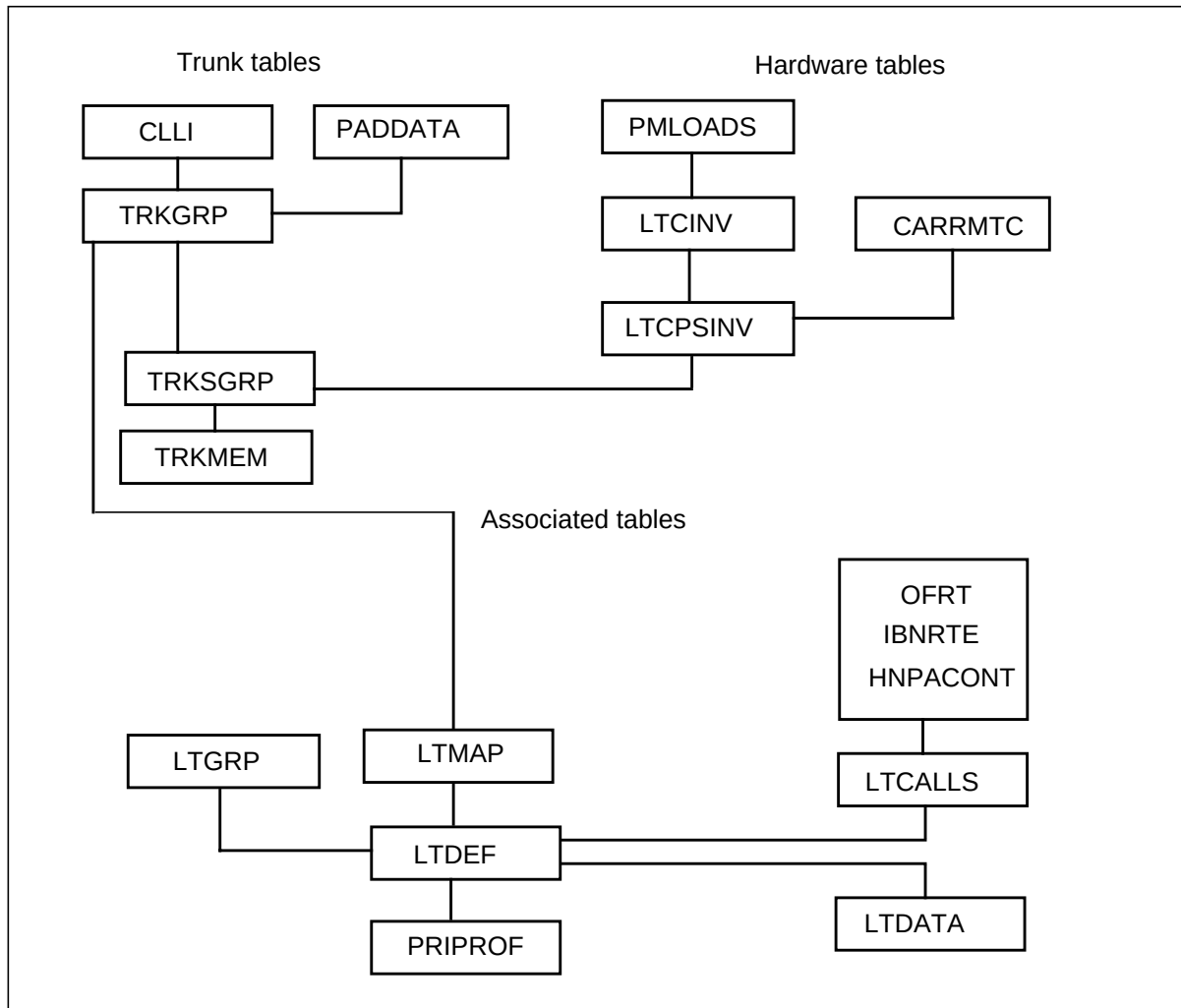
Figure 6-1 PRI datafill table flow
