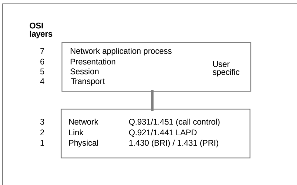
Figure 3-1 OSI and ISDN model comparison
