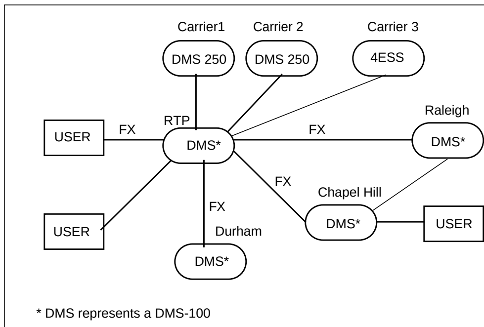
Figure 6-15 Foreign exchange lines
