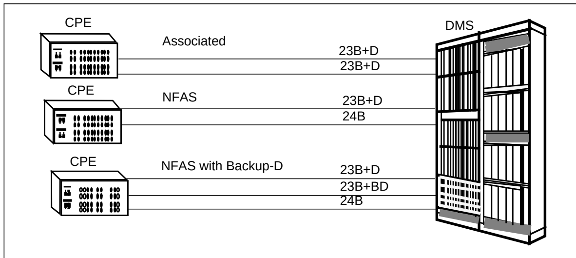
Figure 1-3 PRI configurations
