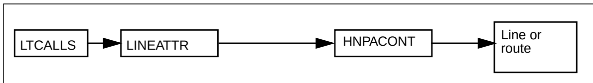
Figure 6-7 Standard routing
