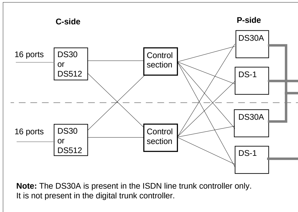
Figure 2-1 XPM hardware configuration
