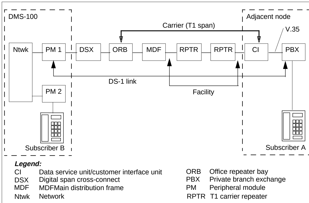
Figure 12-1 PRI hardware model
