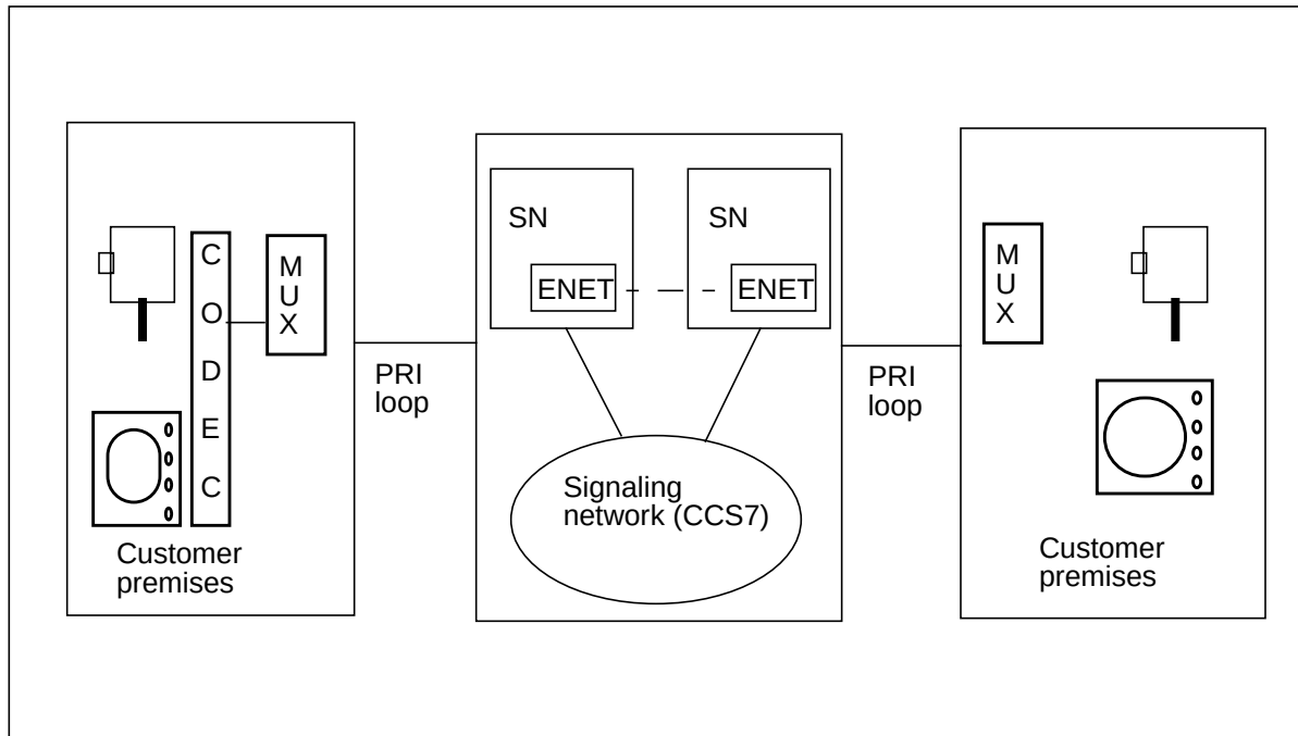
Figure 1-9 Videoconferencing application
