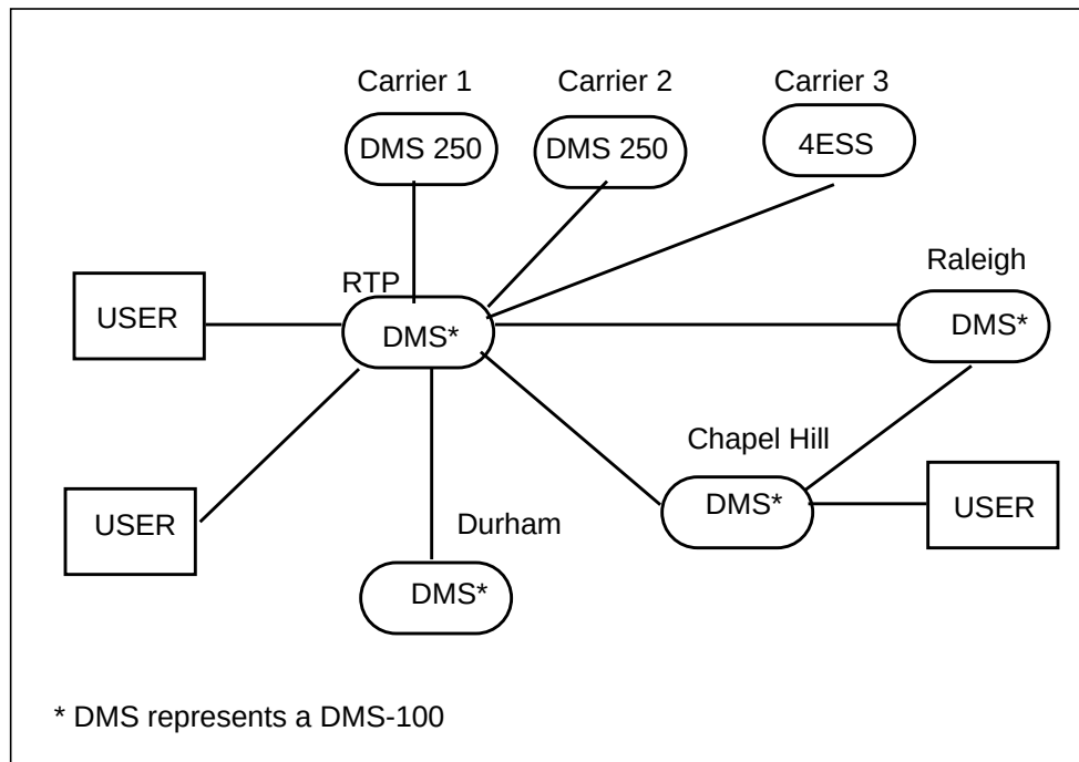
Figure 6-13 Public-switched network
