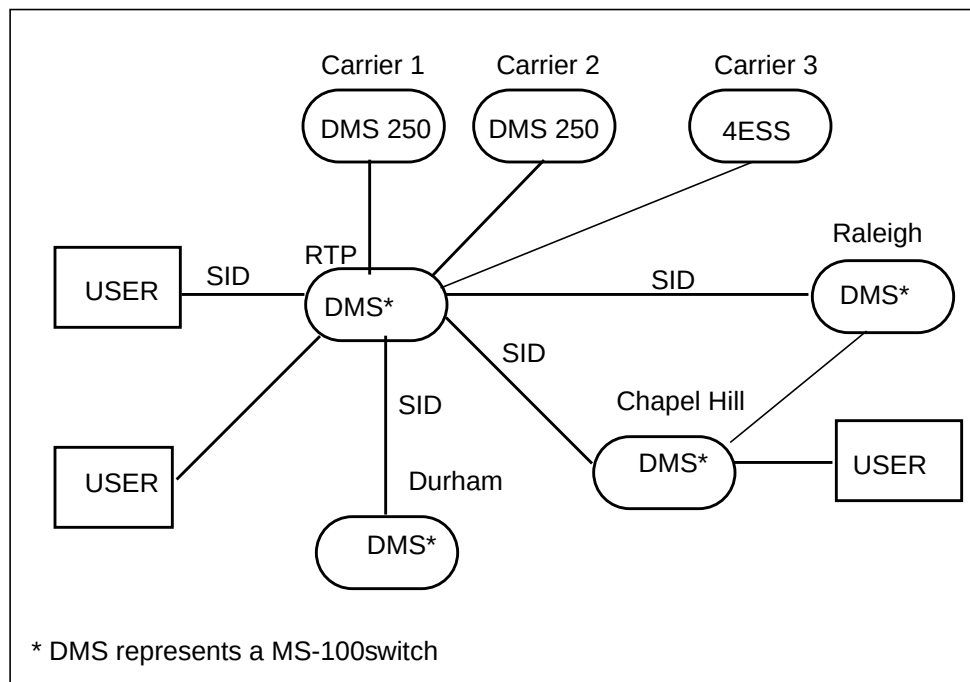
Figure 6-25 Service Identifier Routing on an FX
