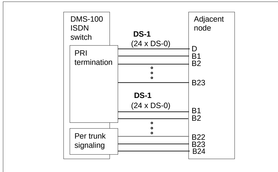
Figure 2-2 PRI channels
