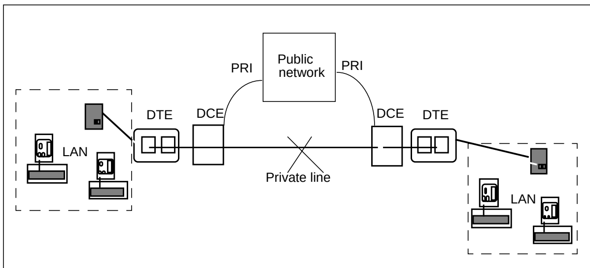
Figure 1-13 Private line backup/augmentation application
