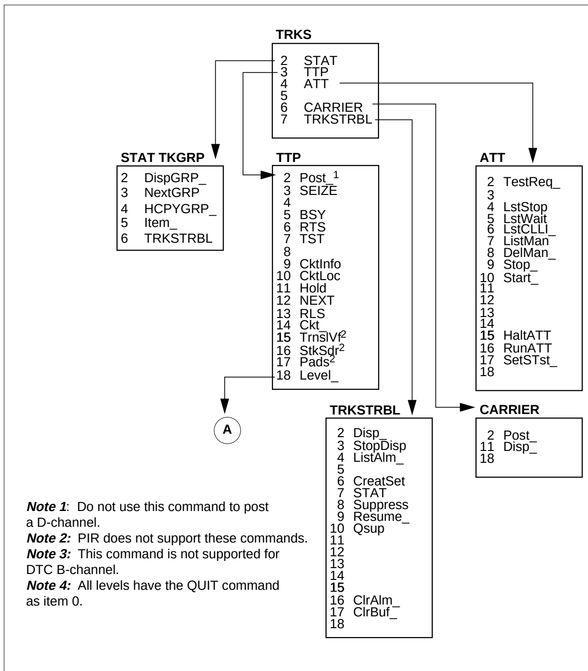
Figure 11-3 TRKS-level commands
