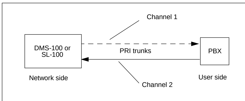
Figure 6-18 RLT overview
