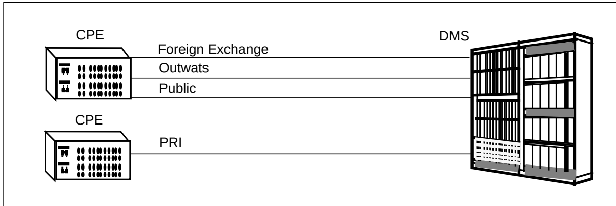
Figure 1-1 PRI integrated services access (ISA/call-by-call)
