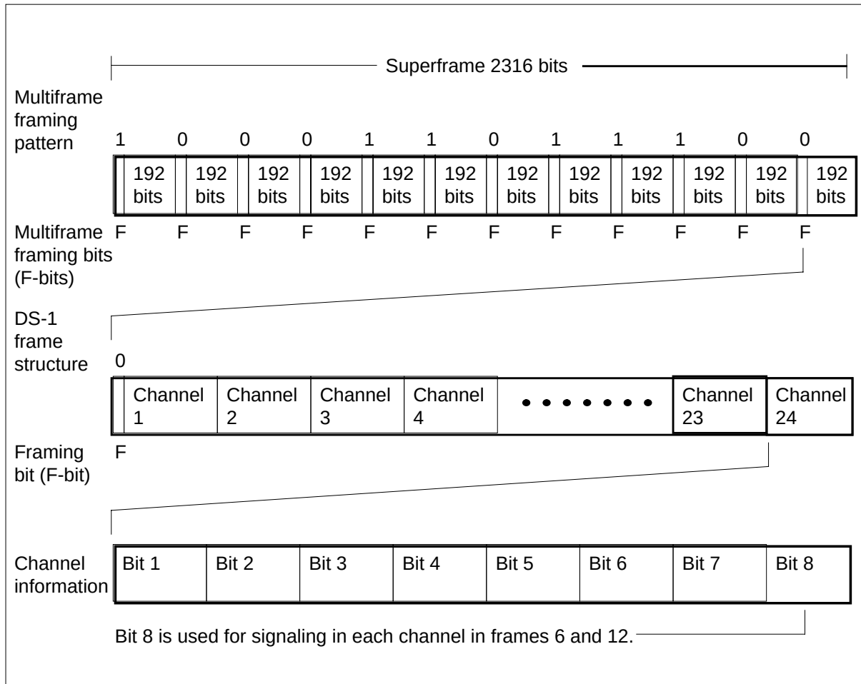
Figure 3-2 DS-1 and Superframe signaling formats
