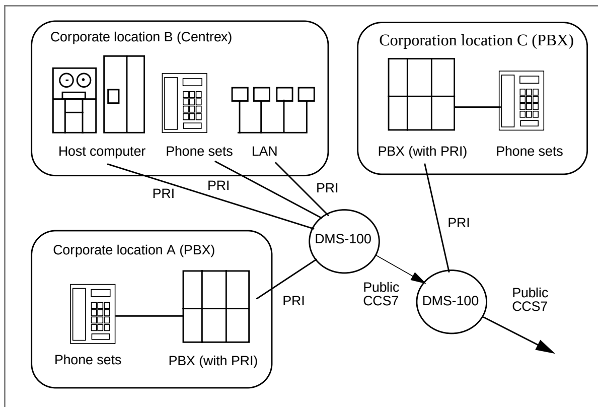
Figure 4-1 A typical PRI network
