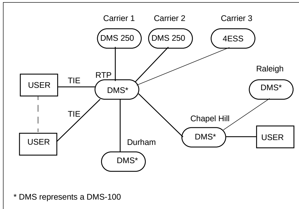
Figure 6-14 Tie line
