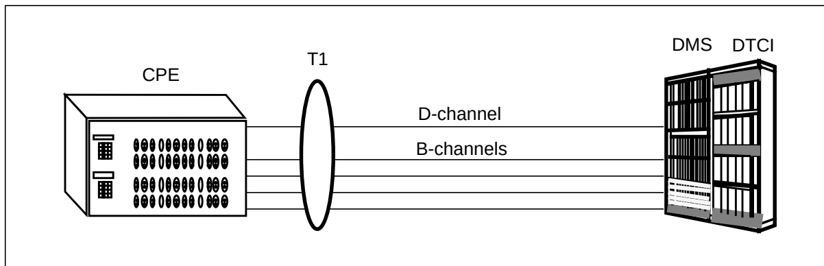
Figure 1-2 PRI out-of-band messaging
