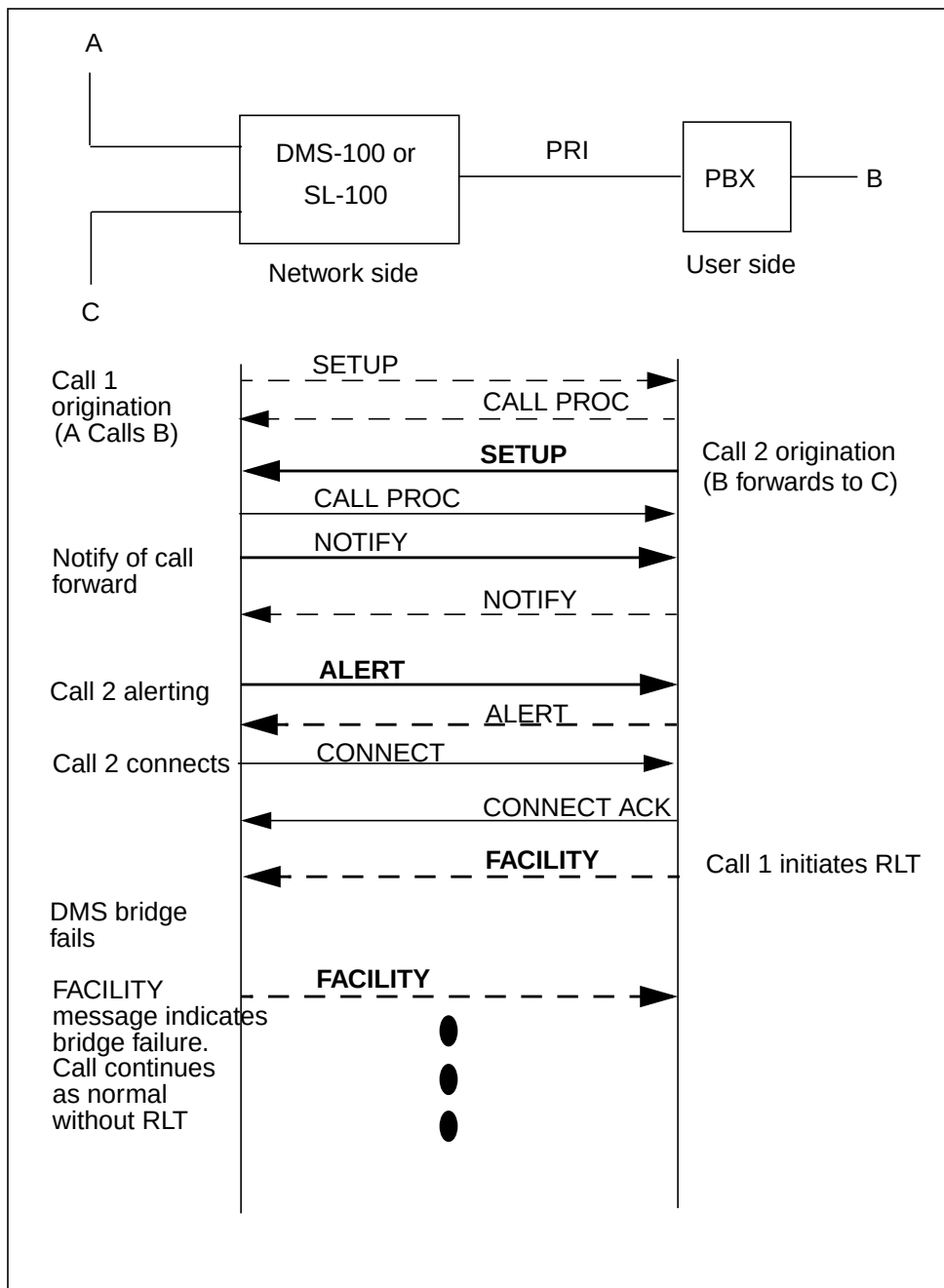
Figure 6-23 RLT scenario with Bridge Failure
