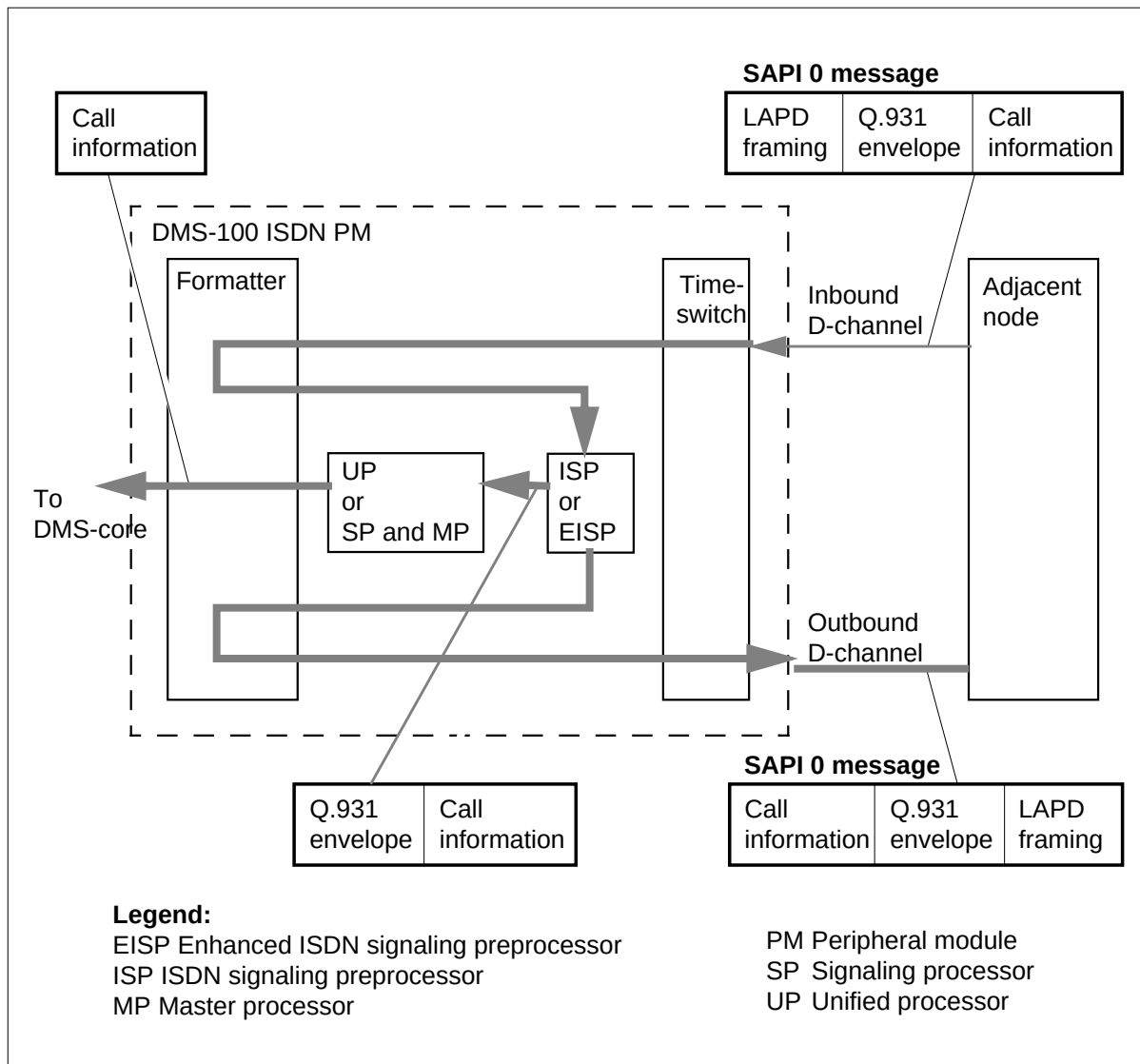
Figure 2-5 PRI D channel processing
