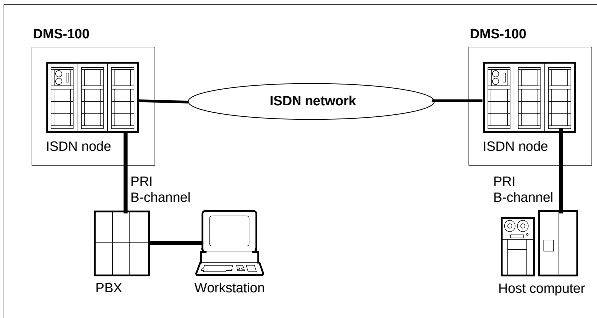
Figure 2-3 B-channel data call example
