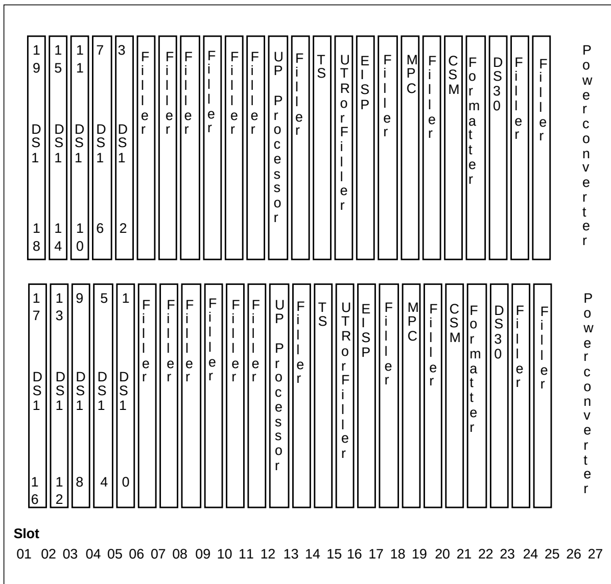
Figure 5-1 XPM-PLUS dual unit node DTCl
