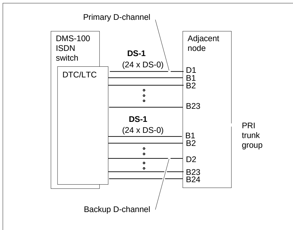
Figure 2-4 PRI consolidated signaling
