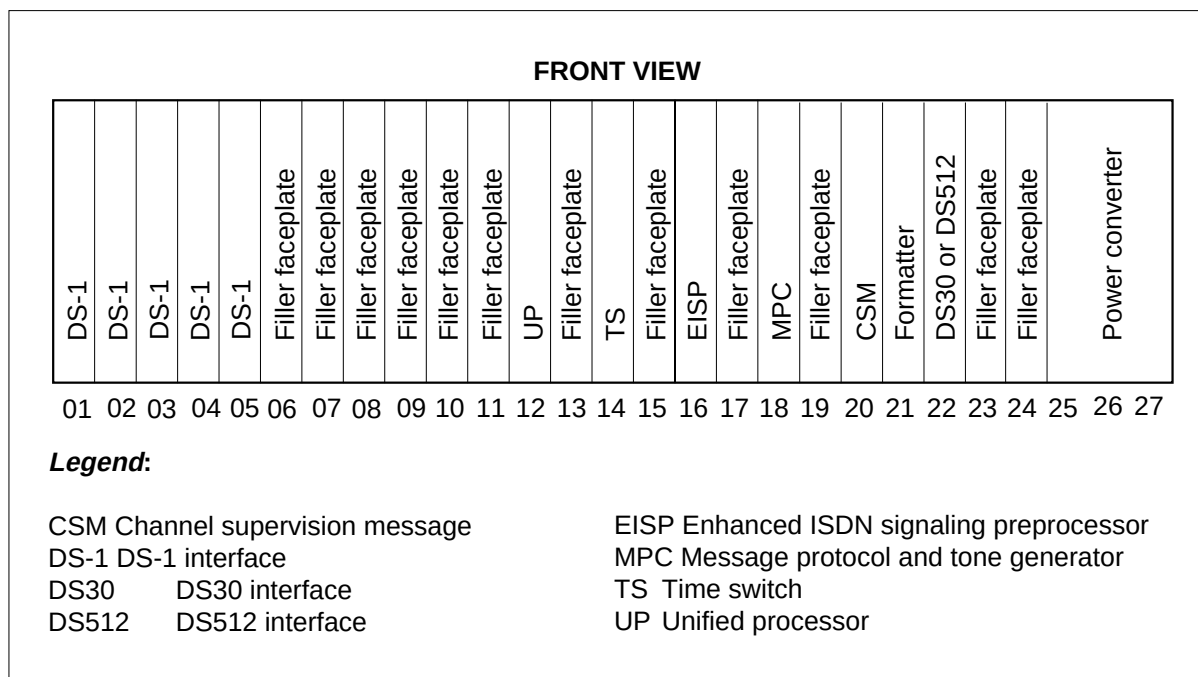
Figure 2-6 DTCI shelf layout for an XPM configuration
