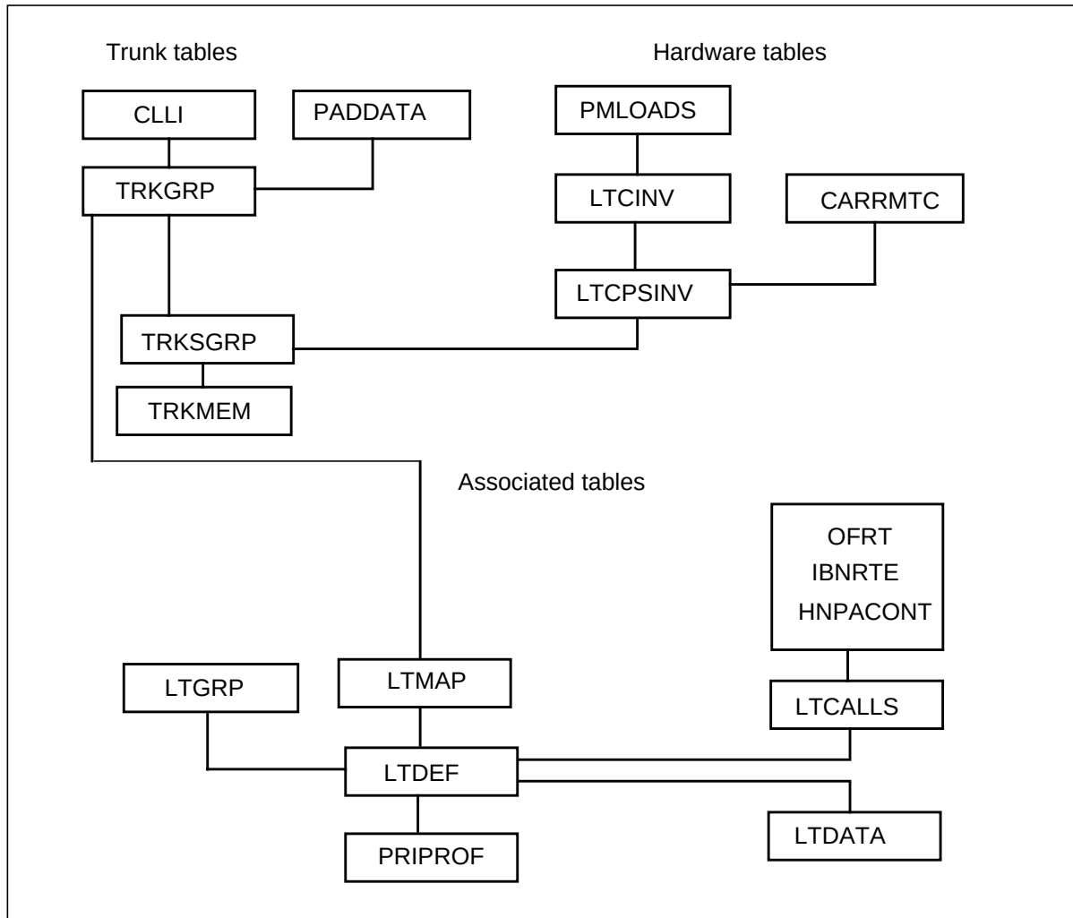
Figure 5-2 PRI datafill table flow
