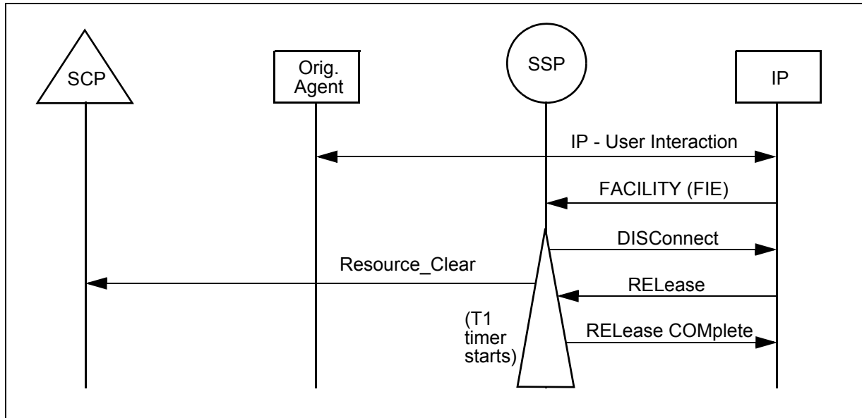
Figure 90 SSP receives Return Error component in FACILITY message
