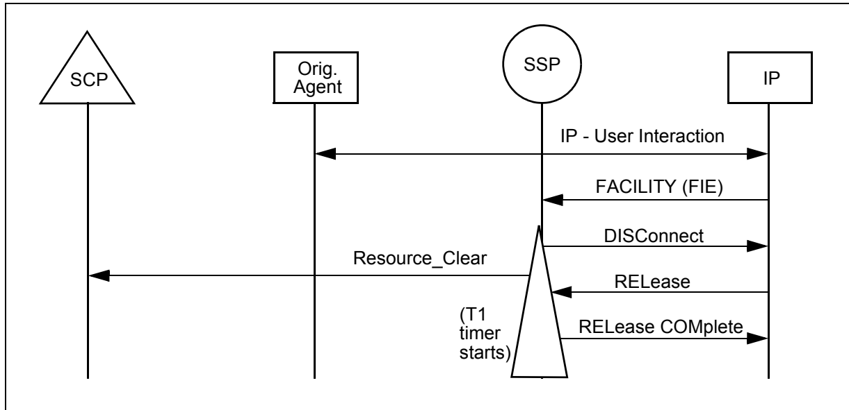
Figure 89 SSP receives Reject component in a FACILITY message from a local IP
