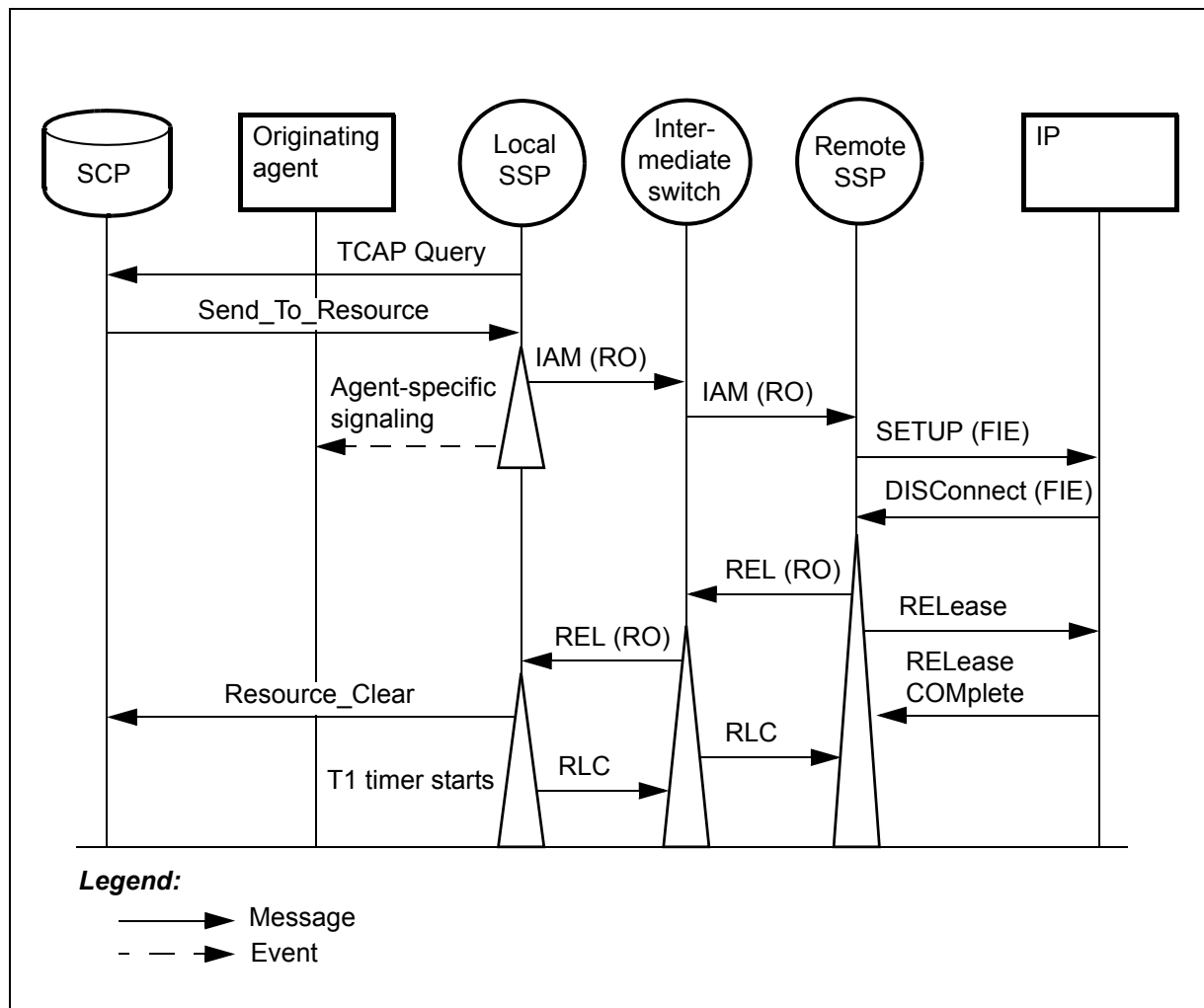
Figure 99 Remote IP cannot execute the requested operation
