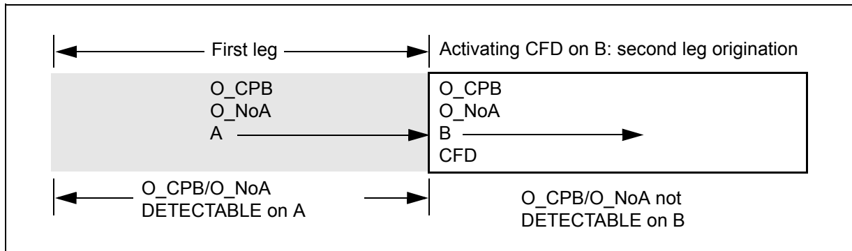
Figure 119 Second leg origination
