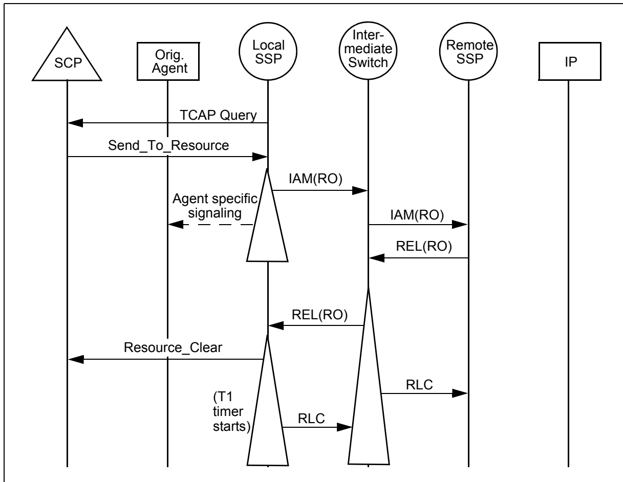
Figure 101 Remote SSP cannot execute the requested operation
