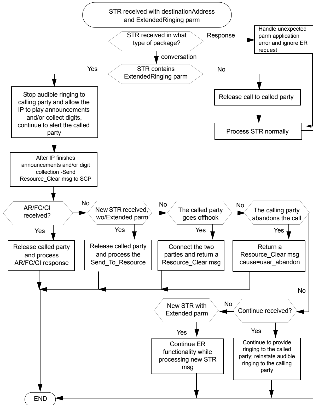
Figure 71 External STR-ER response handling
