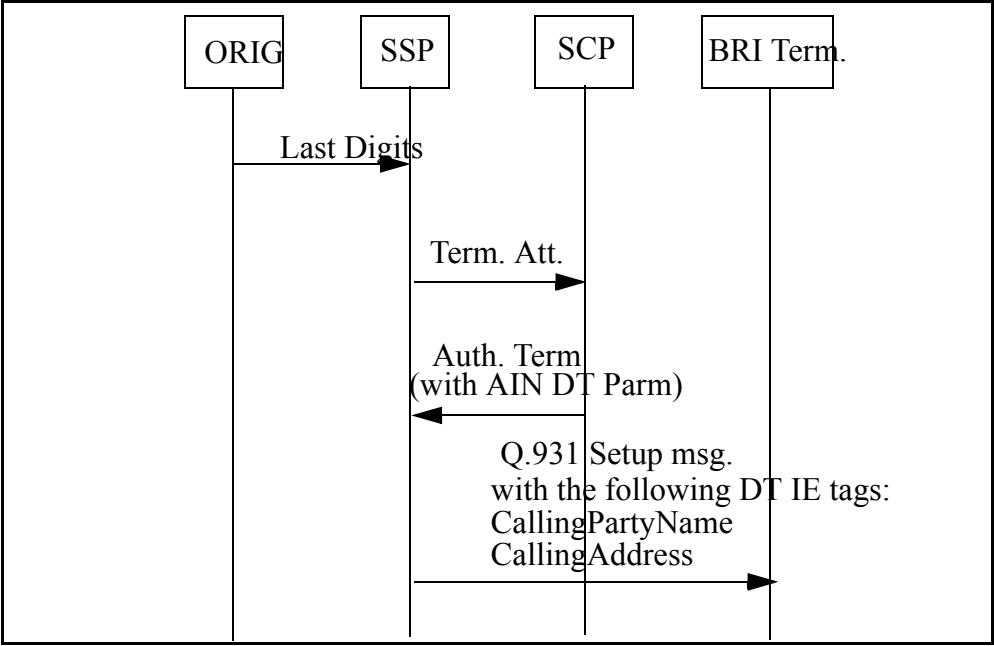
Figure 14 ISDN BRI call termination flow diagram with Display Text delivered in Q.931 Setup message
