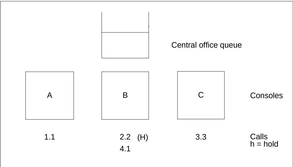
Call status after removing call 4.1
