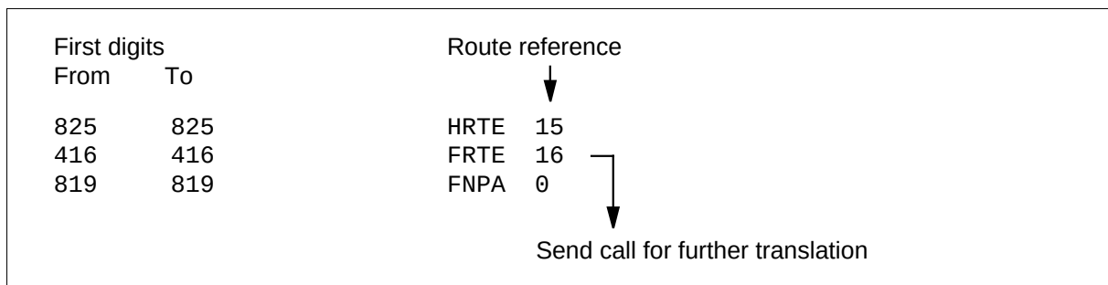
Figure 1-14 Subtable RTEREF
