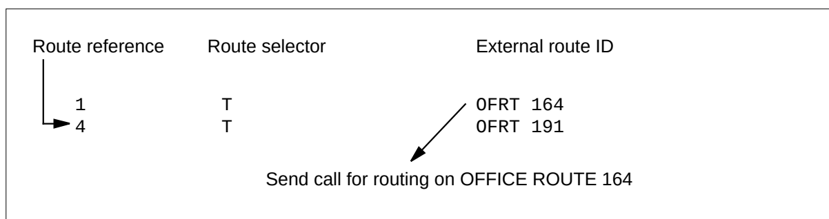
Figure 1-17 Subtable RETEREF
