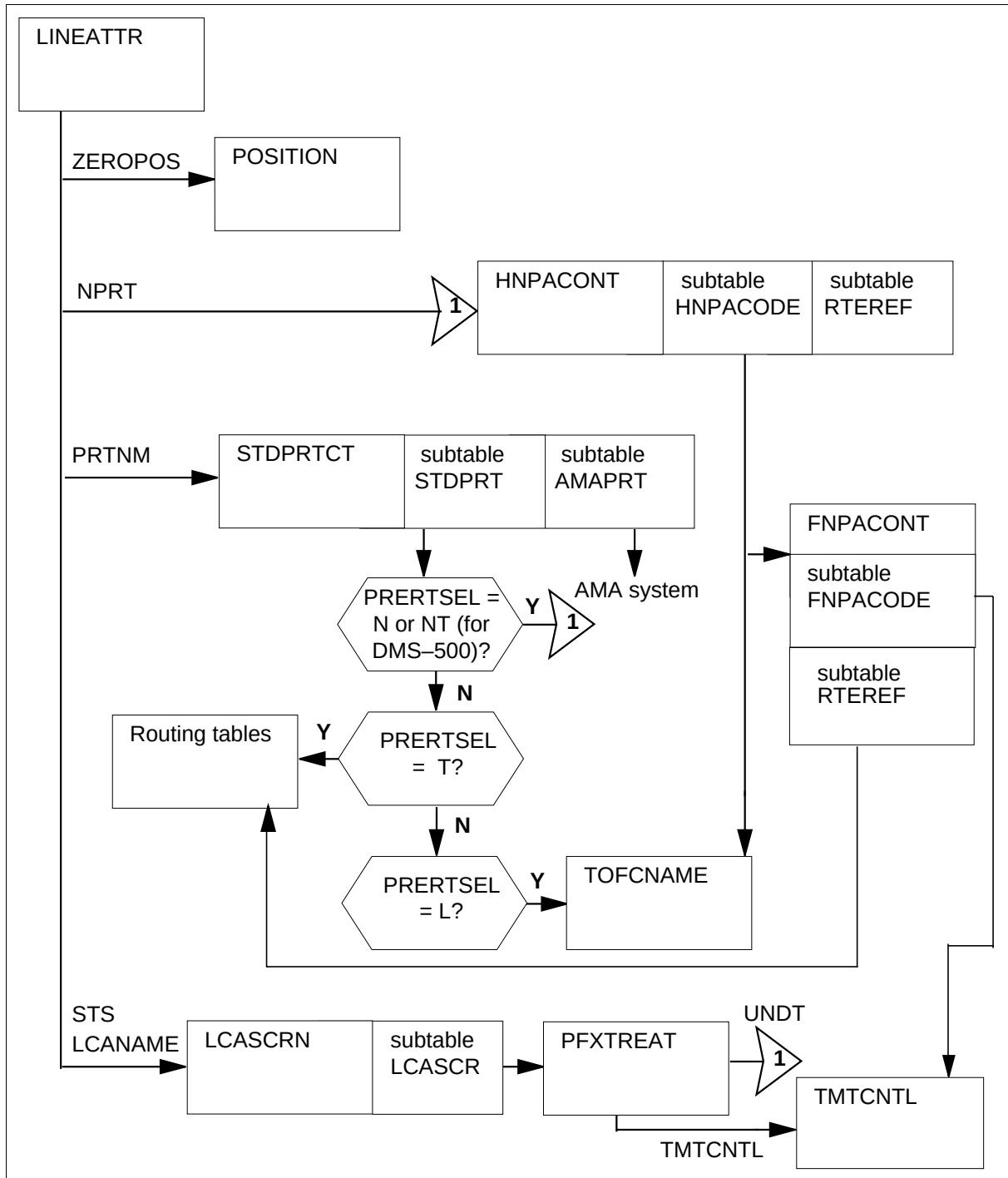
Figure 1-4 Table flow for screening
