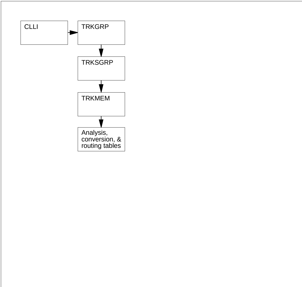
Figure 2-1 Translations table flow for trunk tables
