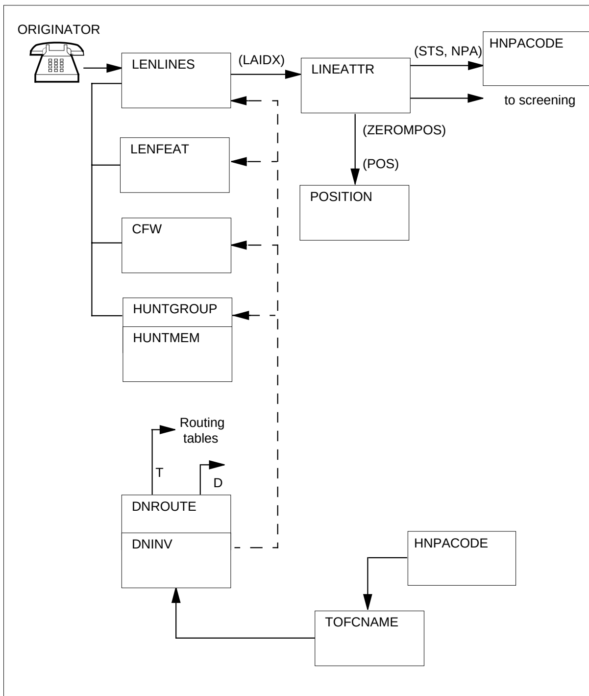
Figure 1-3 Table flow for lines
