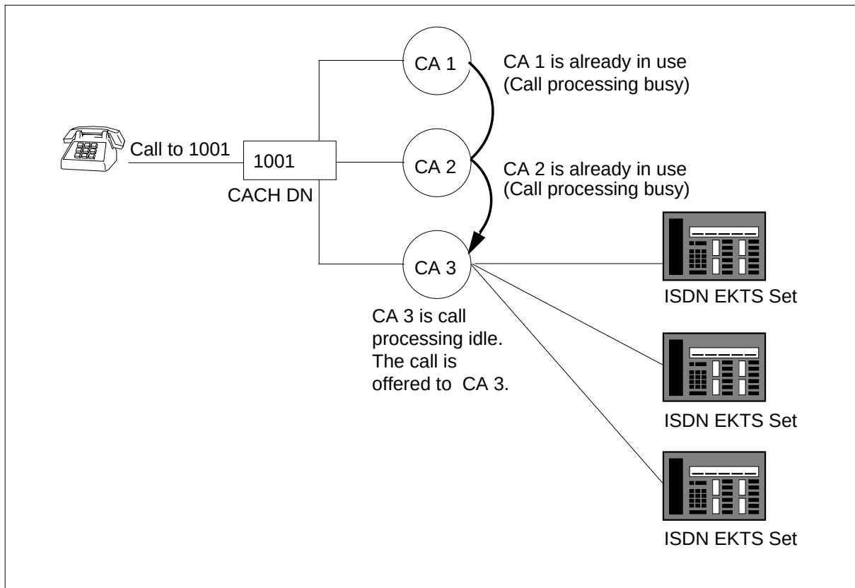
Example of a terminating CACH call-CA1 and CA 2 are call processing busy
